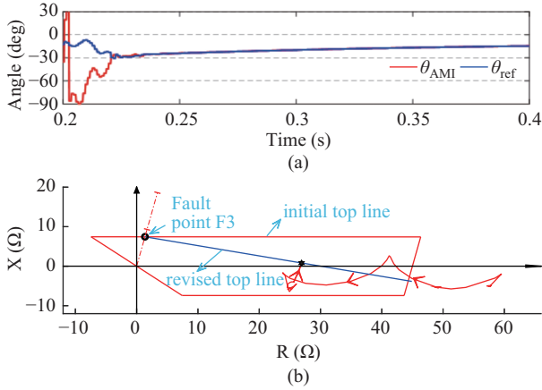
Fig. 9. Fault BC at point F3 ( R_f = 10 \Omega ). (a) Dynamic angles \theta_{AMI} and \theta_{ref} . (b) Trajectory of Z_{app}^{BC} .
