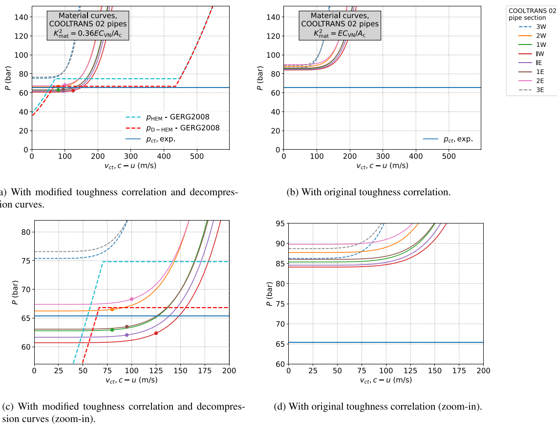
Fig. 9. Two-curve plots for COOLTRANS Test 2 with and without updated toughness correlation. For the dashed material curves, arrest was observed experimentally. Fluid decompression curves for HEM and D-HEM are included in addition to the crack-tip pressure inferred from the experiment (Michal et al., 2020).
