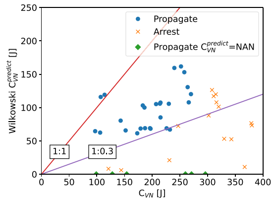
(b) Actual and predicted C_{VN} with Wilkowski correction.
