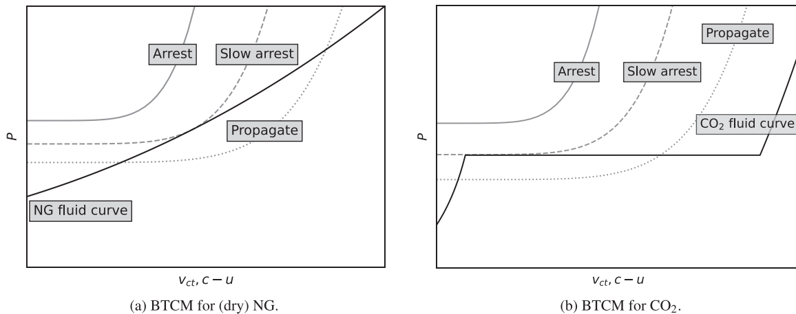
Fig. 1. Illustration of the Battelle two-curve method (BTCM) for \text{CO}_2 and (dry) natural gas (NG) showing an example fluid curve and material curves that would result in propagating and arresting fractures, as well as the limiting case of slow arrest.
