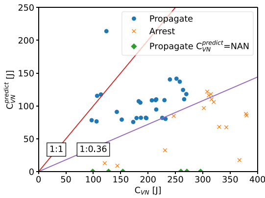
(a) Actual and predicted C_{VN}
