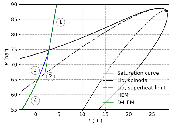
(b) The steps in the D-HEM calculation (zoom-in).
