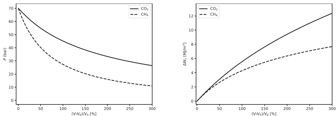
(a) Pressure along isentropes vs relative volume change.
