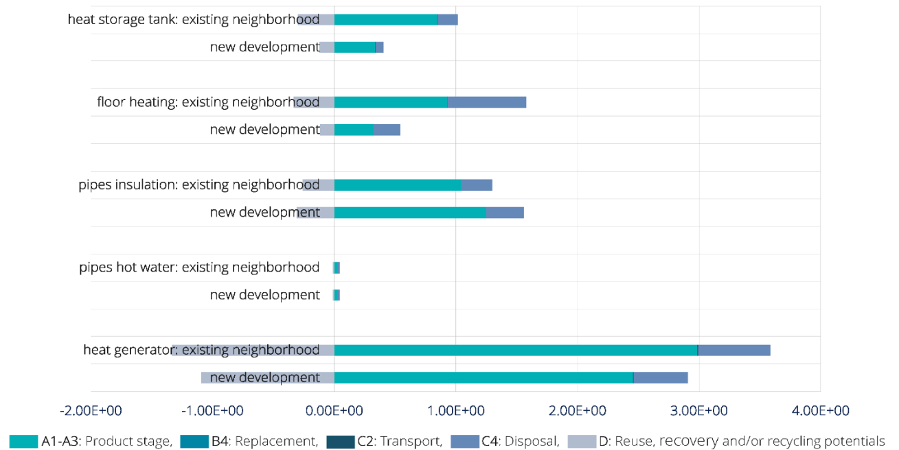
Figure 21. Comparison GWP for two cases by different TBS [kg CO 2 -eq.]
