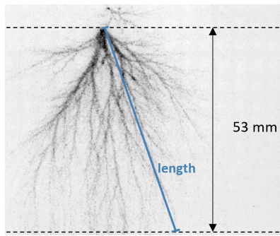
Fig. 3 – The streamer length was measured by drawing a straight line from the needle-tip (streamer starting-point) to the end of the longest branch, as illustrated with the blue line. The height of the needle-tip and the position of the flat electrode are marked with dashed lines. Some shorter streamers are emerging from the rod-electrode above the needle.
