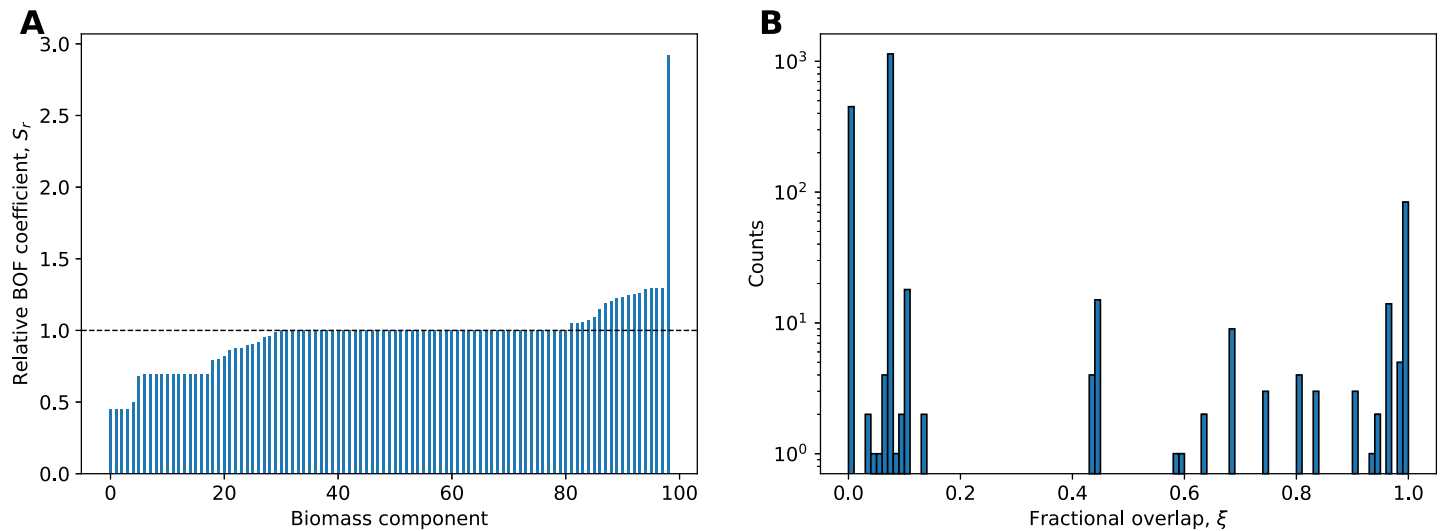
Fig 2. Adjustments of BOF stoichiometries impact attainable flux ranges. (A) Rank-ordered, relative value of BOF coefficients, S_r (Eq 2), of eBOF compared to mBOF. (B) Histogram of fractional overlap of attainable flux ranges, \xi (Eq 1), for all model reactions using mBOF versus eBOF.
