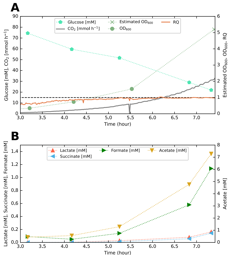
Fig 1. Time-course fermentation profile. Fermentation profile of E. coli K-12 MG1655 growing in a minimal glucose medium before sampling of biomass at \sim 7.5 h. (A) Glucose concentration [mM], CO 2 in the off-gas [mmol h -1 ], respiratory quotient (RQ) [unitless], and OD 600 [unitless]. Unity is highlighted on the same axis as the RQ for reference. The final OD 600 was estimated from the measured cell concentration of 2.6 \text{ gCDW L}^{-1} at sampling, assuming a cell dry weight to OD 600 conversion factor of 0.5 [15, 48]. (B) Concentrations [mM] of the fermentation products lactate, formate, acetate, and succinate. The same figure, except plotted from t = 0 , can be seen in S4 Fig .
