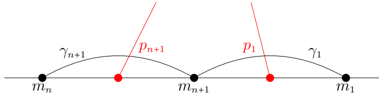
FIGURE 15. The notation used in the proof of Theorem 4.11
