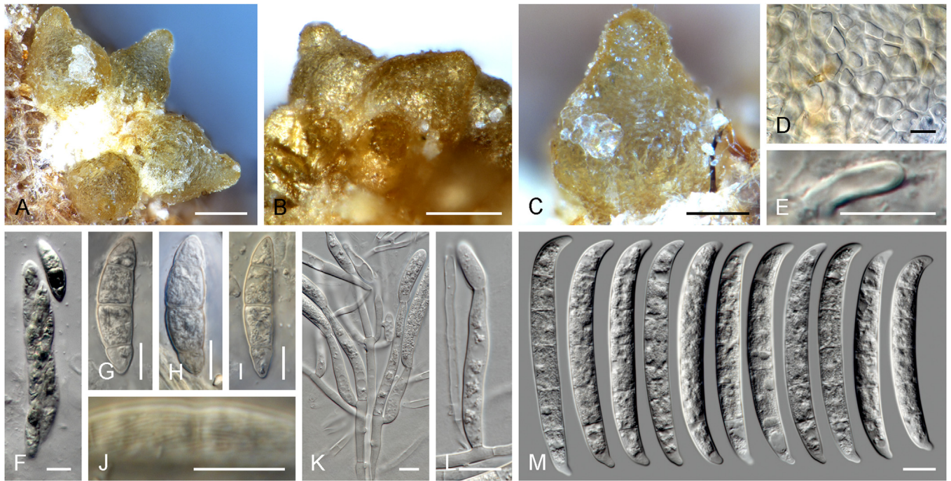
Fig. 30. Luteonectria albida . A–C. Ascomata on natural substrate. D. Surface view of perithecial wall in lactic acid. E. Detail of ascum hair. F. Asci. G–J. Ascospores (J. Surface view). K, L. Conidiophores and conidiogenous cells. M. Macroconidia. A, C. BPI 550103. B. BPI 1108874. D–J. BPI 1108875. K–M. CBS 102683. Scale bars: A, B = 100 \mu m; C = 50 \mu m; all others = 10 \mu m.
