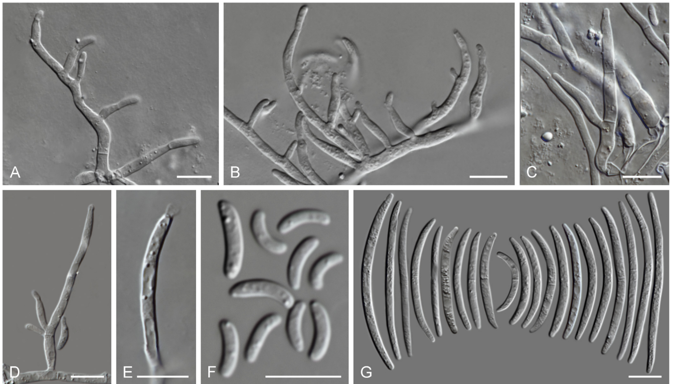
Fig. 47. Stylonectria comiculata (CBS 125491). A–E. Conidiophores and conidiogenous cells. F. Microconidia. G. Macroconidia. Scale bars = 10 \mu m.
