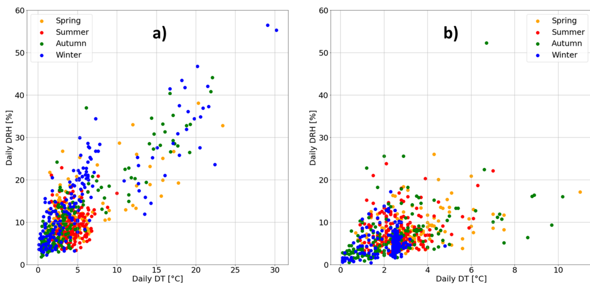
Figure 4. Scatter map of daily range of RH vs. daily range of T for Ringebu church (a) and Heddal church (b). The different colours stand for the different seasons of the calendar year, according to the legend.
