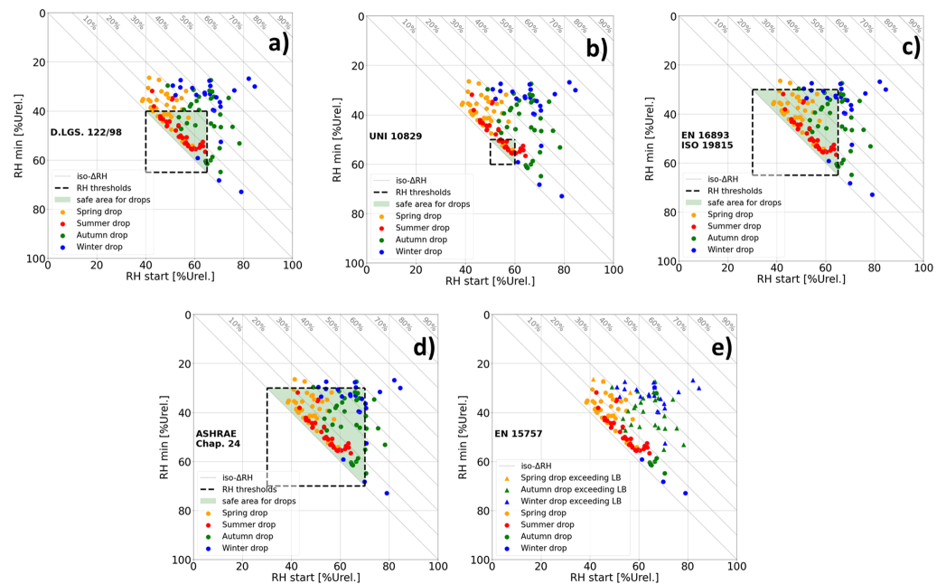
Figure 6. Scatterplots of the drops of RH identified in Ringebu church through the MoD strategy as originally explained in [20], together with the thresholds defined by the standards: D. Lgs. 122 art. 150 par. 6 (a), UNI 10829 (b), EN 16893 and ISO 19815 (c), ASHRAE Chap. 24 (d), EN 15757 (e).
