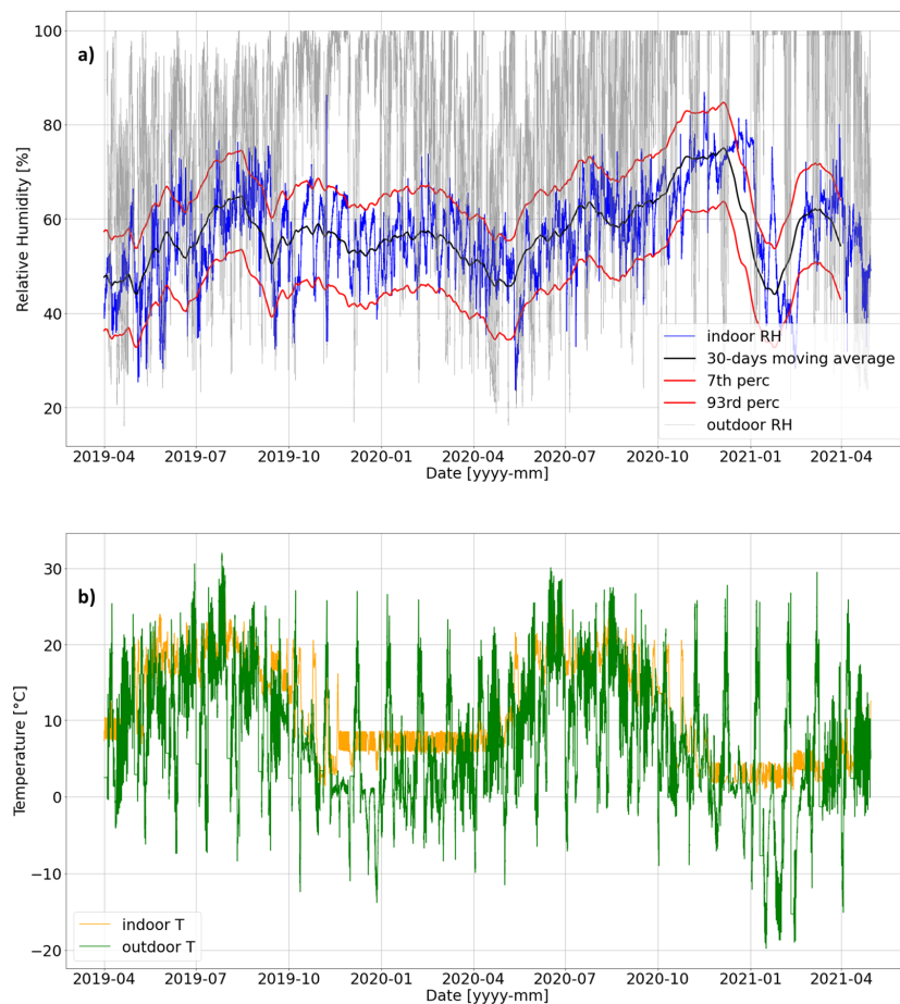
Figure A2. Microclimatic timeseries collected inside and outside Heddal church from the end of March 2019 to the end of April 2021: (a) outdoor RH (grey), indoor RH (blue), moving average of RH (black) and percentiles (red) of RH fluctuations computed according to [4]; (b) outdoor T (green) and indoor T (orange).
