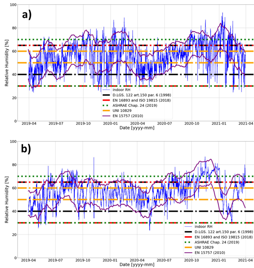
Figure 5. Indoor RH timeseries in Ringebu (a) and Heddal (b) church, together with the thresholds defined by the standards: D. Lgs. 122 art. 150 par. 6 (black dashed line), UNI 10829 (orange dashed lines), EN 16893 and ISO 19815 (red dashed lines), ASHRAE Chap. 24 (green dotted lines), EN 15757 (purple curves).
