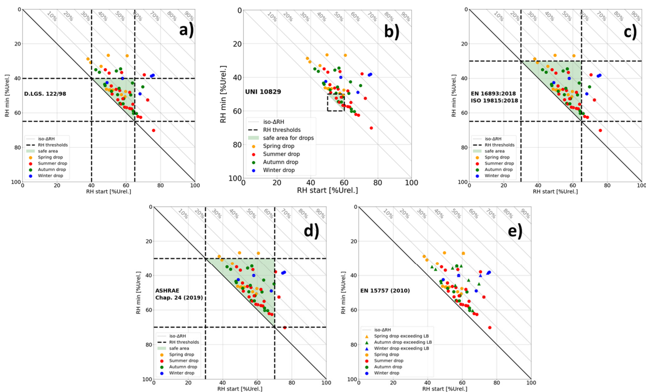
Figure 7. Scatterplots of the drops of RH identified in Heddal church through the MoD strategy as originally explained in [20], together with the thresholds defined by the standards: D. Lgs. 122 art. 150 par. 6 (a), UNI 10829 (b), EN 16893 and ISO 19815 (c), ASHRAE Chap. 24 (d), EN 15757 (e).
