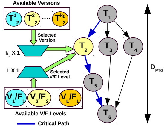
Fig. 2: Task graph
