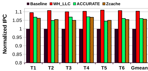
Fig. 15: Change in performance (IPC) by applying WH_LLC at the LLC along with Way-shutdown and Zcache.
