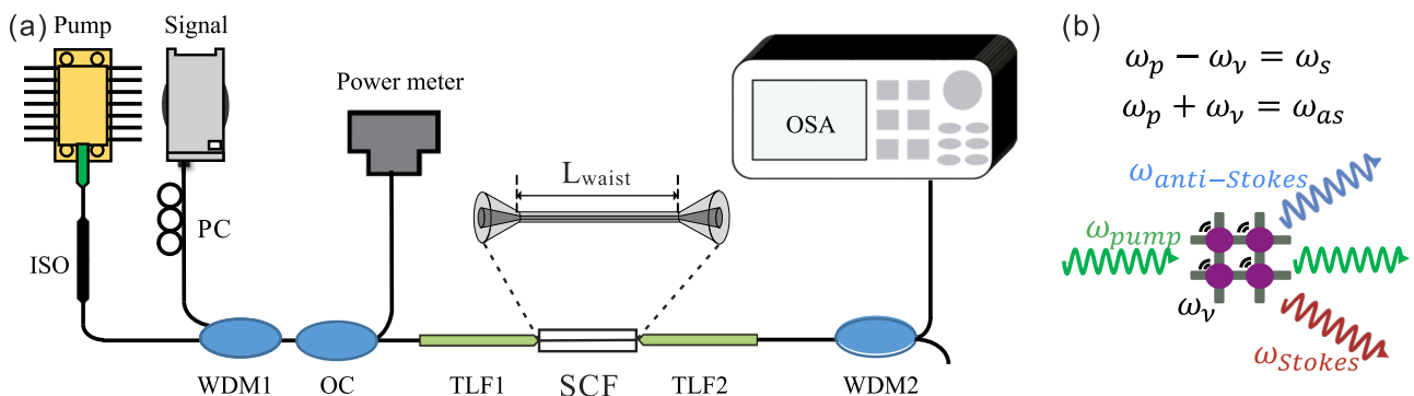
FIG. 1. (a) Schematic of the experimental setup to measure the Raman response of the tapered SCFs. ISO: isolator, PC: polarization controller, WDM: wavelength division multiplexer, OC: optical coupler, TLF: tapered lensed fiber, and OSA: optical spectrum analyzer. The inset shows the geometry for the tapered SCF. (b) Schematic of Raman scattering and energy conservation equations.
