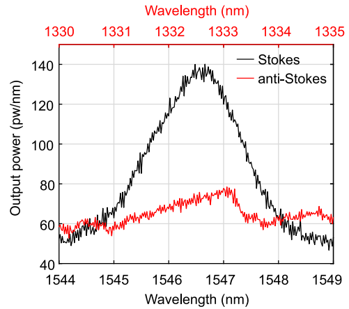
FIG. 4. Comparison of Stokes (bottom wavelength axis) and anti-Stokes (top axis) Raman emission for a pump wavelength of 1431 nm and a coupled power of ~50 mW.
