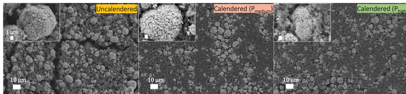
Fig. 7 SEM surface analysis of lignin/water cathode coatings with similar mass loading ( 7.4 \pm 0.3 \text{ mg/cm}^2 ) which was uncalendered, calendered at medium pressure using a 60 \mu\text{m} calendering gap ( P_{\text{medium}} ), or calendered at high pressure using a 45 \mu\text{m} calendering gap ( P_{\text{high}} ) (Magnitude: 1000 \times ). The NMC111 particles are shown in the top right corner (Magnitude: 10000 \times ). The rate capability of these cathodes is shown in Figure 10b.
