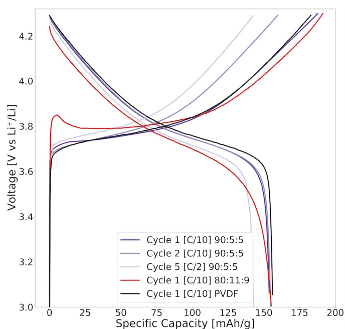
Fig. 13 The voltage profile of the first and second cycle at C/10 and the fifth cycle at C/2 for NMC111 cathodes fabricated using 80:11:9 (red) or 90:5:5 (purple) lignin/water (7.4 mg/cm 2 ), and 85:10:5 PVDF/NMP-fabricated cathodes (black) (6.9 mg/cm 2 ). The cathodes were cycled in coin cells between 3.0 - 4.3 V (vs Li + /Li) at different [C-rates] at 22°C using a Li metal anode. 1C = 160 mA/g.
