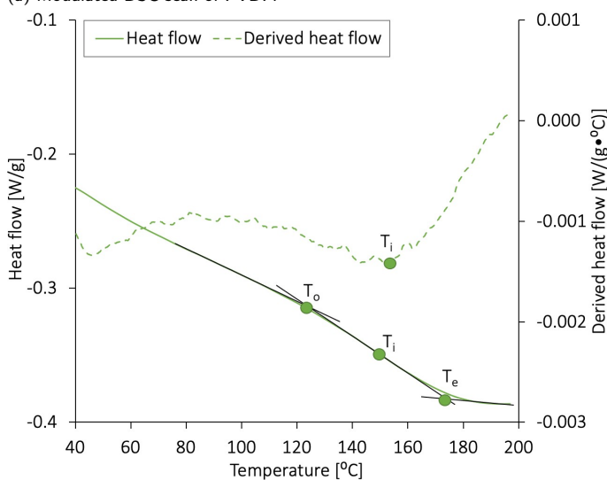
(b) DSC scan of lignin.
