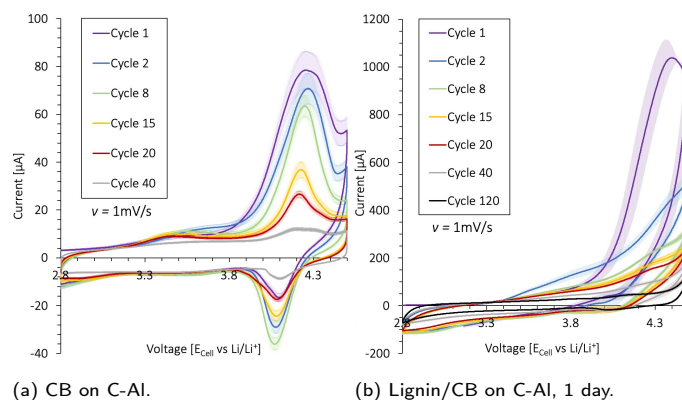
Fig. 4 The electrochemical activity of the a) carbon black (CB) coated on C-Al, and lignin/CB (50/50 wt %) coated on C-Al scanned after 1 day wetting. The coin cells were scanned between 2.8 - 4.5 V (vs Li/Li + ) using a Li-metal anode, LiPF 6 in ED/DMC/DEC electrolyte, and a scan rate of v = 1 mV/s at 22 °C.
