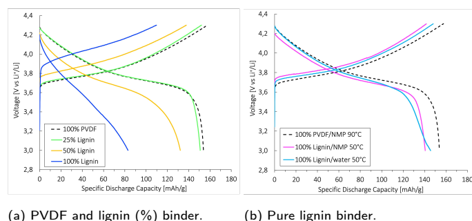
Fig. 8 Specific discharge capacity during the third formation cycle at C/10 (1 C = 160 mA/g). The cathodes were coated onto Al-foil with a mass loading of 4.4-4.8 mg/cm 2 , and calendered at P medium . A PVDF/NMP-based cathode dried at 90 °C (black) was used as a baseline. The cathodes were cycled between 3.0 - 4.3 V (vs Li + /Li) against a Li-metal anode in a coin cell at 22 °C.
