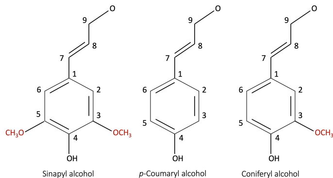
Fig. 1 The monomer species building up a lignin molecule: (a) p-coumaryl alcohol (4-hydroxyl phenyl, H), (b) coniferyl alcohol (guaiacyl, G), (c) sinapyl alcohol (syringyl, S) 19,26
