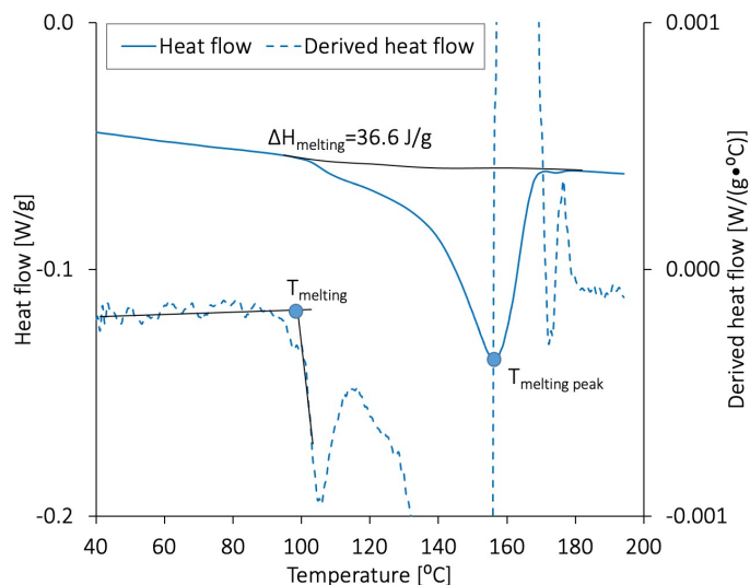
(a) Modulated DSC scan of PVDF.
