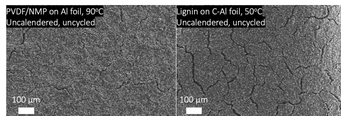
Fig. 6 SEM surface crack analysis of an uncalendered PVDF/NMP-based cathode dried at 90 °C (left) and a lignin/water-based (right) cathode dried at 50 °C with similar mass loading ( 7.4 \text{ mg/cm}^2 \pm 0.2 ).
