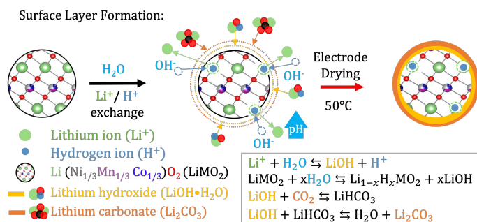
Fig. 2 When the NMC material is exposed to water \text{Li}^+ starts leaching out from its structure while \text{H}^+ from the water intercalates the structure 44 . \text{OH}^- in the solution steadily increases the pH and combines with \text{Li}^+ to form \text{LiOH} as the water evaporates during electrode drying. Further, \text{LiOH} reacts with \text{CO}_2 to form \text{LiHCO}_3 and eventually \text{Li}_2\text{CO}_3 .
