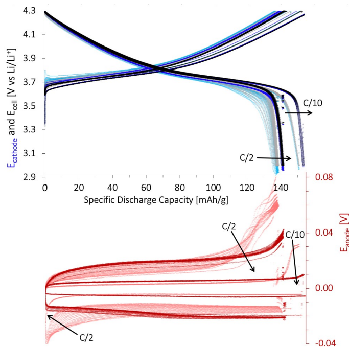
Fig. 11 The galvanostatic cycling performance of a PAT cell using Li metal as anode and reference electrode. The response from the Li-metal anode (red E_{\text{anode}} ), NMC111 working cathode (blue E_{\text{cathode}} ), and both (black E_{\text{cell}} ) were measured. The lignin/water-cathode (80:11:9 wt % NMC111:CB:lignin) was coated on C-Al-foil, with 7.4 \text{ mg/cm}^2 mass loading and calendered at P_{\text{medium}} . The cell was cycled after a 8 days wetting period for 5 cycles at C/10, 21 cycles at C/2 (light colour), 5 cycles at C/10, and 21 cycles at C/2 (dark colour) between 3.0 - 4.3 V vs \text{Li}^+/\text{Li} (1 C = 160 \text{ mA/g} ) at 22^\circ\text{C} . Arrows represent an increasing cycle number. The cathode surface area used for PAT cells was larger ( 2.54 \text{ cm}^2 ) compared to the coin cells ( 1.78 \text{ cm}^2 ) and the separator was glass fiber.
