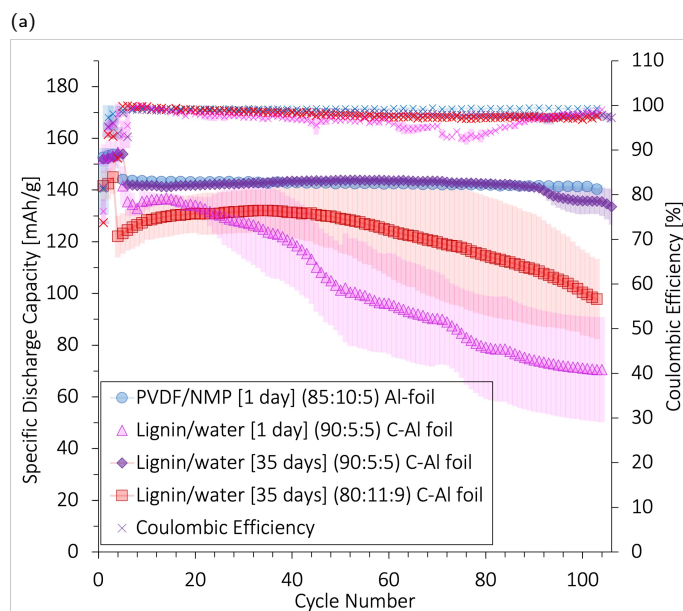
Fig. 12 The average specific discharge capacity (mAh/g) and coulombic efficiency (%) of three coin cells and their standard deviation. The lignin/water cathodes were coated onto a C-Al current collector with 80:11:9 wt % NMC111:CB:binder unless specified. The days refer to The mass loading for all cathodes was 7.4 \pm 0.3 \text{ mg/cm}^2 . An 85:10:5 PVDF/NMP-based cathode with comparable mass loading ( 6.6 \pm 0.6 \text{ mg/cm}^2 ) coated onto a plain Al-foil and wetted for 1 day (blue circles) was used as the baseline. The cathodes were cycled in coin cells between 3.0 - 4.3 V (vs Li + /Li) using a Li-metal anode. The C-rate was C/10 for the first 3 or 5 cycles and C/2 for the following 100 cycles.
