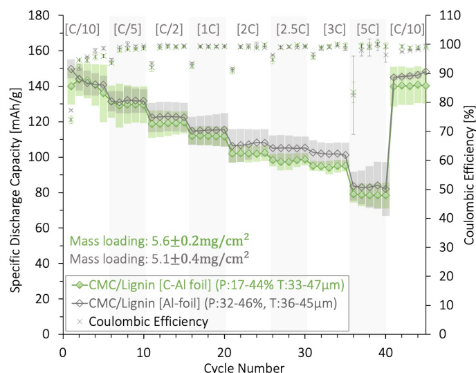
Fig. 9 The average rate capability of three cells with aqueous produced NMC111 cathodes using CMC/lignin (green diamond) coated on plain Al-foil (empty) or carbon coated-Al-foil (C-Al) (filled). T=electrode coating thickness, P=porosity. The cathodes were cycled at different [C-rates] were 1 C = 160 mA/g between 3.0 - 4.3 V (vs Li + /Li) using a coin cell and Li-metal anode at 22 °C. Calendered at P medium .
