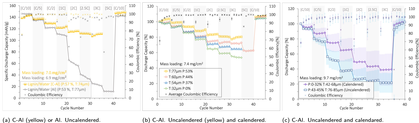
Fig. 10 The rate capability (%) and coulombic efficiency (%) of uncalendered and calendered lignin/water-based NMC111 cathodes with (a), (b) low and (c) high mass loading, resulting in different thicknesses ( T ) and porosities ( P ). An SEM analysis of the cathode surfaces in (b) is presented in Figure 7. The cathodes were cycled at different [C-rates] (1 C = 160 mA/g) in coin cells at 22 °C between 3.0 - 4.3 V (vs \text{Li}^+/\text{Li} ) using a Li-metal anode. The plots with deviation bars show the average and of three cells deviation of three cells.
