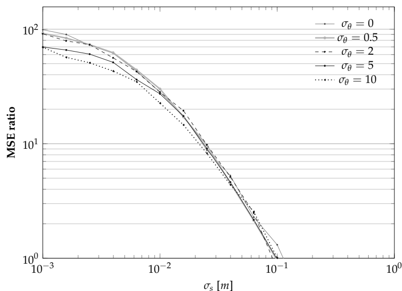
Figure 9. Dependency of the MSE ratio (31) on the standard deviation \sigma_\theta of the sensor-to-landmark angle measurement error in (6), and on the standard deviation \sigma_s of the sensor position evolution uncertainty in (8) for the case L = 2 .
