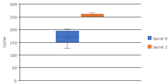
Fig. 4: Speculation Invariant access latency, in cycles, leaking the secret
