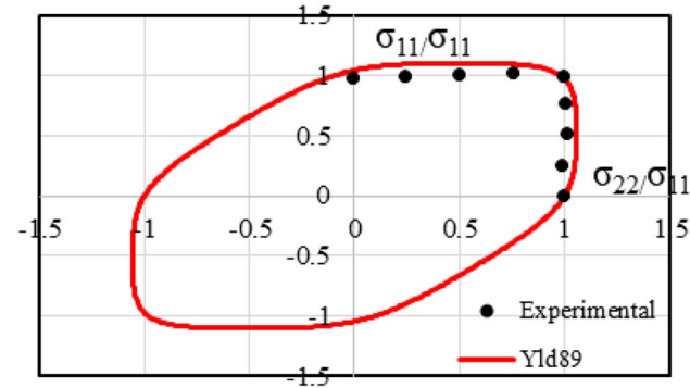
Fig. 55 Yield locus cut of AA 6016-T4 obtained with Yld89
