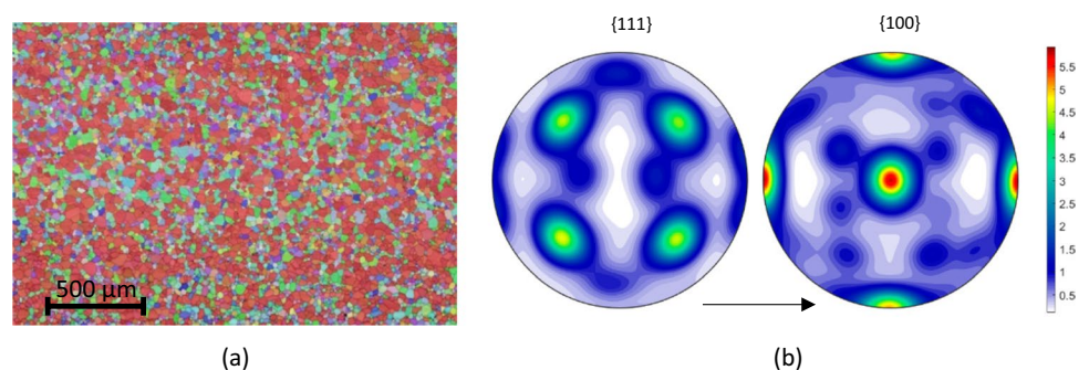
Fig. 1 Initial texture of the 6016-T4 aluminium alloy: a EBSD map; b \{111\} and \{100\} pole figures; the arrow indicates the rolling direction (RD)
