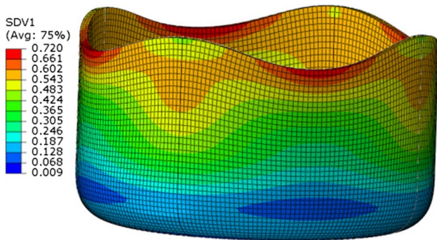
Fig. 110 Predicted isocontours of equivalent plastic strain predicted by Caz2018singlecrys yield criterion with the anisotropy coefficients given in “Caz2018polycrys” Section (Table 15 - ideal cubic texture)
