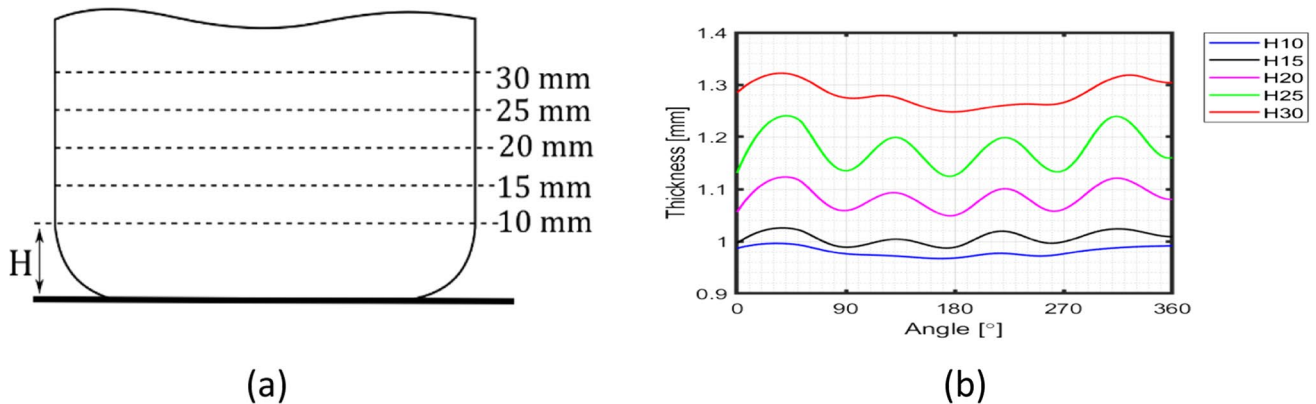
Fig. 23 a Reference heights for the thickness measurements and b Evolution of thickness-angle for different cup heights
