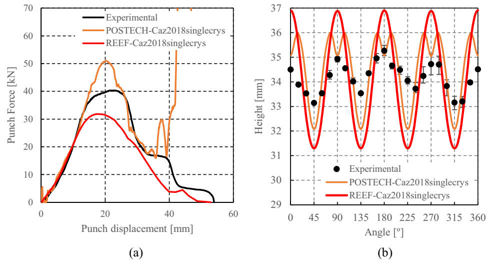
Fig. 109 Comparison between experimental and predicted results by Caz2018singlecrys for the data set of “Caz2018polycrys” Section (Table 15 - REEF) and of “Caz2018singlecrys” Section (Table 20 – POSTECH): a punch force-displacement, b earing profile
