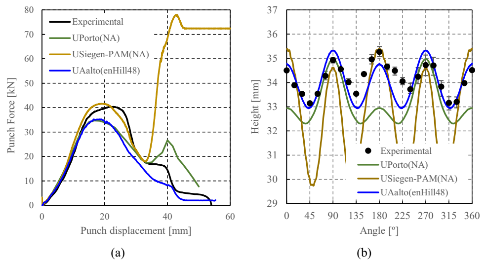
Fig. 78 Comparison between experimental and predicted results by (NA) Hill48 criterion with constant or evolving anisotropy parameters identified in “Hill48 and non-associated flow rule” Section (Eqs. 71): a punch force-displacement, b earing profile
