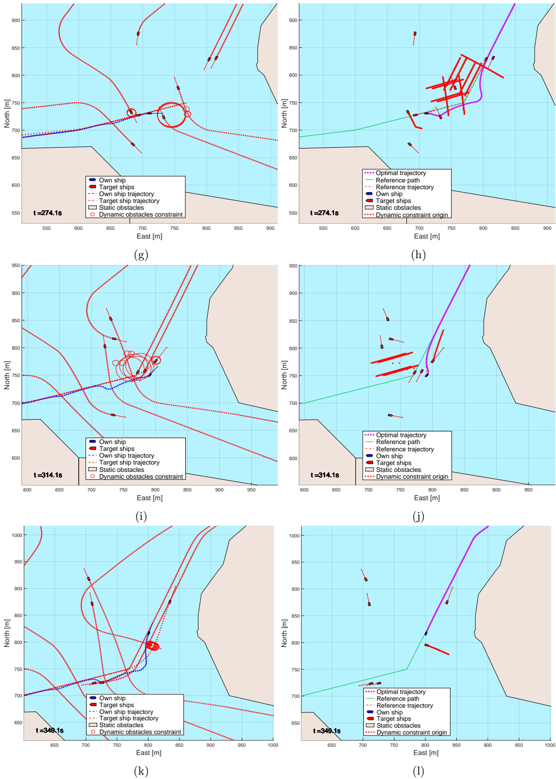
Figure 25: Fjord. Here shown with full prediction. Observe the OS handles the stress test pretty well.
