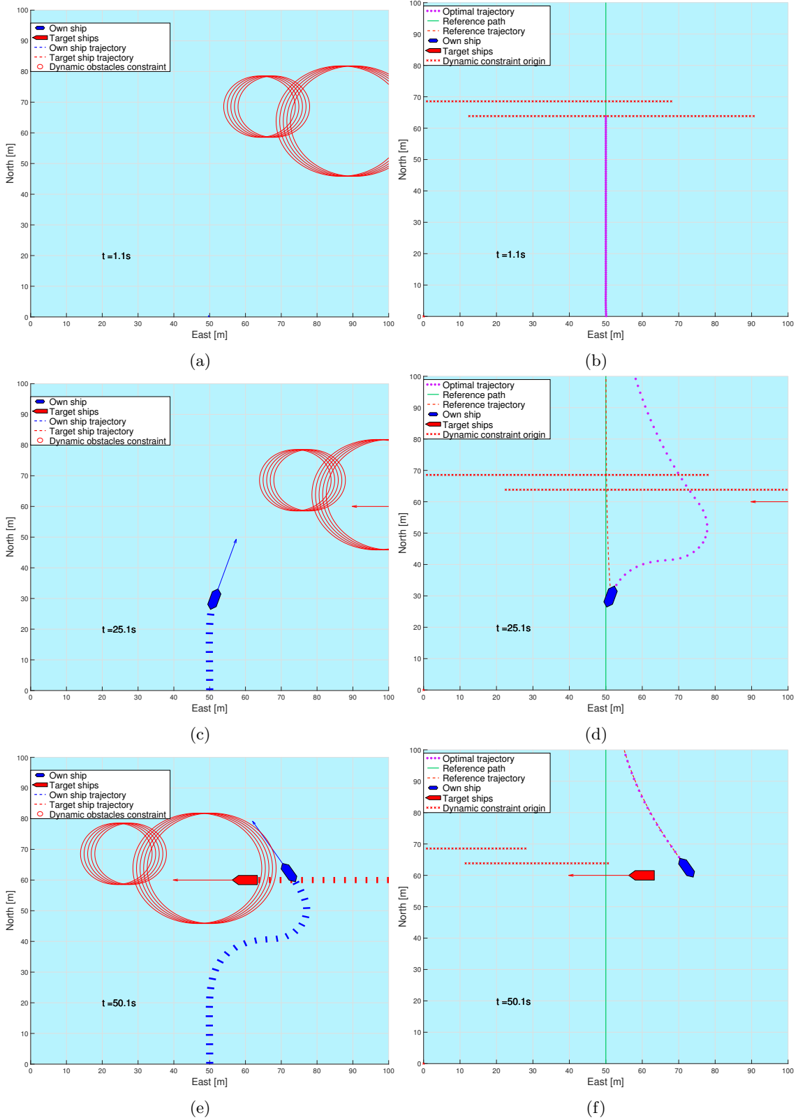
Figure 16: Simple Give-way. Result independent of prediction level.
