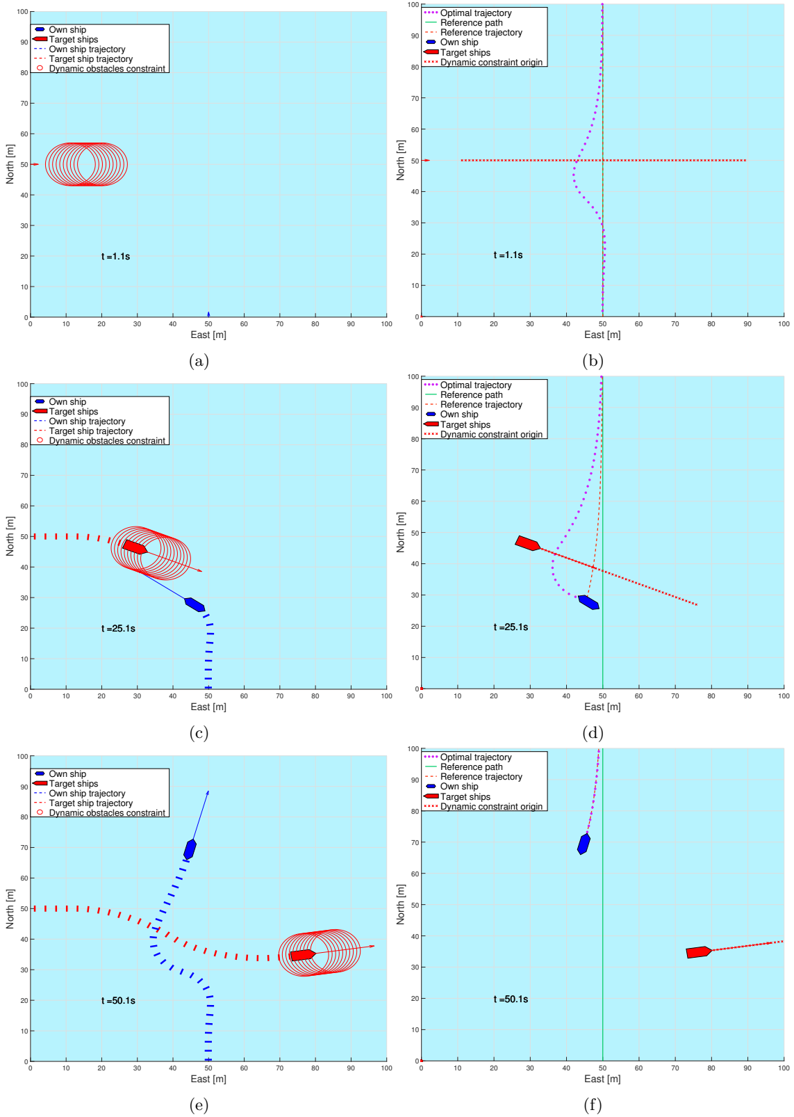
Figure 18: Simple Stand-on. Here shown with simple prediction, the OS can be observed to yield when it shouldn't.
