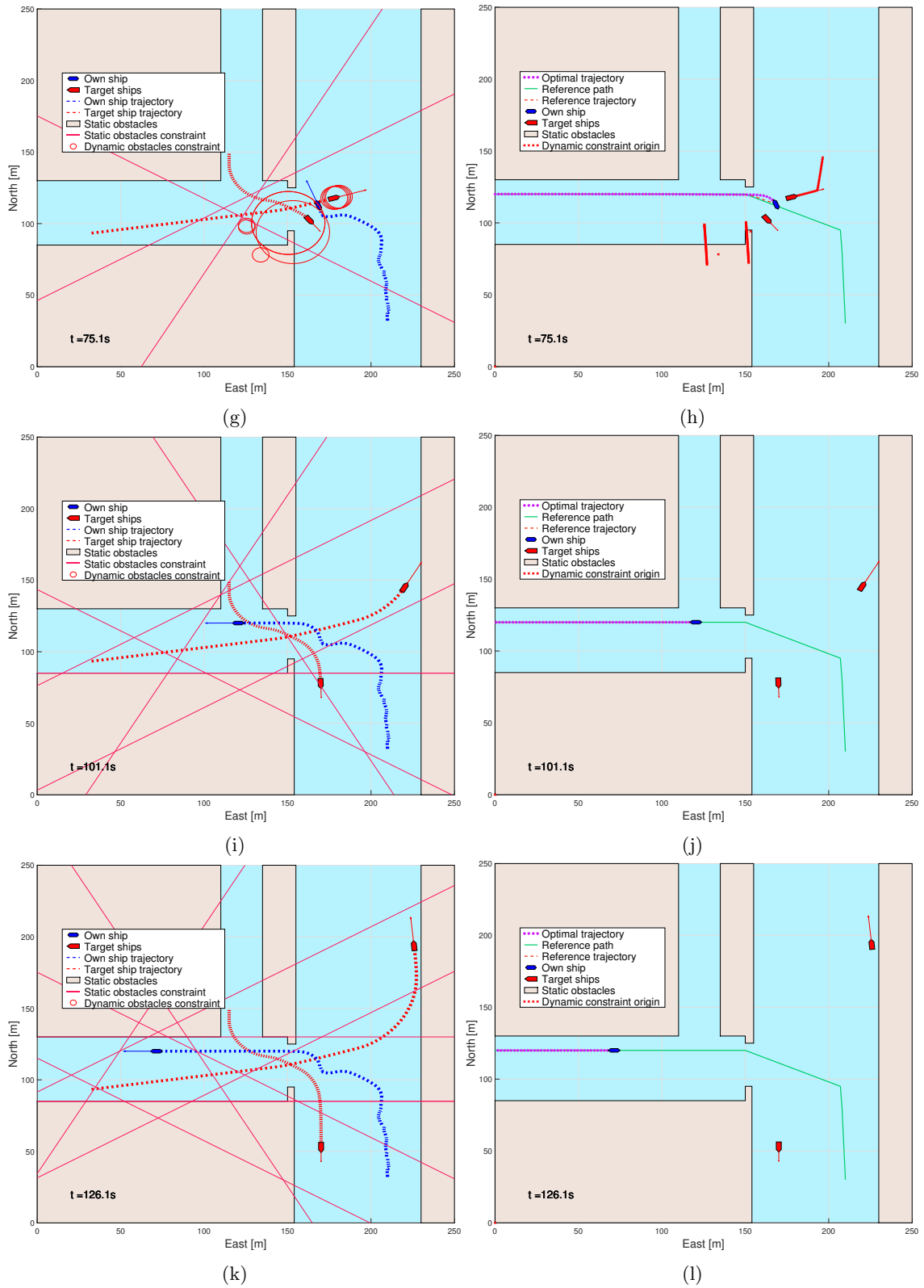
Figure 23: Canals. Here shown with full prediction.
