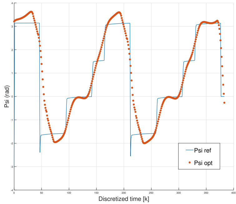
(a) Here we see the heading reference and optimal values, at about k = 50 , and again around 200 we can see that the heading reference experiences a discontinuous jump as it wraps from \pi to -\pi .
