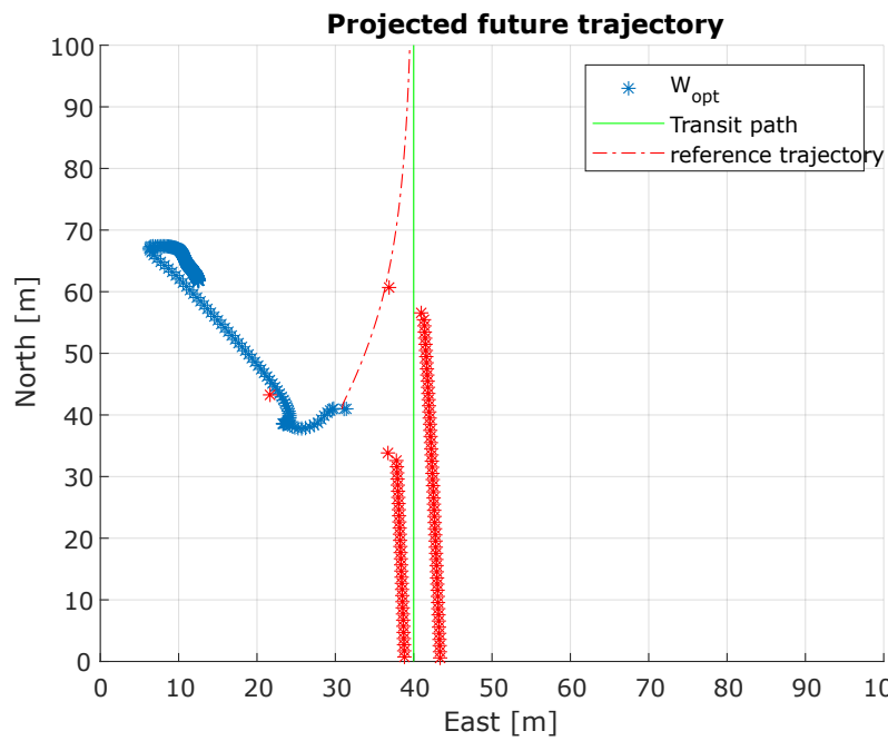
(b) When caught inside an active constraint, the solver is unable to find a feasible solution. Old style figure.
