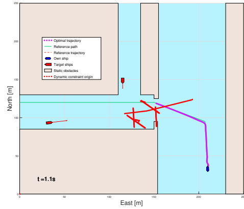
(f) Speed is reduced, resulting in a shorter optimal trajectory.
