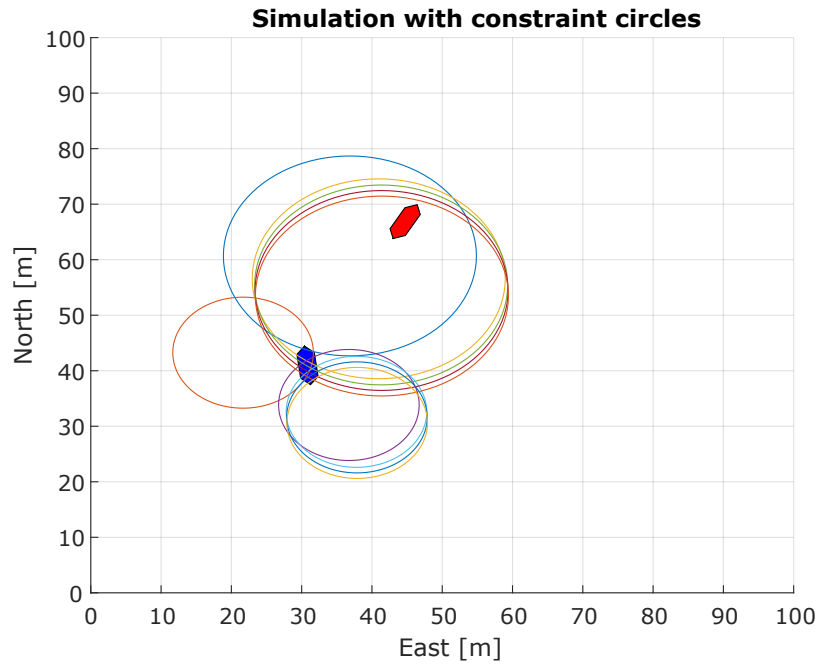
(a) When prediction goes wrong, the OS can get caught by moving constraints. Old style figure.
