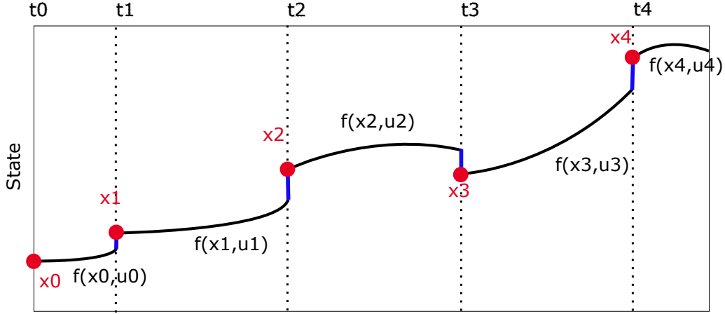
Figure 5: A physically feasible trajectory is formed by "pinching" the shooting gaps close. Reproduction from (Gros 2017).
