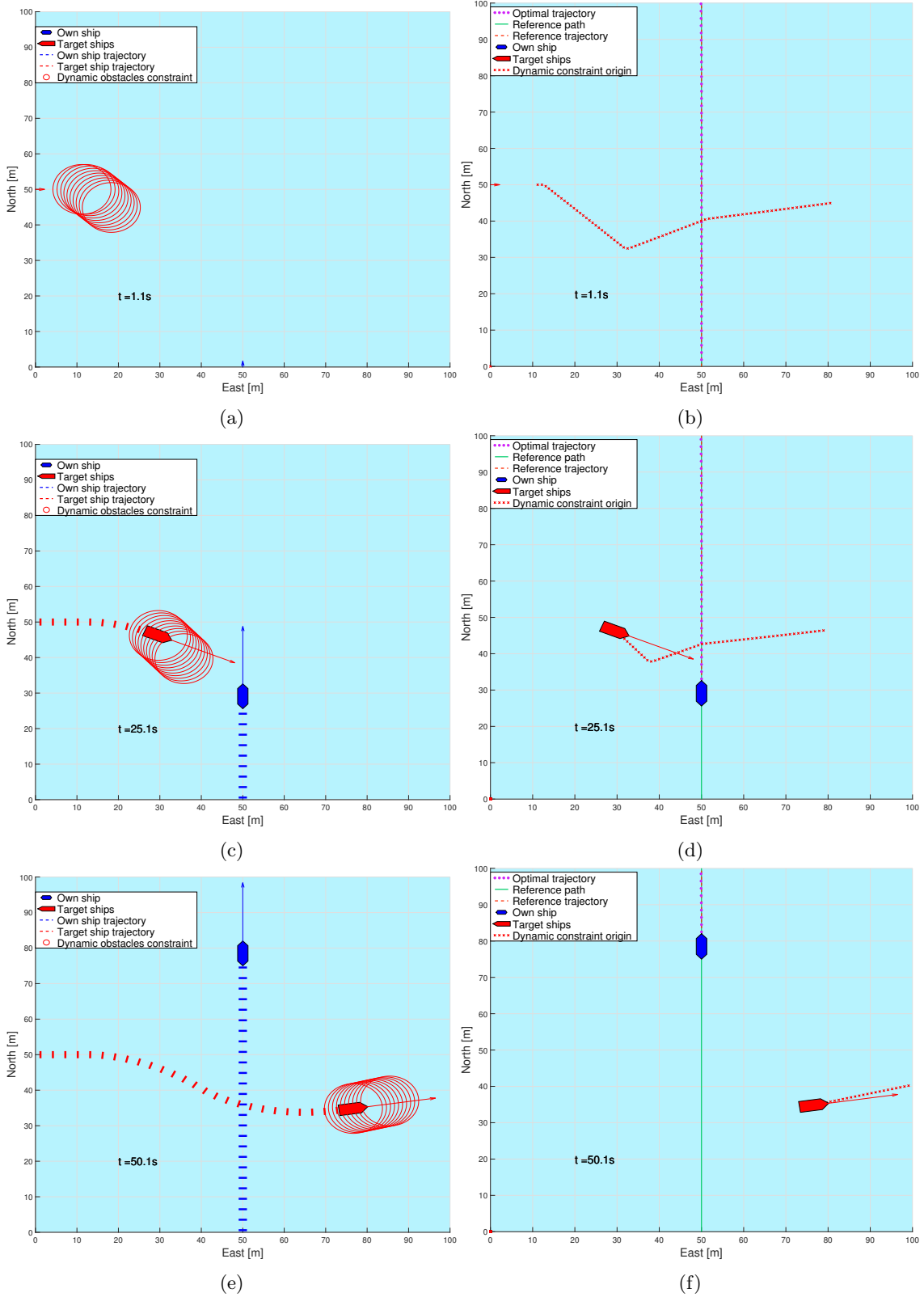
Figure 17: Simple Stand-on. Here shown with full prediction, OS correctly stands on.
