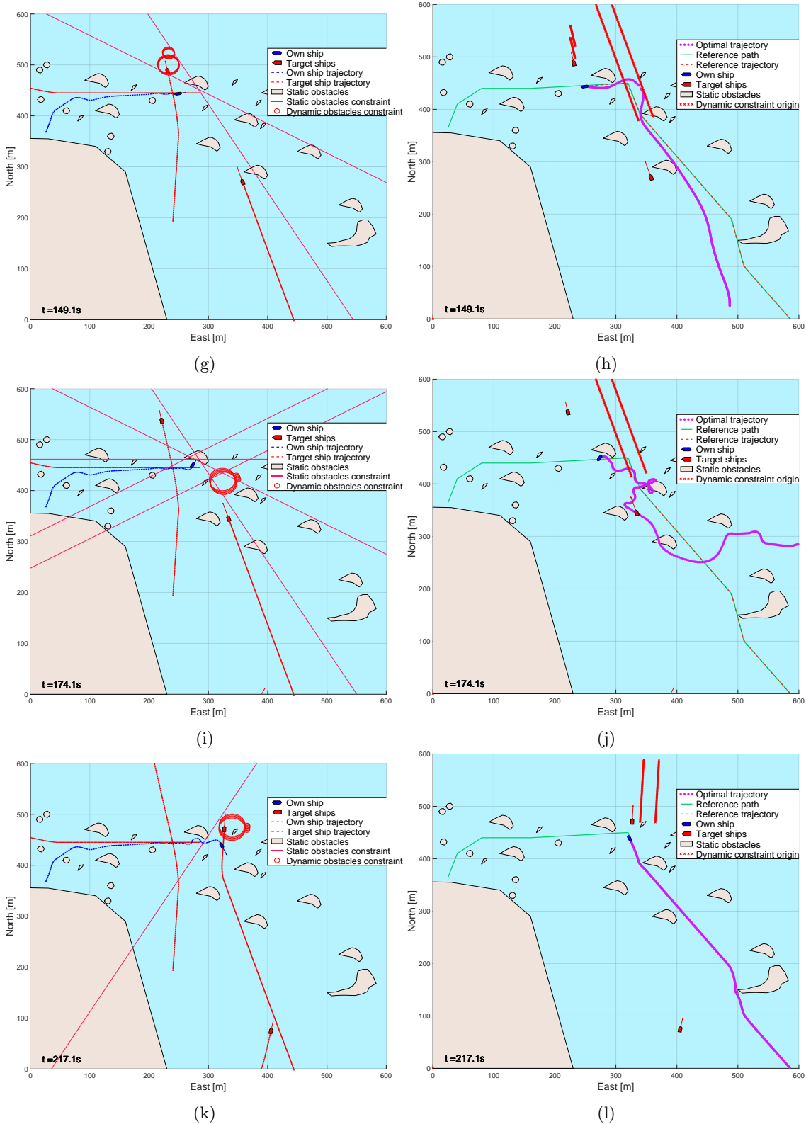
Figure 31: Skjærgård with traffic. Here with simple prediction.
