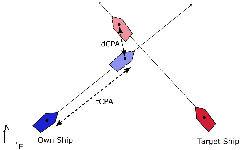
Figure 6: Visualizing dCPA and tCPA.
