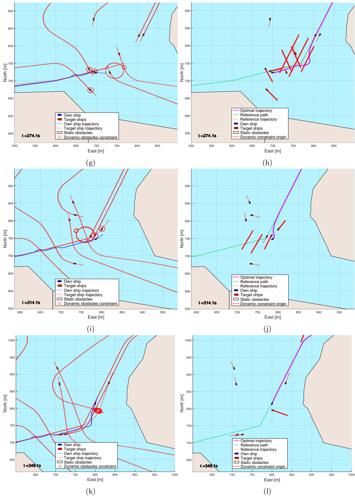
Figure 26: Fjord. Here shown with simple prediction. Observe the OS behaves much more erratically compared to the full prediction level.
