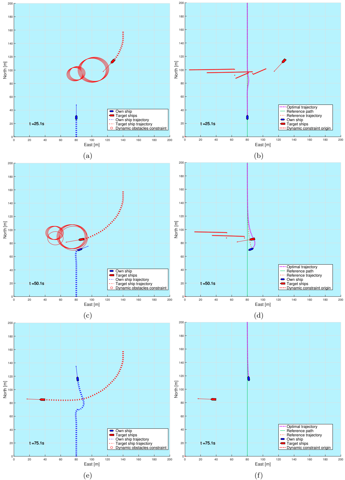
Figure 20: Give-way with a turn, here with full prediction. Observe the OS not expecting to have to yield until it's almost too late.
