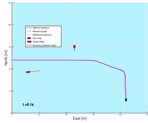
(b) Start of simulation, no active obstacles.
