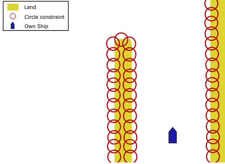
Figure 11: First approach to placing static obstacle constraints, accurate but leads to overload of constraints and poor computational performance.
