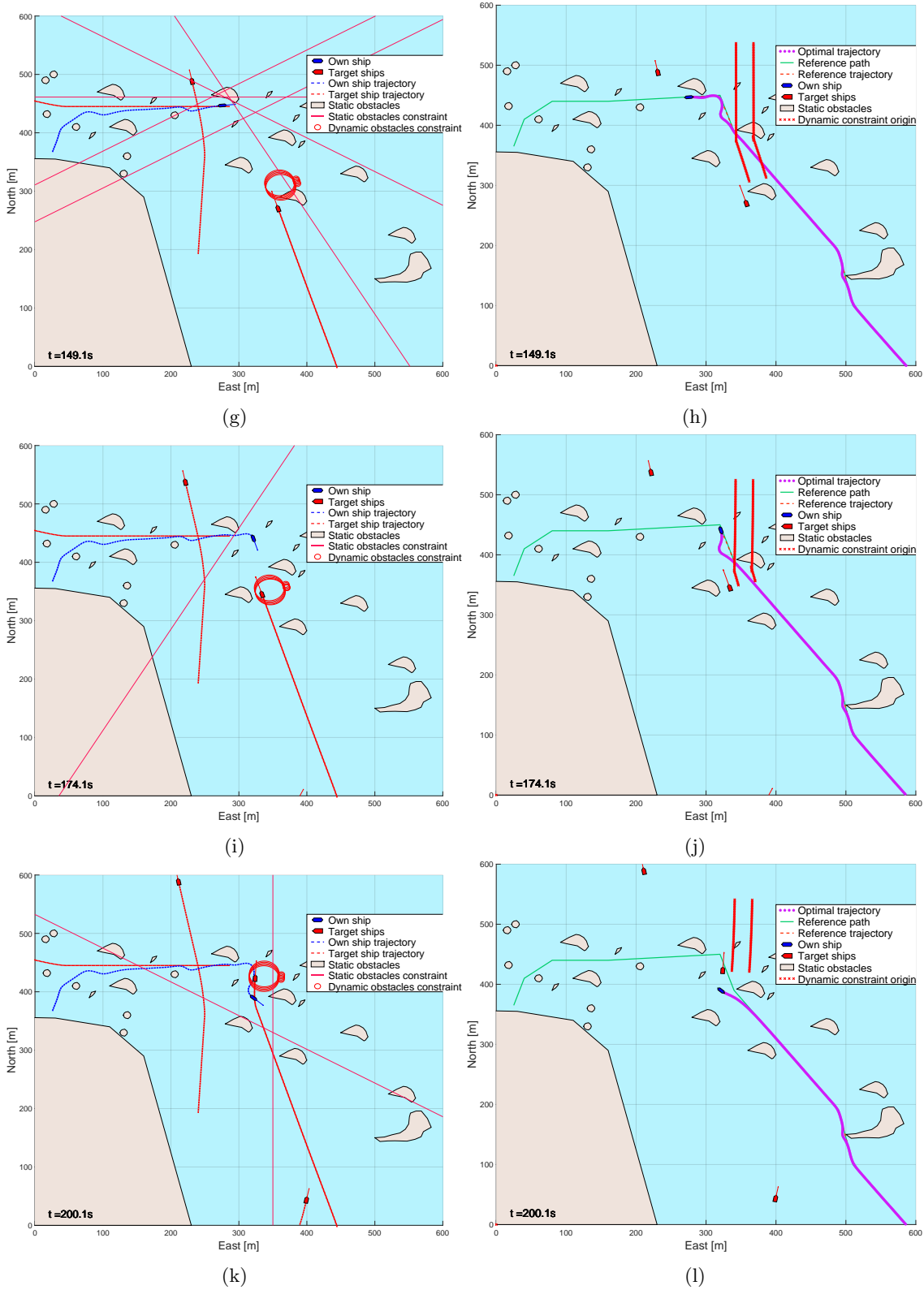
Figure 30: Skjærgård with traffic. Here with full prediction.
