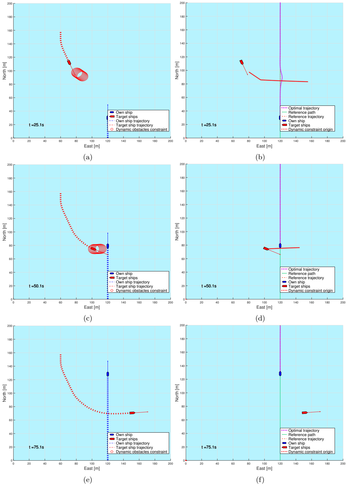
Figure 22: Stand-on with turn. Result independent of prediction level.
