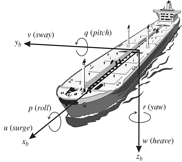
Figure 3: A ship's 6 degrees of freedom, from (Fossen 2011).
