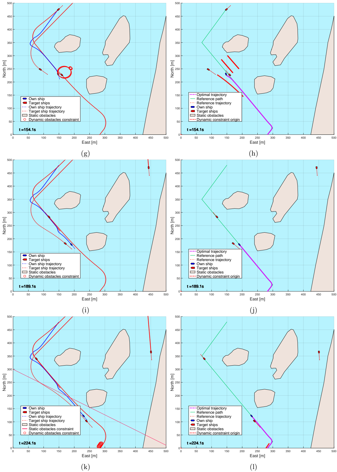
Figure 28: Helløya in reverse. Here with full prediction, the OS behaves to expectations.
