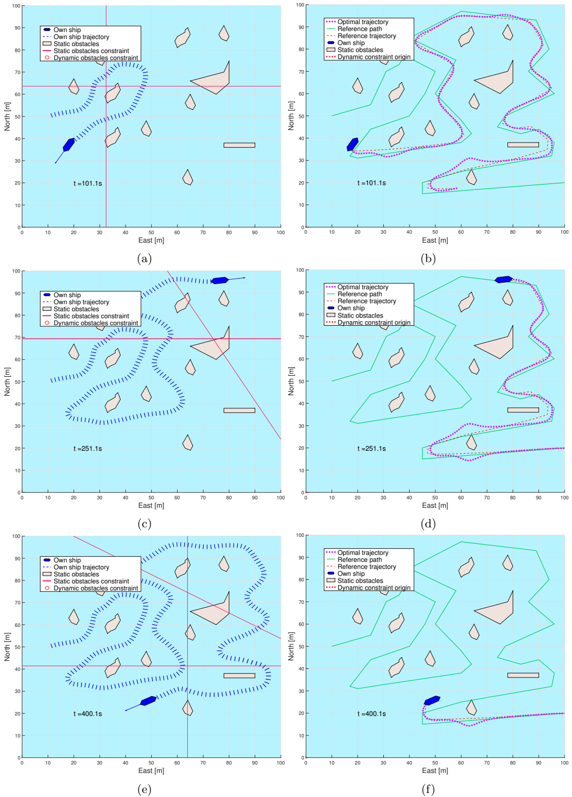
Figure 32: Skjærgård without traffic simulation. Result independent of prediction level due to no TSs.
