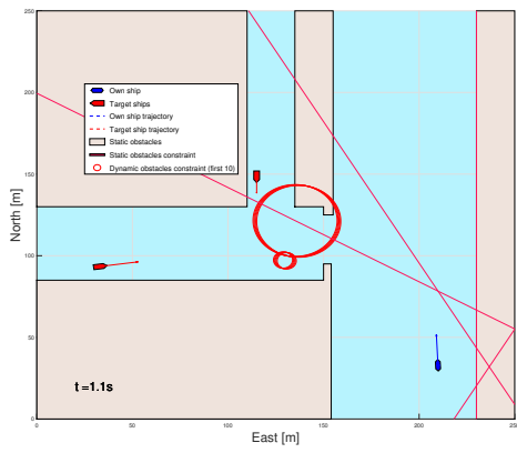
(e) Speed is reduced, resulting in a shorter optimal trajectory.
