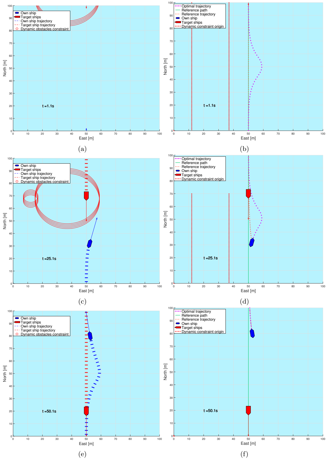
Figure 15: Simple Head-on. Result independent of prediction level.
