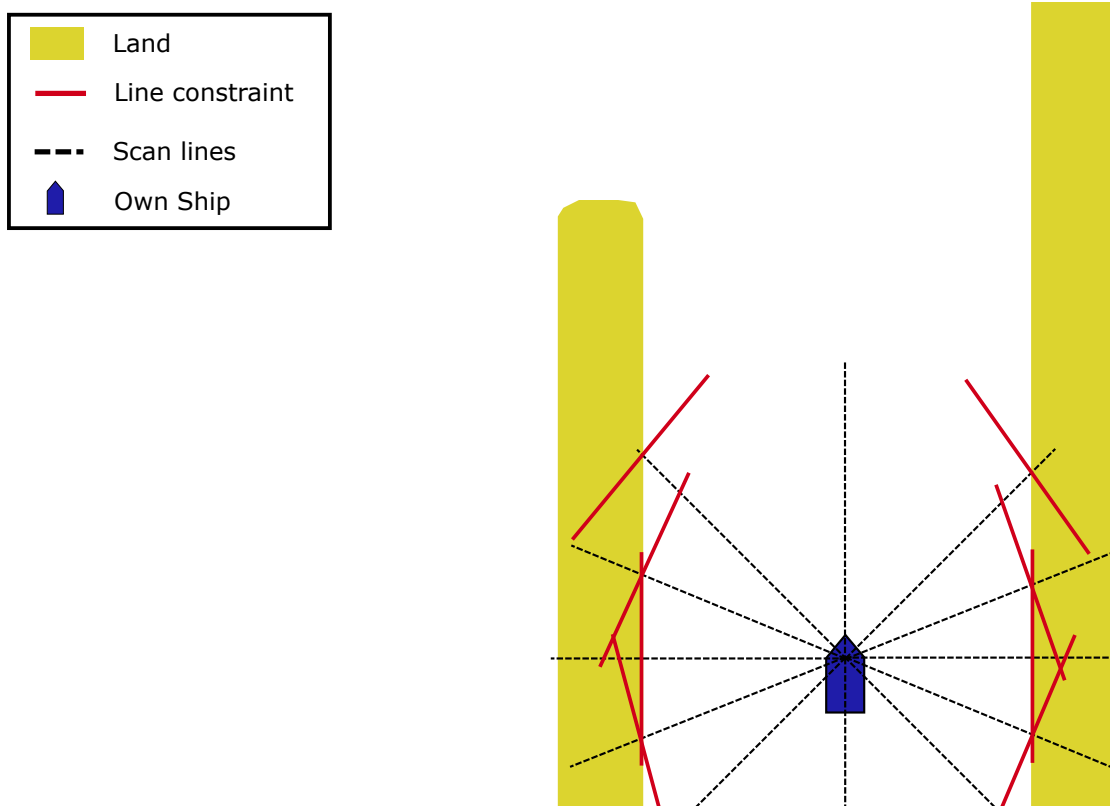
Figure 14: Current approach to placing static obstacle constraints, ditching the circular constraints in favor of straight lines based on proximity. Combines the best of both prior versions.
