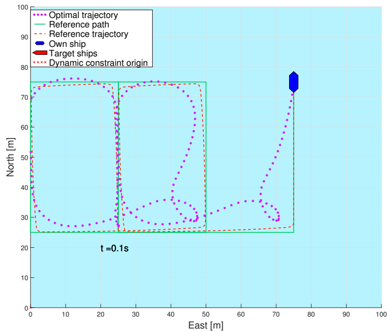
(b) When the heading reference experiences a discontinuity the optimal trajectory becomes weird.
