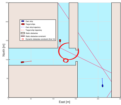
(c) Obstacles activate, breaking the optimal trajectory.
