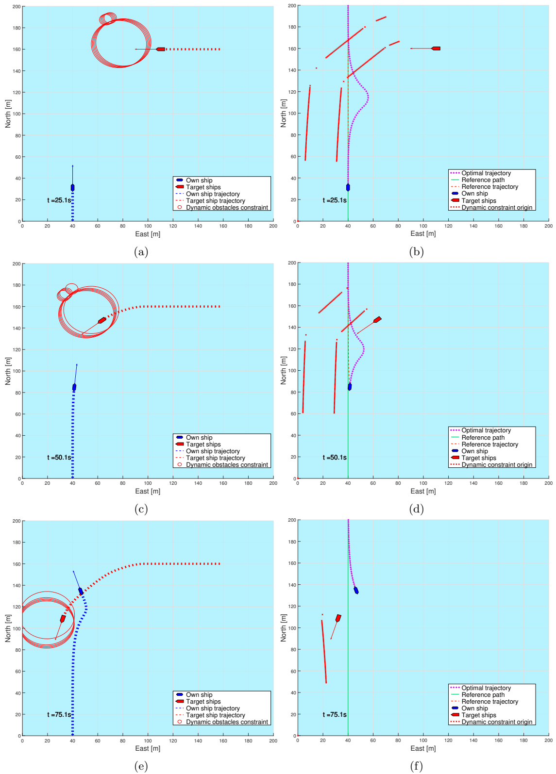
Figure 19: Head-on with a turn. Result for this were the same regardless of prediction level.
