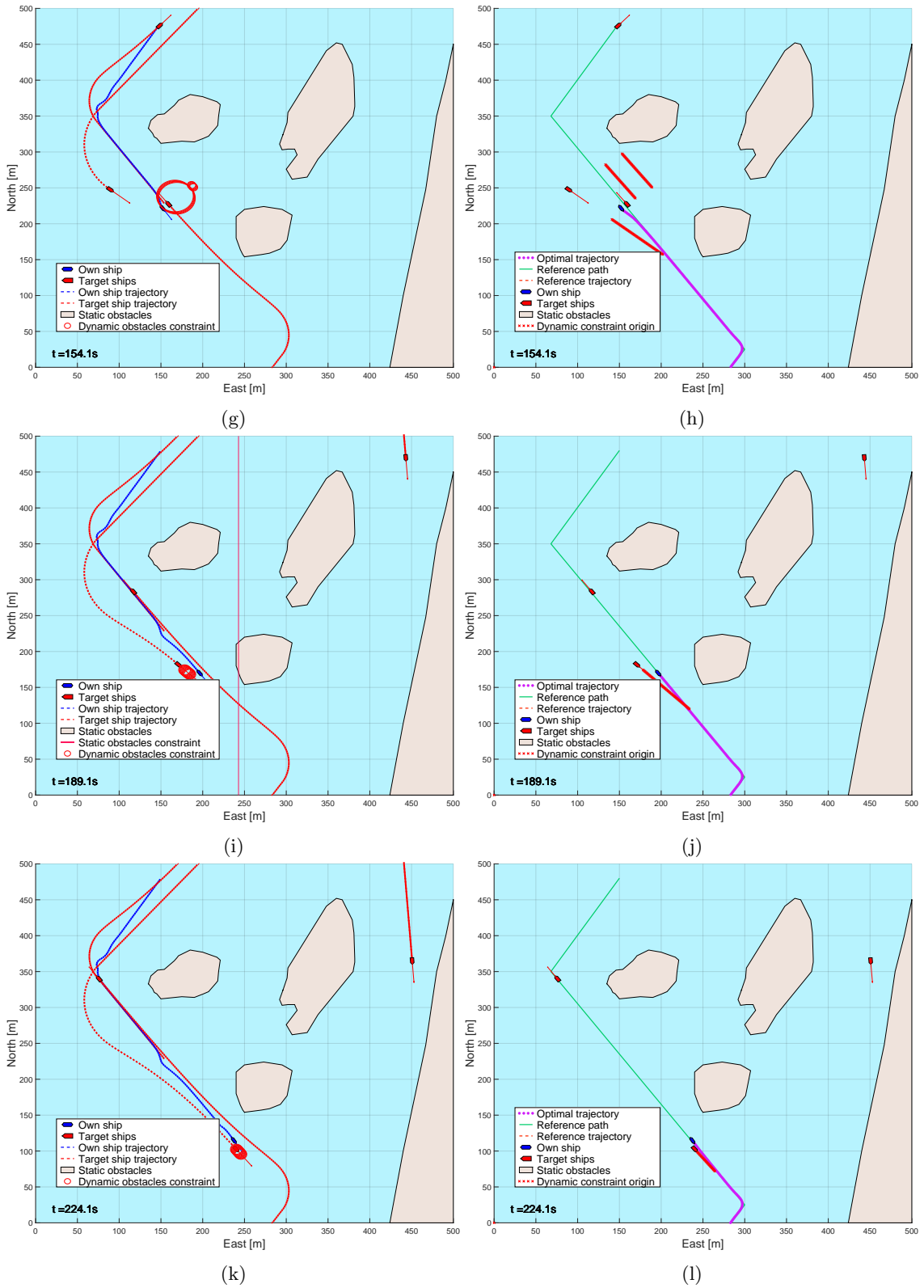
Figure 29: Helløya in reverse. Here with simple prediction, the OS behaves slightly erratically.
