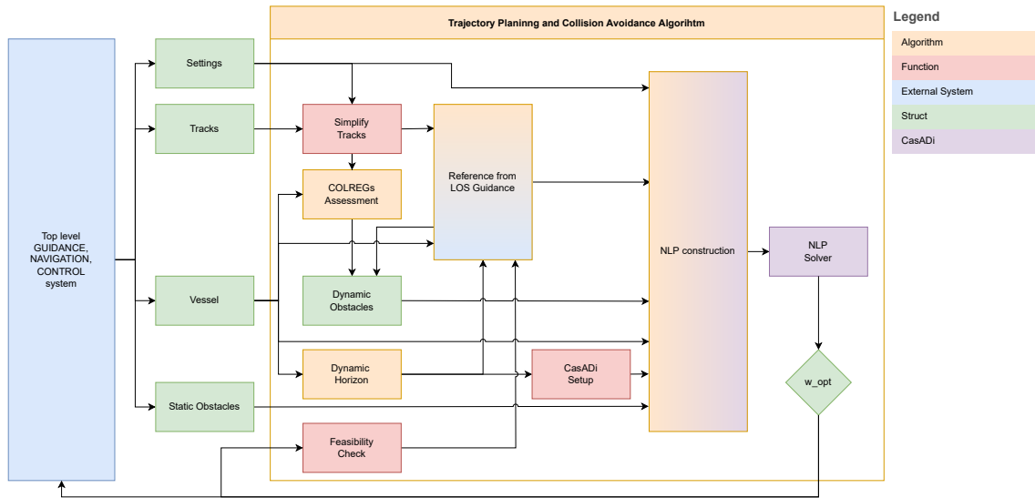
Figure 10: A simplified overview of the developed algorithm.
