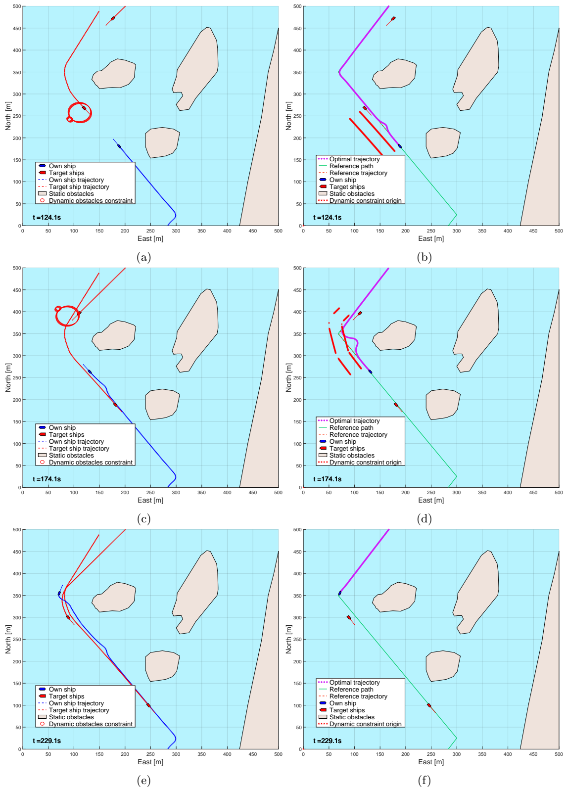
Figure 27: Helløya. Here, the OS behaves to expectations independently of prediction level.
