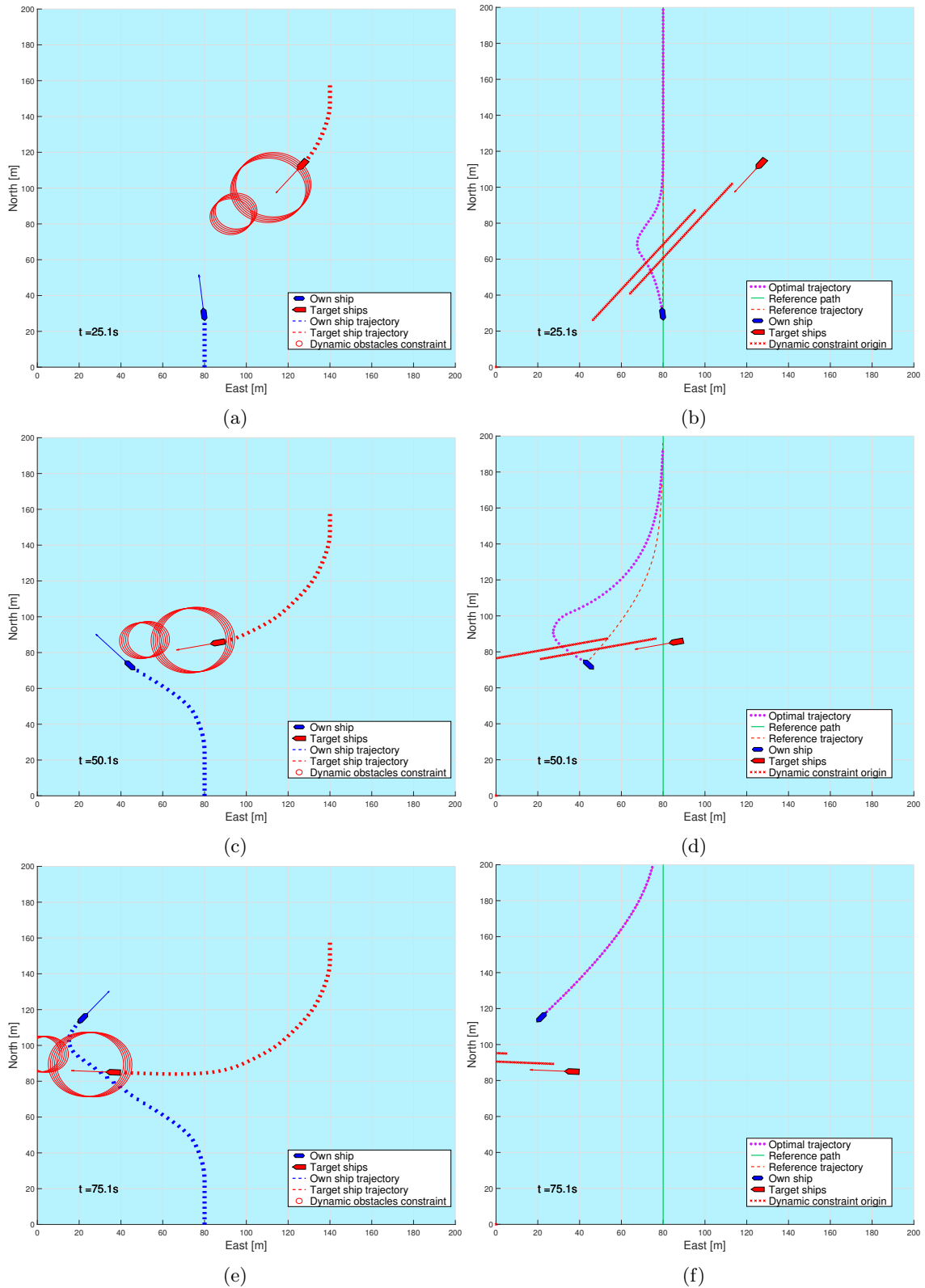
Figure 21: Give-way with a turn, here with simple prediction. Observe as the OS gets dragged along by the constraints of the turning TS.
