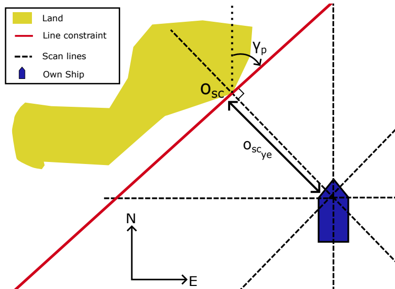
Figure 13: Geometry for straight line constraints used to handle static obstacles.
