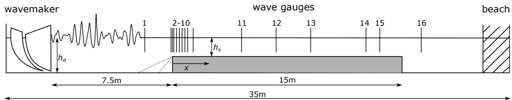
FIGURE 1. Experimental set-up.
