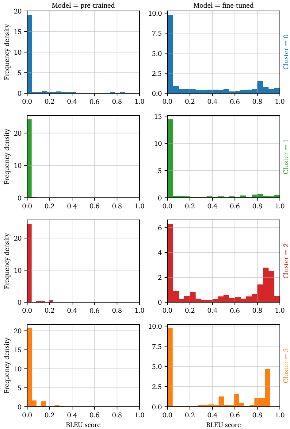
Figure 6.1: BLEU score frequency distribution of generated functions grouped by model and comment cluster, using only comments as model input.
