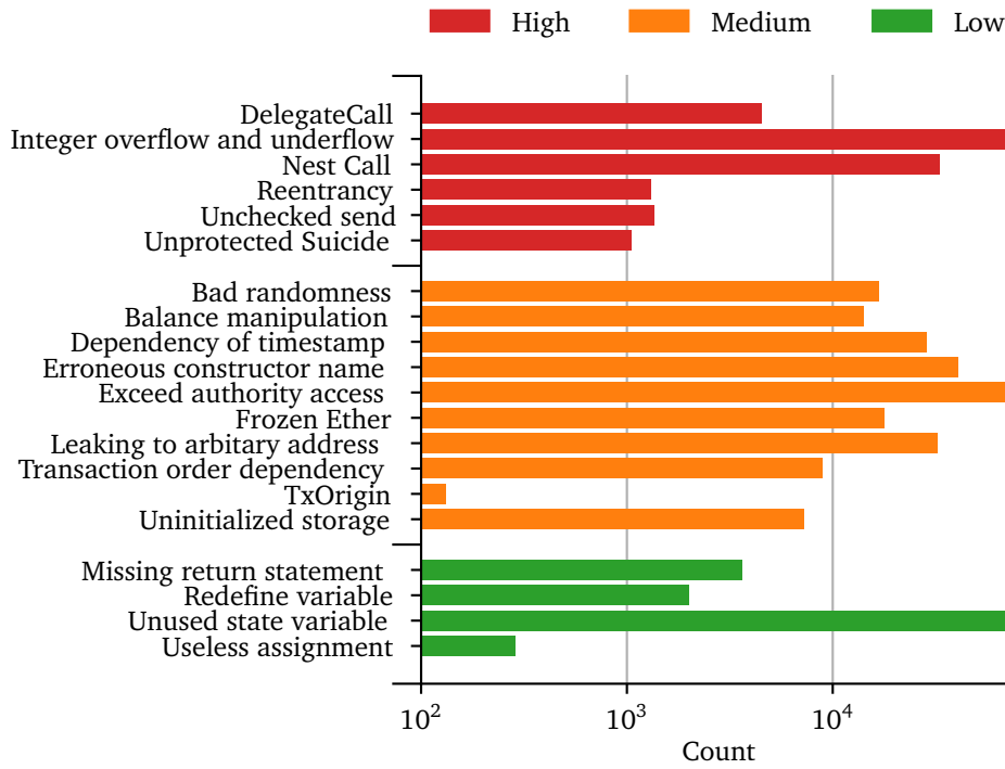
Figure 5.13: Distribution of vulnerabilities in the inflated dataset.
