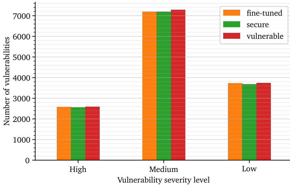
Figure 6.5: Count of vulnerabilities.
