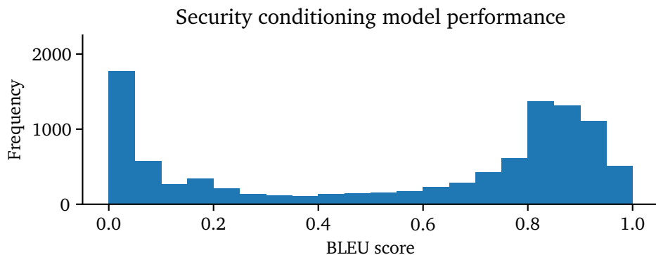
Figure 6.4: BLEU score frequency distribution of 10.000 generated functions with fine-tuned model with security conditioning using comment-aided approach.
