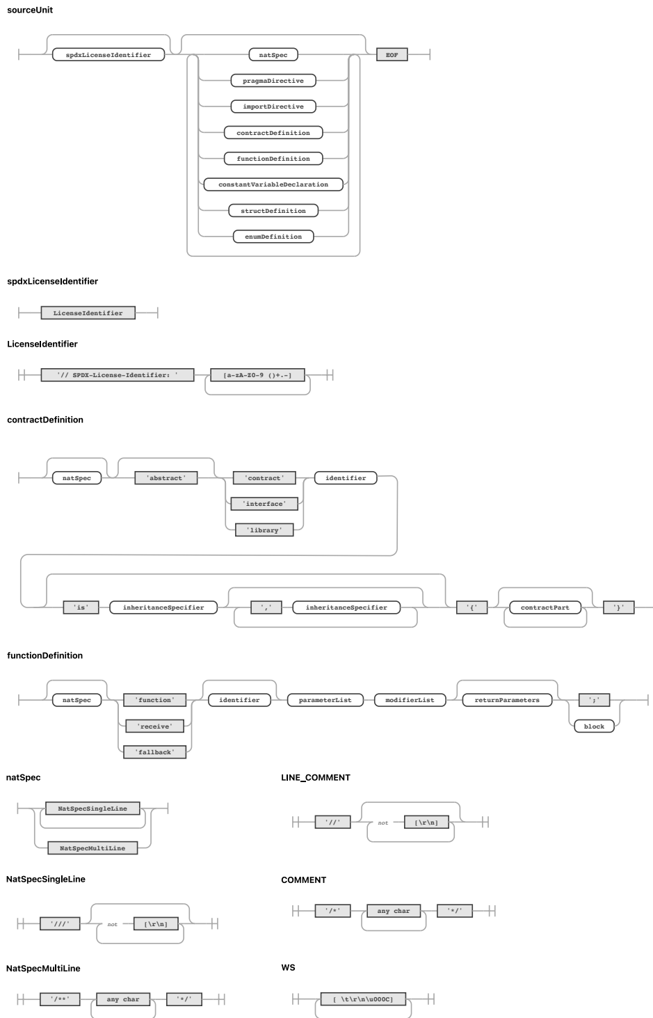
Figure 5.1: Railroad diagrams of main code comment alteration to Solidity grammar.
