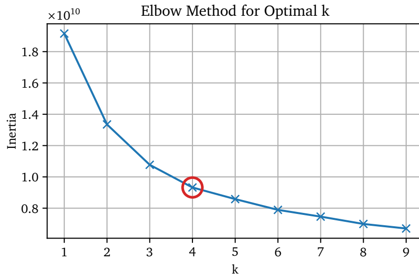
Figure 5.2: Elbow method for determining the optimal number of clusters.
