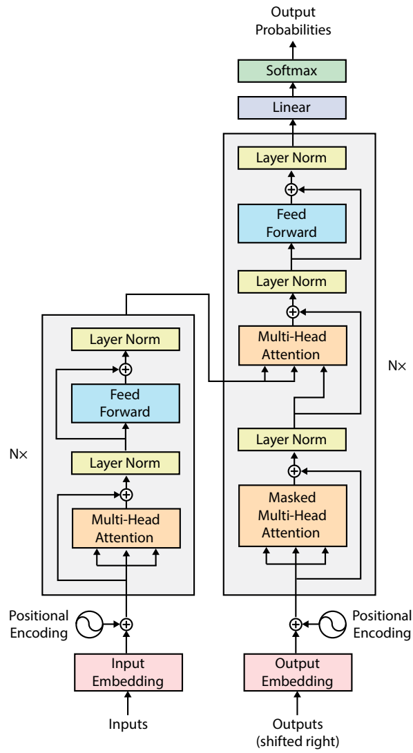
Figure 2.1: Architecture of a standard Transformer Vaswani et al. [6]
