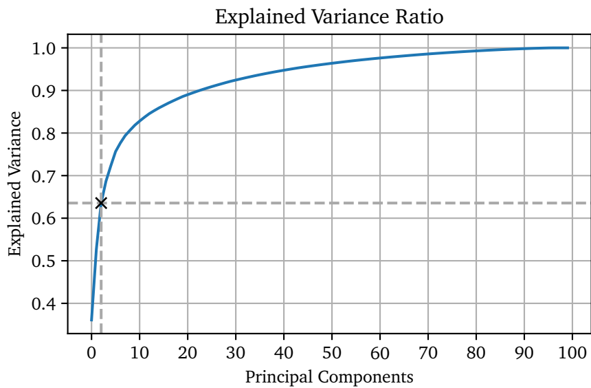
Figure 5.3: Scree Plot for the PCA dimensionality reduction
