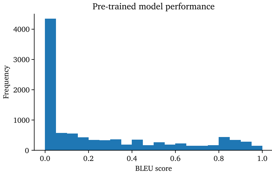
Figure 6.2: BLEU score frequency distribution of 10,000 generated functions with pre-trained model using comment-aided approach.
