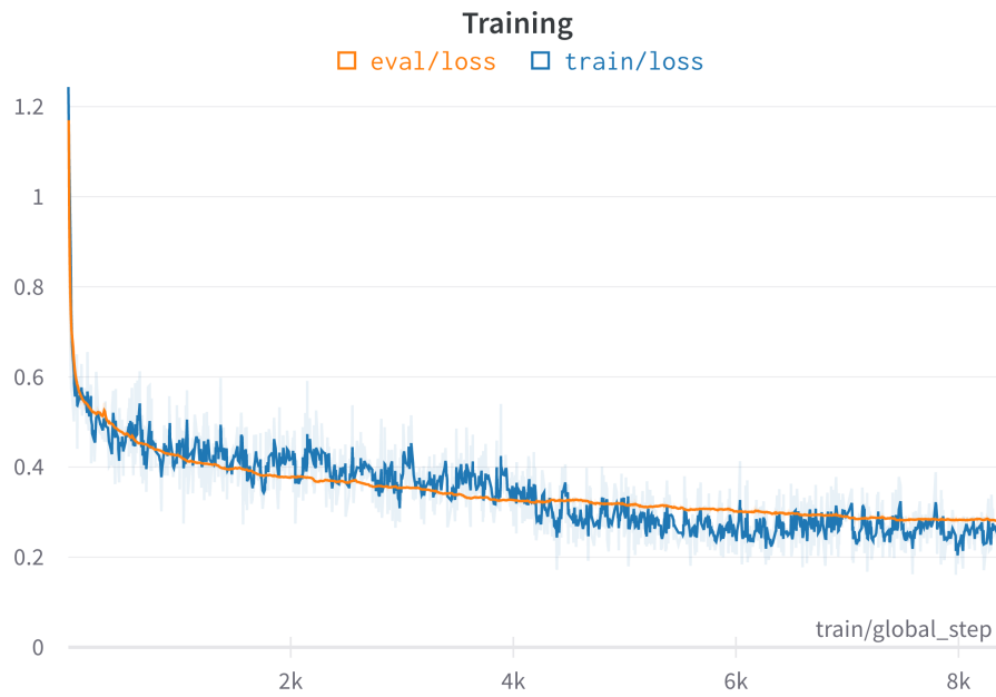
Figure 5.14: Training and evaluation loss during training of model with security conditioning.
