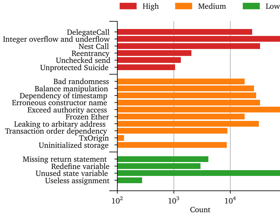
Figure 5.11: Distribution of vulnerabilities in the flattened dataset.
