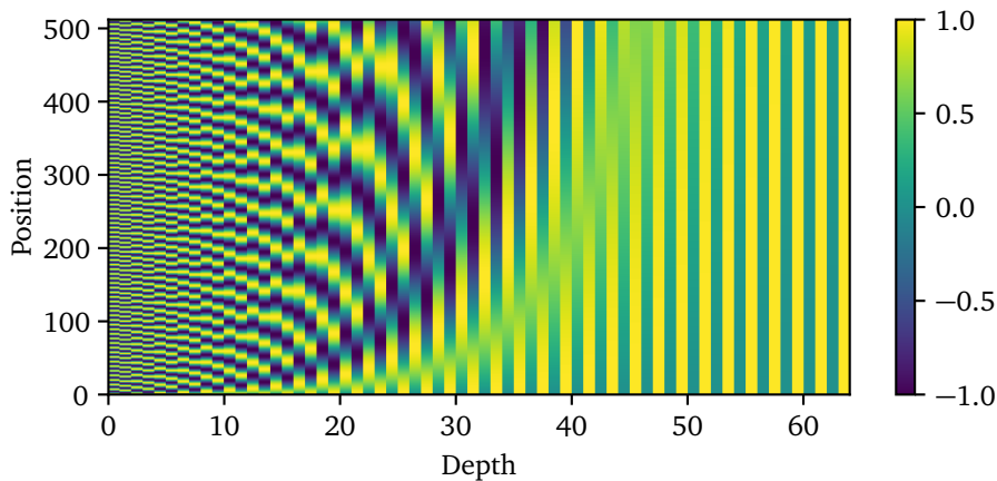
Figure 2.2: The 64-dimensional positional encoding for a sentence with the maximum length of 512. Each row represents an positional encoding vector.
