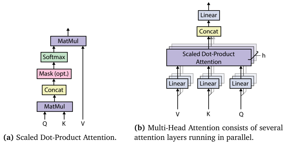
Figure 2.3: Multi-Head Attention module in Transformer architecture Vaswani et al. [6]
