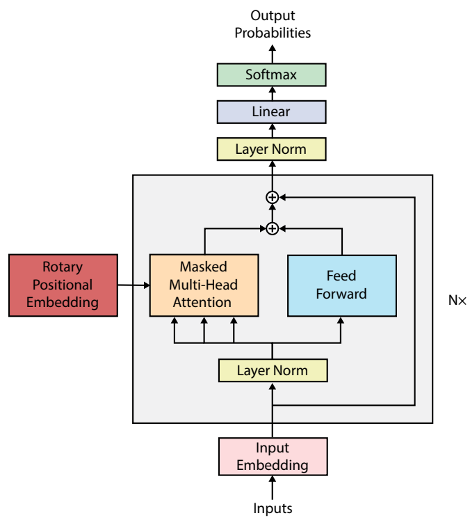
Figure 4.2: Diagram of GPT-J model architecture.
