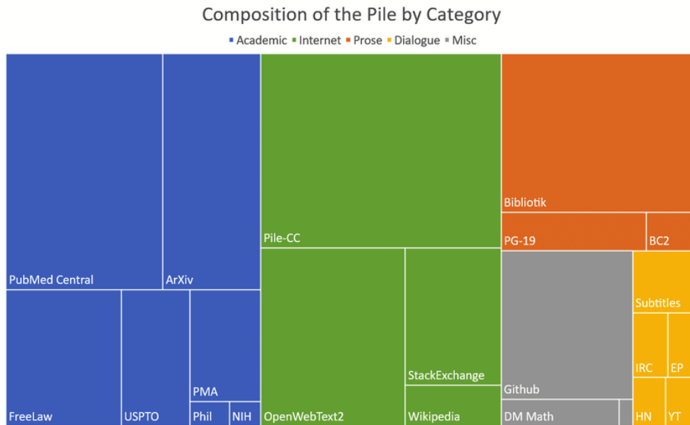
Figure 4.1: Treemap of the Pile components by effective size. Source: [46]
