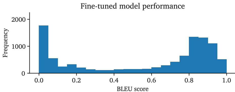
Figure 6.3: BLEU score frequency distribution of 10,000 generated functions with fine-tuned model using comment-aided approach.
