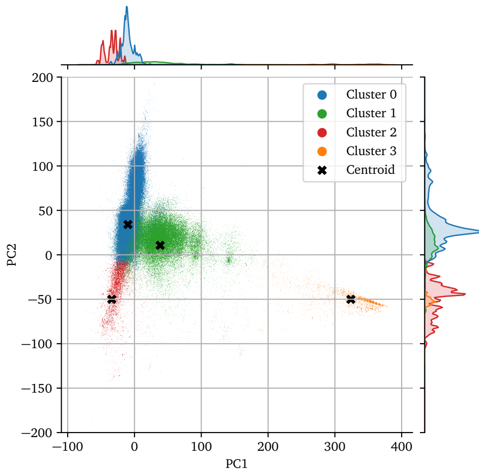
Figure 5.4: 2D plot of the comment clusters.
