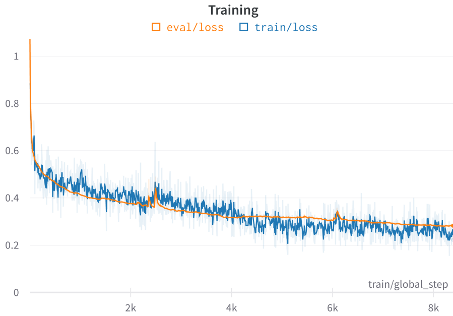
Figure 5.7: Training and evaluation loss during model training.
