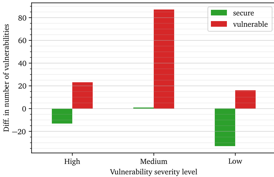
Figure 6.6: Difference in count of vulnerabilities compared to fine-tuned model without security conditioning.
