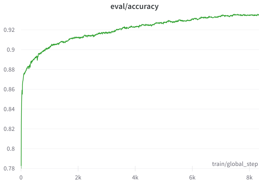
Figure 5.15: Evaluation plot of accuracy during training of model with security conditioning.
