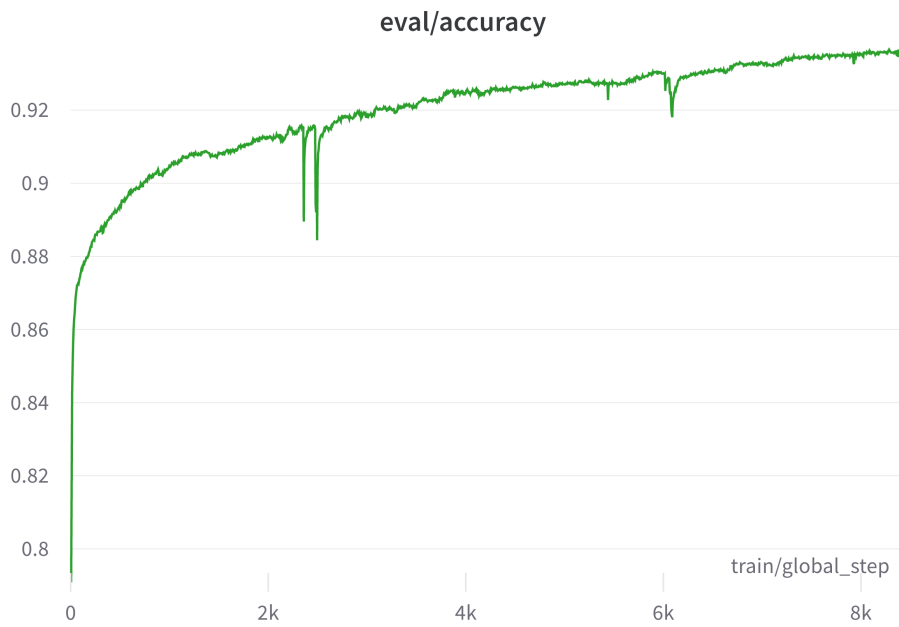
Figure 5.8: Evaluation accuracy during model training.
