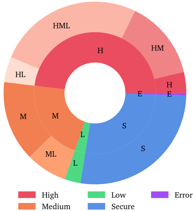
Figure 5.12: Doughnut chart over the distribution of the vulnerability severities in the inflated dataset at different granularity levels, where each level occurs at least once in the SC.
