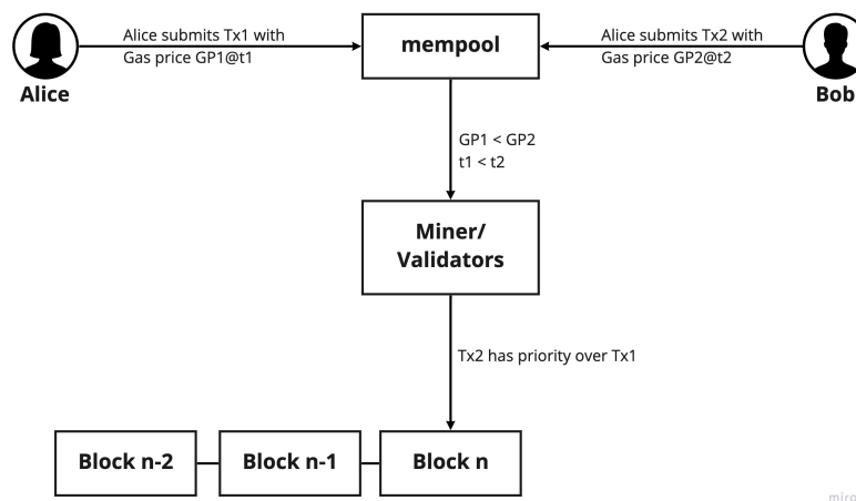
Figure 2.12: Illustration of frontrunning in blockchain
