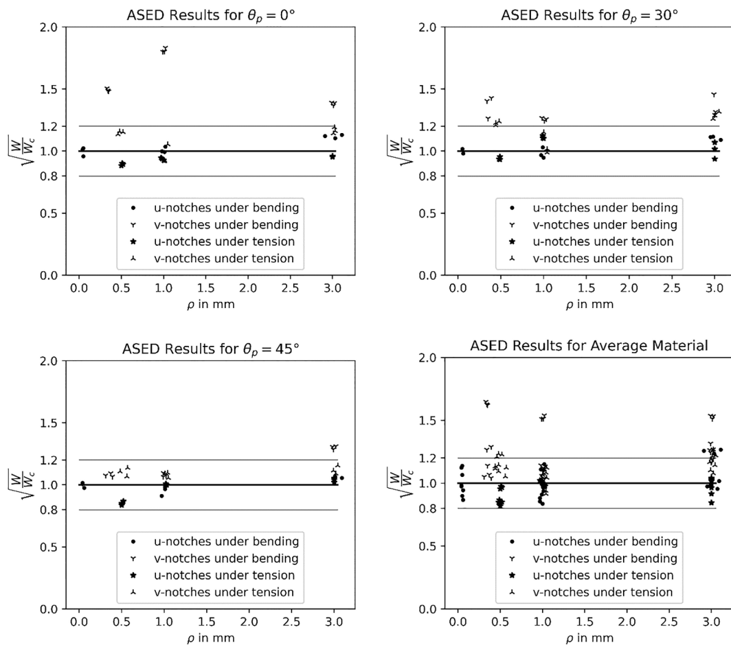
Fig. 10. Accuracy of the ASED criterion applied to the data from [33] using the R_0 from Fig. 9. The thin lines denote the \pm 20\% scatter band. The predictions are given numerically in Table B.1 in the appendix.
