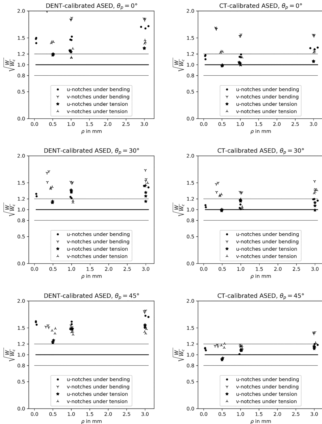
Fig. 8. Relatively low accuracy of the ASED criterion applied to the data from [33] using the K_{Ic} values from Tables 1 and 3. Left: K_{Ic} from tensile test; Right: K_{Ic} from CT specimen. The thin lines denote the \pm 20\% scatter band. The predictions are given numerically in Tables B.2 and B.3 in the appendix.
