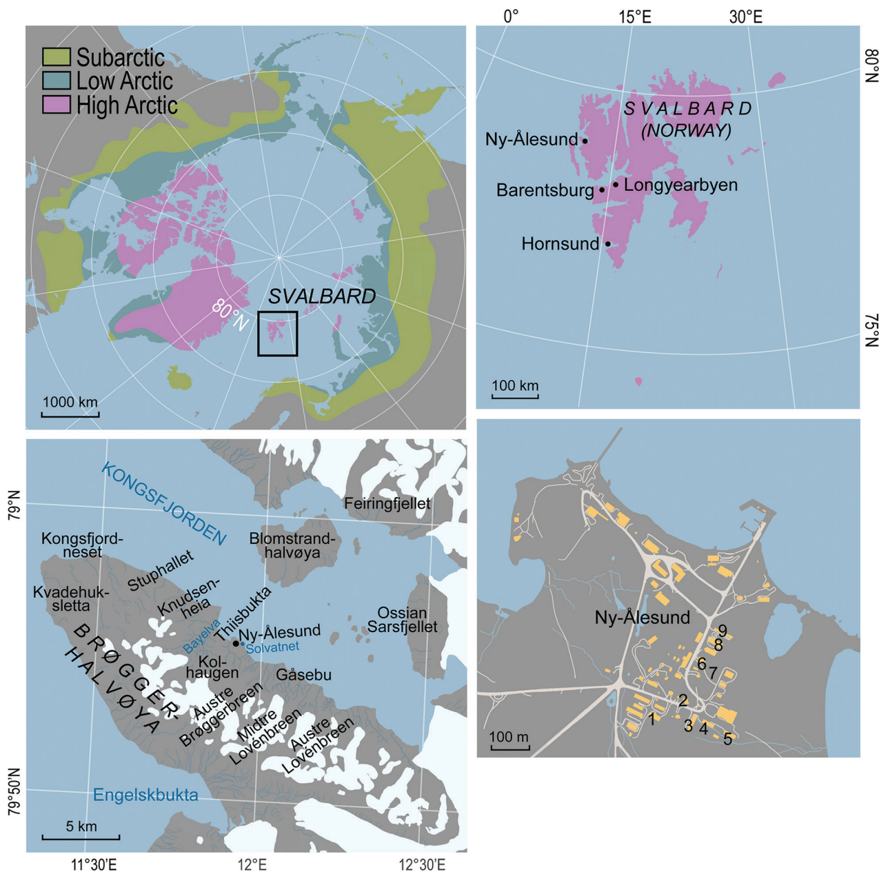
Fig. 1 The location of Svalbard, Brøggerhalvøya and Ny-Ålesund in the circumpolar Arctic. In Ny-Ålesund, the nine research stations are as follows: (1) National Research Council (Italy); (2) Alfred Wegener Institute for Polar and Marine Research (Germany) and the Polar Institute Paul Emile Victor (France); (3) Norwegian Polar Institute; (4) Korea Polar Research Institute; (5) Polar Research Institute of China; (6) National Centre for Polar and Ocean Research (India); (7) National Institute of Polar Research (Japan); (8) Natural Environmental Research Council (UK); (9) University of Groningen (Netherlands). (Figure by S.M. Kristiansen.)
