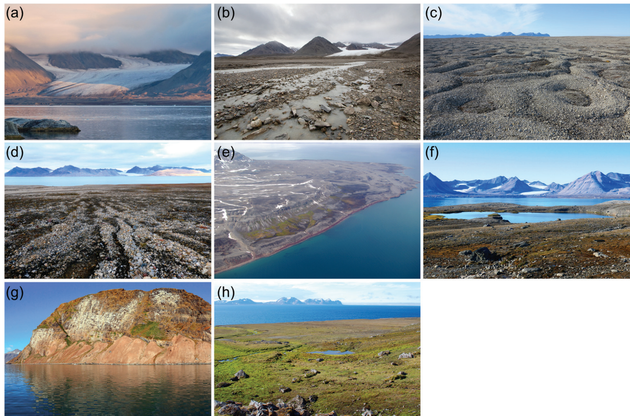
Fig. 2 Dominant landforms and habitats close to Ny-Ålesund. (a) The Midtre Lovénbreen glacier. (b) Moraine with braided streams below the Midtre Lovénbreen glacier. (c) Sorted stone circles at Kvadehuksletta. (d) Sorted stone stripes at Stuphallet. (e) View of the north-western peninsula, showing the plateaued landscape and the bird cliffs at Stuphallet, where nesting seabirds introduce marine-derived nutrients, leading to extensive plant growth. (f) Inland lake on Blomstrandhalvøya, where shorebirds and waterfowl breed. (g) Ossidian Sarsfjellet, a bird cliff, where summertime nutrient inputs from nesting black-legged kittiwakes ( Rissa tridactyla ), coupled with an exceptionally mild microclimate, lead to high diversity of vascular plants and bryophytes. (h) Moss tundra habitat in flat lowlands beneath bird cliffs at Simlestupet. (Photo a by F. Samuelsson; b by E.M. Biersma; c and h by Å.Ø. Pedersen; d, f and g by J. Mosbacher; and e by P. Convey).
