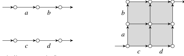
Figure 21. HDAs X = \square^{(a<b)} and Y = \square^{(c<d)} (left) and their tensor product X \otimes Y .
