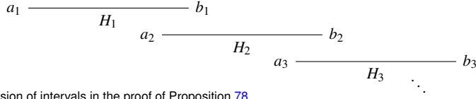
Figure 19. Progression of intervals in the proof of Proposition 78.
