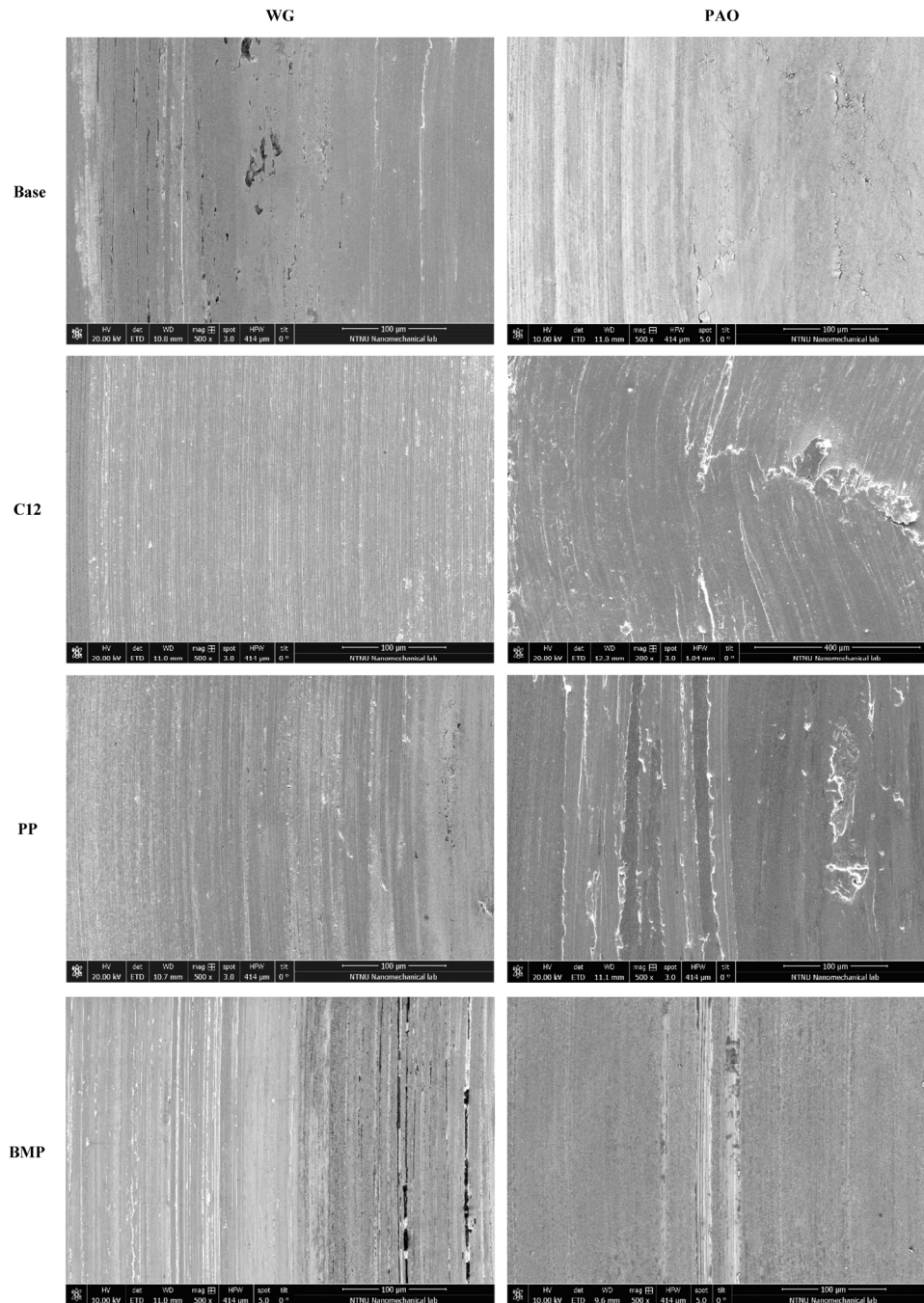
Fig. 4 SEM images of the wear tracks on stainless steel disk tested in different lubricants at room temperature. Pictures were taken with 500x magnification except for PAO-C12 with 200 \times magnification.
