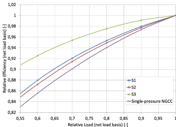
Fig. 8. Optimal steady-state net efficiencies for three different GC control strategies when operating at part loads. The three strategies are compared to a readily available technology, i.e. a single-pressure natural gas combined cycle.
