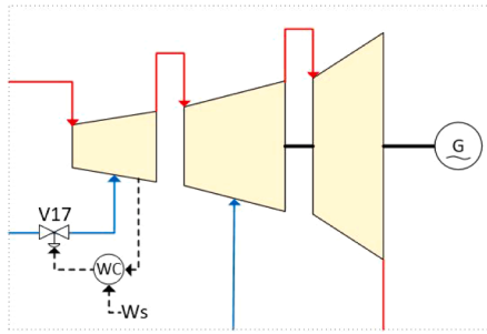
Fig. 6. Section of the closed control loop of control strategy S2 and S3 illustrating the control of the cooling stream to the first section of the turbine (i.e. HTT1).
