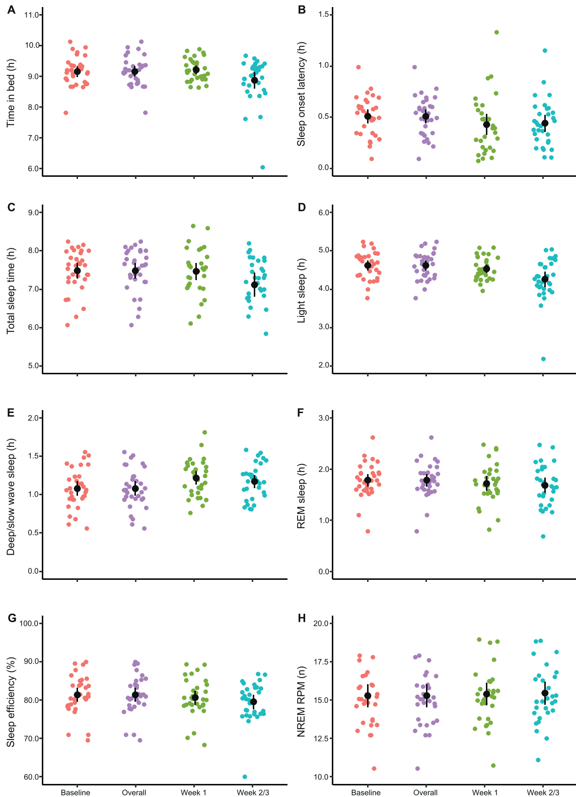
Fig. 1. Visualization of the descriptive data for the measured sleep variables. Data is based on sleep monitoring in 33 elite endurance athletes at near-sea-level baseline (pink dots) and at altitude overall (purple dots), week 1 (green dots) and weeks 2 and 3 combined (blue dots). Each data point represents each athletes' mean score in the respective sleep variables. The filled black dot represents the mean for the whole group, with upper and lower 95% confidence intervals represented by the bar intersecting the mean. (Color version of figure is available online.)
