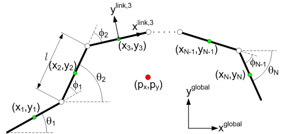
Fig. 1. Kinematic parameters for the snake robot.
