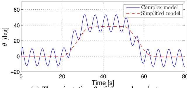
(c) The orientation \theta of the snake robot.
