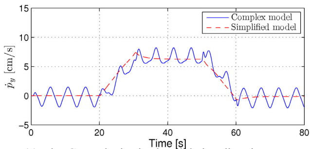
(e) The CM velocity in the global y direction, \dot{p}_y .
