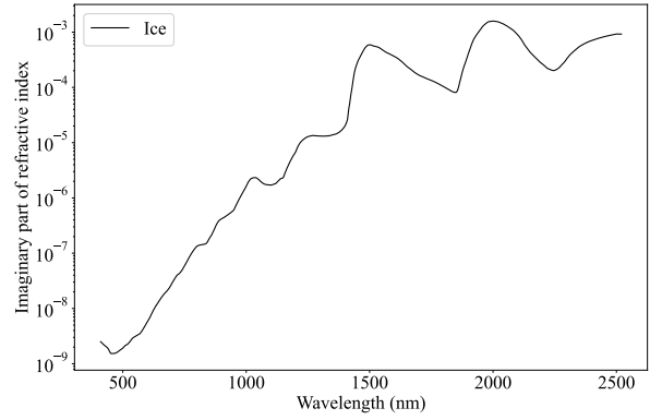
Figure 1. Evolution of the imaginary part of the ice refractive index based on the database in [22]. The y-axis is displayed in logarithmic scale.
