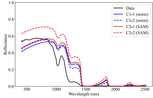
Figure 9. Spectra obtained from the model used with \beta and M estimated by cost functions and approaches for the image acquired at t_1 = 23 min.
