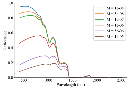
Figure 2. Influence of the concentration of pollutants for a grain size of 1000 \mu\text{m} .
