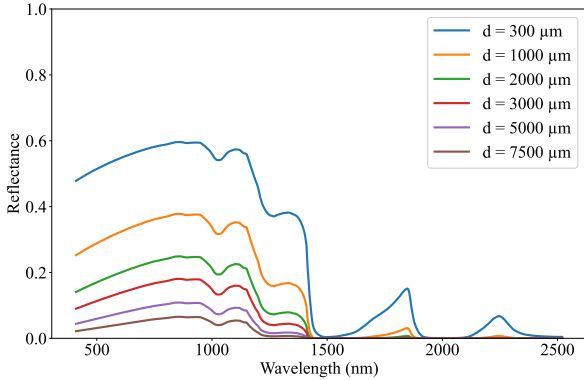
Figure 3. Influence of the snow grain size for a concentration of pollutants of 3.10^{-6}
