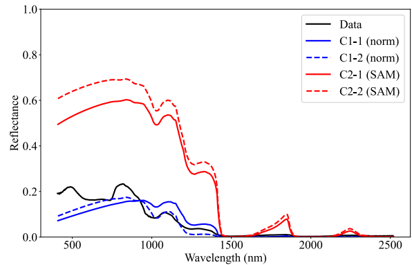
Figure 10. Spectra obtained from the model used with \beta and M estimated by cost functions and approaches for the image acquired at t_2 = 88 min.
