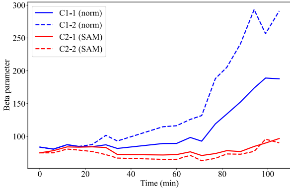
Figure 8. Estimation of \beta parameter using the two cost functions \mathcal{C}_1 and \mathcal{C}_2 with two approaches of optimization.
