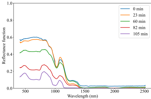
Figure 6. Full spectrum reconstructed for a couple of images along the experiment. The VNIR and SWIR spectra were connected using the shared overlap between 950 nm and 1000 nm.
