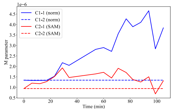
Figure 7. Estimation of M parameter using the two cost functions \mathcal{C}_1 and \mathcal{C}_2 with the first approach of optimization.
