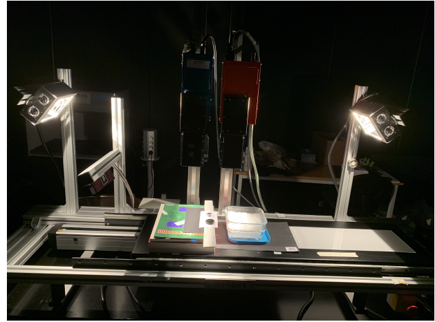
Figure 4. Experimental setup for the acquisition. The Spectralon® and the snow sample are placed on a moving platform whose speed is controlled by a computer and linked to the integration time of each camera. The platform is moving from right to left on this picture.
