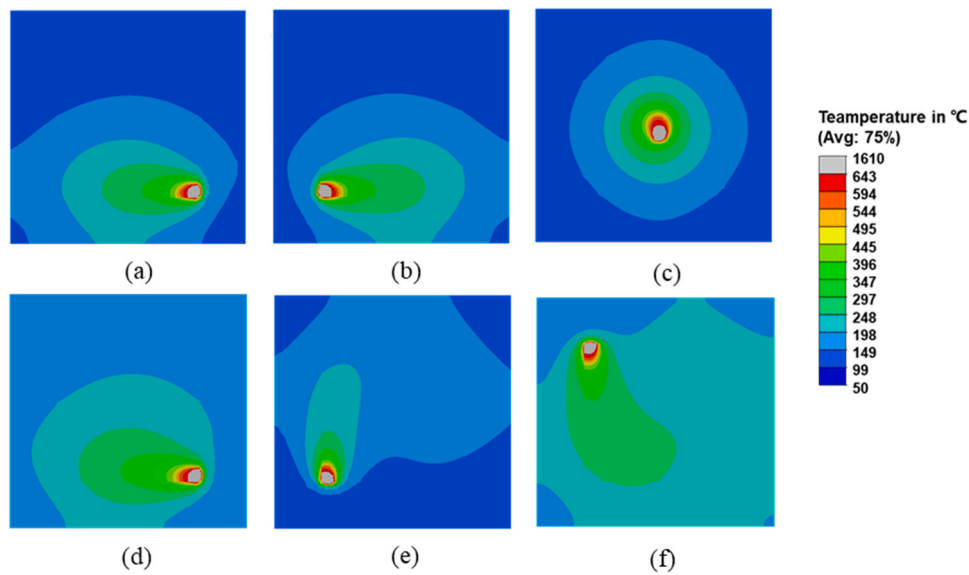
Fig. 9. The transient temperature fields of the six patterns at the end of the deposition process, (a) Raster; (b) Zigzag; (c) Out-in spiral; (d) Alternate-line; (e) In-out spiral; (f) S. The grey color shows the melting zone.
