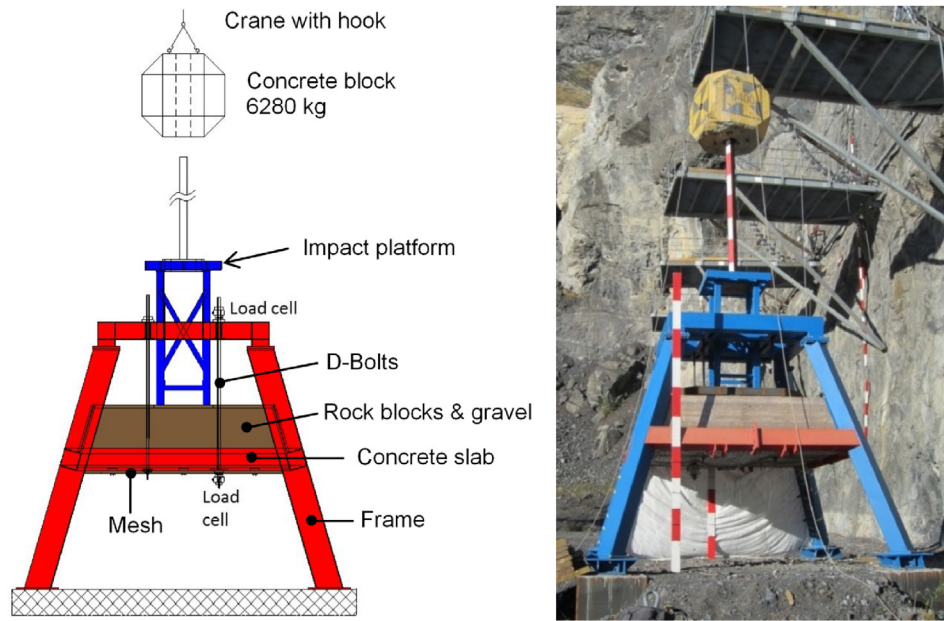
Fig. 17. The setup for the full-scale impact tests (Roth, 2014).
