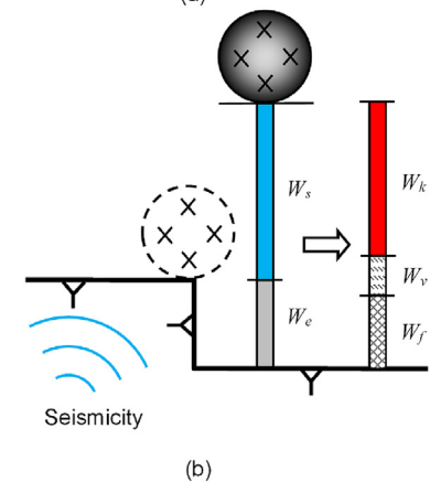
Fig. 12. Conceptual models for (a) self-initiated strain burst and (b) fault-slip rockburst. The crosses in the ball mean that the rock is pre-fractured prior to the burst event.
