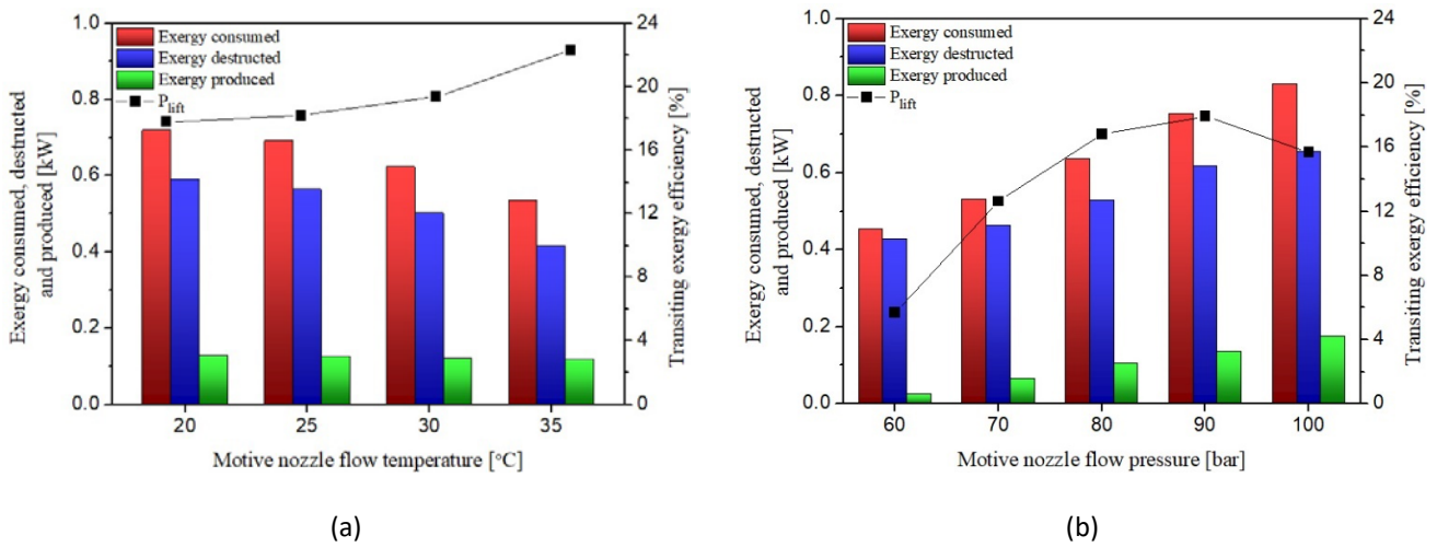
Figure 13: Ejector exergy metrics at different motive nozzle flow temperatures and pressure at T_{evap} = -6^\circ\text{C} , (a) P_{rec} \approx 35.4 bar and P_{MN} = 34.5 bar, (b) P_{rec} \approx 34.6 bar and T_{MN} = 20^\circ\text{C} .
