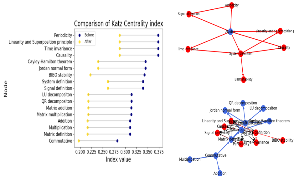
Figure 42: Katz centrality calculated on the 'Systems Theory' learning graph before and after replacing super nodes, using the method that connect to the nodes with incoming and outgoing edges. The values are calculated using a damping factor of \alpha = 0.1 and an initial centrality of \beta = 1.0 .
