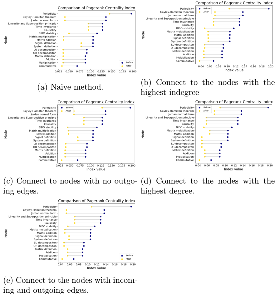
Figure 45: Pagerank centrality index comparison showing how the index changes for every method.
