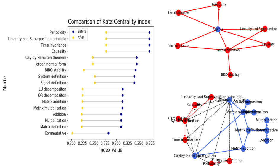
Figure 27: Katz centrality calculated on the 'Systems Theory' learning graph before and after replacing super nodes, using the method that connect to the nodes with the highest indegree. The values are calculated using a damping factor of \alpha = 0.1 and an initial centrality of \beta = 1.0 .
