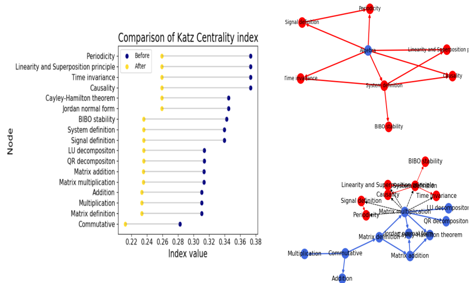
Figure 37: Katz centrality calculated on the 'Systems Theory' learning graph before and after replacing super nodes, using the method that connect to the nodes with the highest degree. The values are calculated using a damping factor of \alpha = 0.1 and an initial centrality of \beta = 1.0 .
