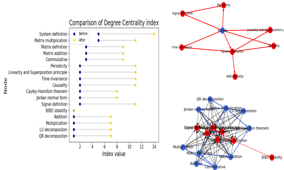
Figure 20: Degree centrality calculated on the ‘Systems Theory’ learning graph before and after replacing super nodes, using the naive method.
