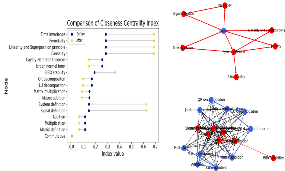
Figure 23: Closeness centrality calculated on the ‘Systems Theory’ learning graph before and after replacing super nodes, using the naive method.
