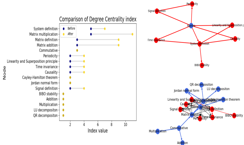
Figure 40: Degree centrality calculated on the 'Systems Theory' learning graph before and after replacing super nodes, using the method that connect to the nodes with incoming and outgoing edges.
