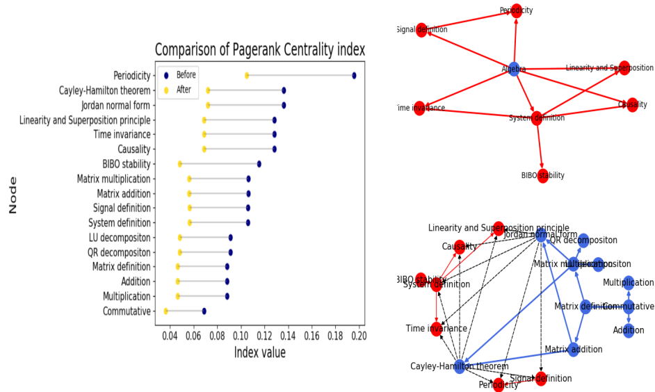
Figure 26: PageRank centrality calculated on the 'Systems Theory' learning graph before and after replacing super nodes, using the method that connect to the nodes with the highest indegree. The values are calculated using a damping factor of \alpha = 0.85 .
