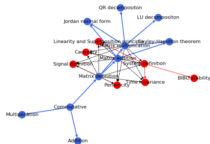
(f) Connect to the nodes with incoming and outgoing edges.
