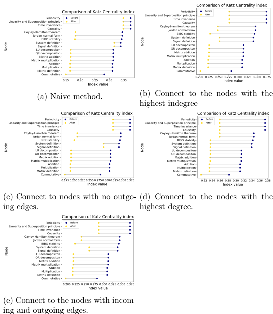
Figure 46: Katz centrality index comparison showing how the index changes for every method.
