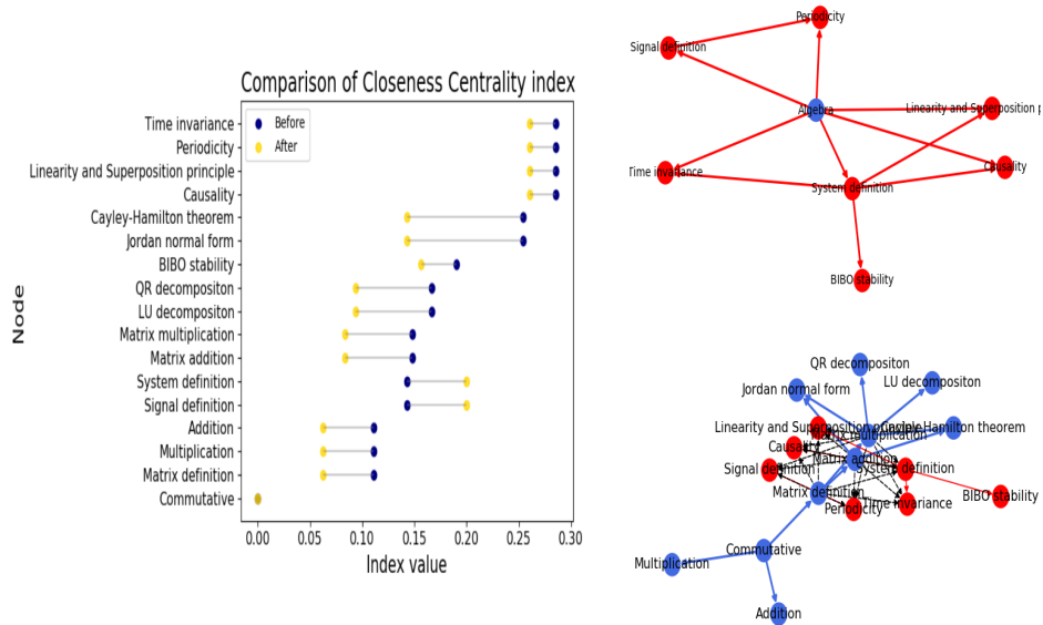
Figure 43: Closeness centrality calculated on the 'Systems Theory' learning graph before and after replacing super nodes, using the method that connect to the nodes with incoming and outgoing edges.
