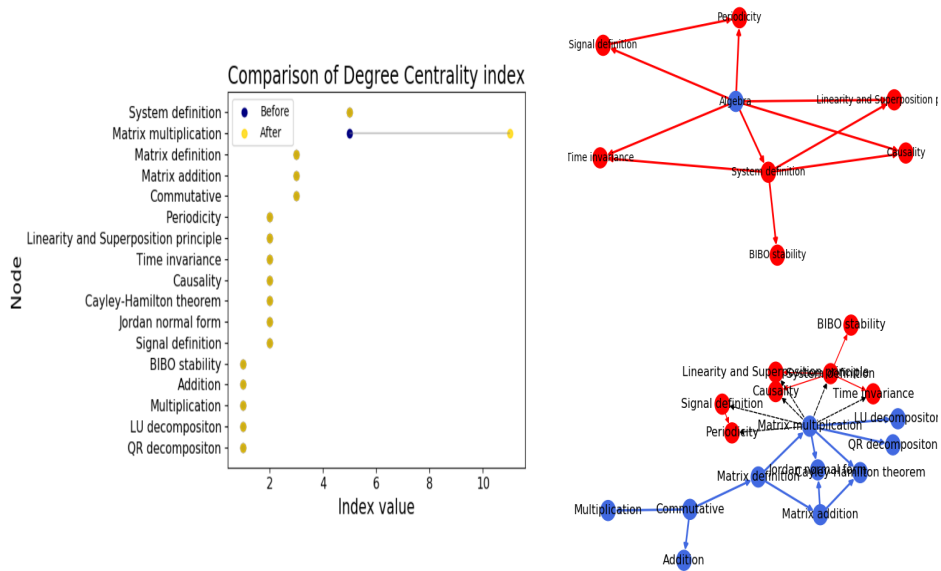
Figure 35: Degree centrality calculated on the 'Systems Theory' learning graph before and after replacing super nodes, using the method that connect to the nodes with the highest degree.
