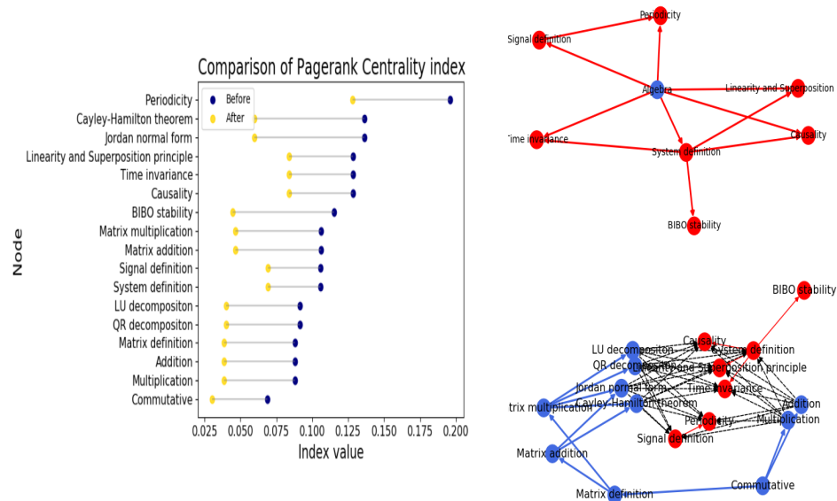
Figure 31: PageRank centrality calculated on the ‘Systems Theory’ learning graph before and after replacing super nodes, using the method that connect to nodes with no outgoing edges. The values are calculated using a damping factor of \alpha = 0.85 .
