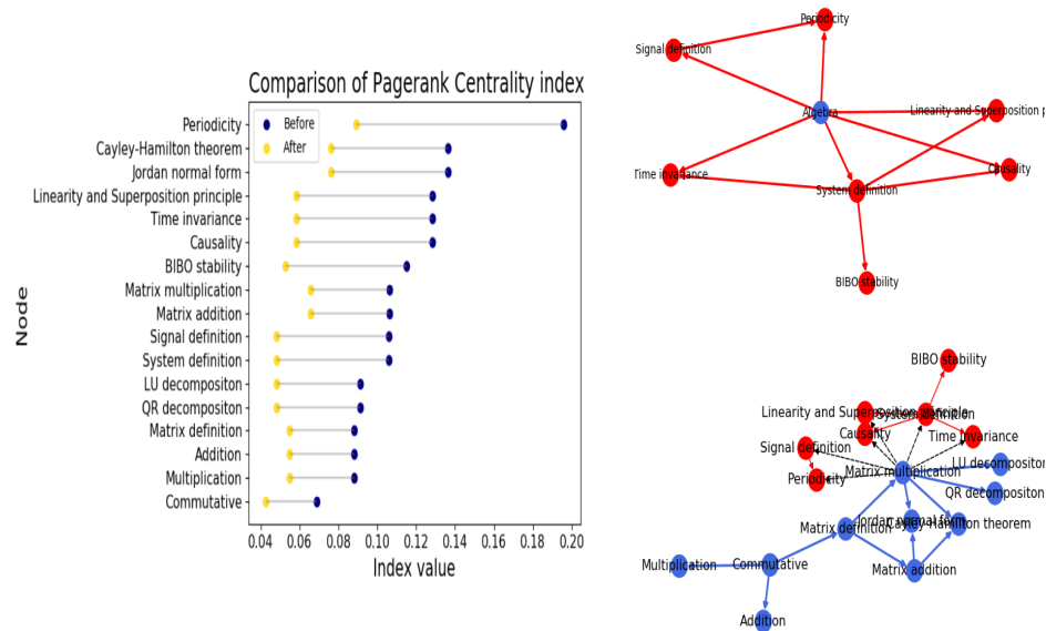
Figure 36: PageRank centrality calculated on the 'Systems Theory' learning graph before and after replacing super nodes, using the method that connect to the nodes with the highest degree. The values are calculated using a damping factor of \alpha = 0.85 .
