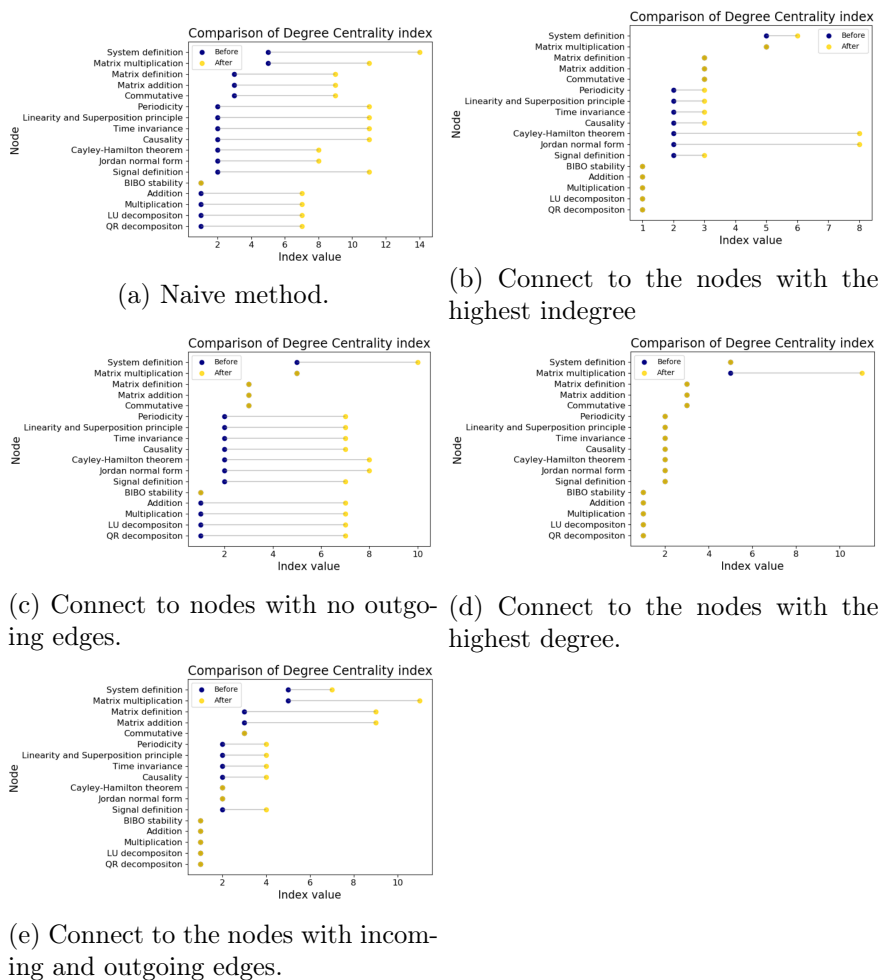
Figure 44: Degree centrality index comparison showing how the index changes for every method.
