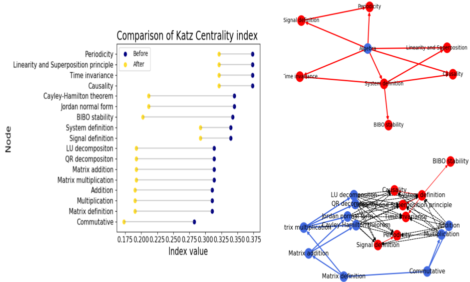
Figure 32: Katz centrality calculated on the 'Systems Theory' learning graph before and after replacing super nodes, using the method that connect to nodes with no outgoing edges. The values are calculated using a damping factor of \alpha = 0.1 and an initial centrality of \beta = 1.0 .
