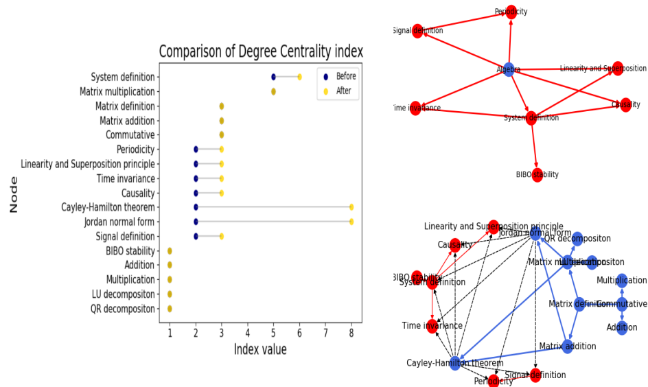
Figure 25: Degree centrality calculated on the 'Systems Theory' learning graph before and after replacing super nodes, using the method that connect to the nodes with the highest indegree.
