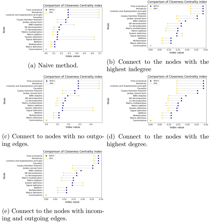
Figure 47: Closeness centrality index comparison showing how the index changes for every method.
