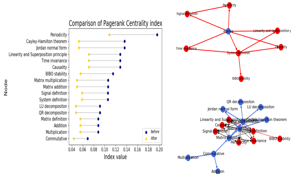
Figure 41: PageRank centrality calculated on the 'Systems Theory' learning graph before and after replacing super nodes, using the method that connect to the nodes with incoming and outgoing edges. The values are calculated using a damping factor of \alpha = 0.85 .
