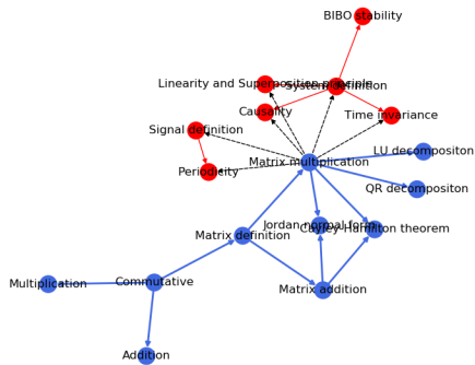
(e) Connect to the nodes with the highest degree.
