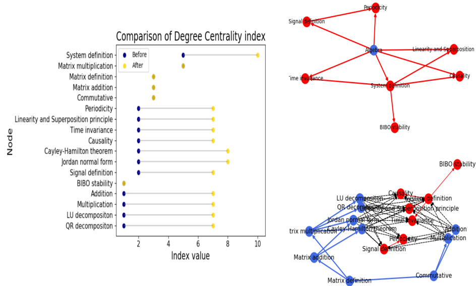
Figure 30: Degree centrality calculated on the 'Systems Theory' learning graph before and after replacing super nodes, using the method that connect to nodes with no outgoing edges.
