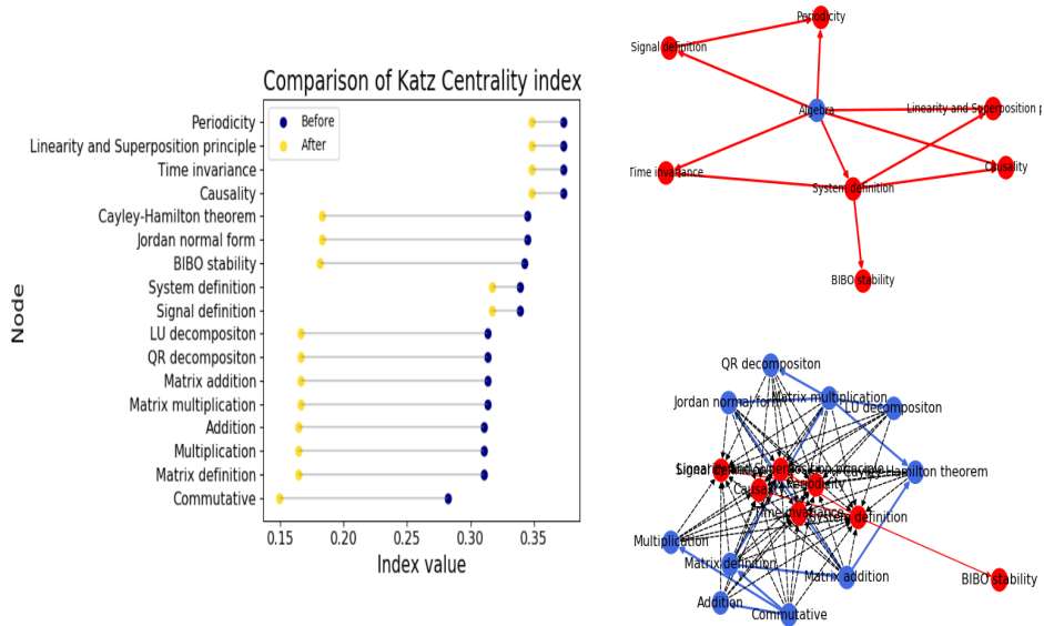
Figure 22: Katz centrality calculated on the ‘Systems Theory’ learning graph before and after replacing super nodes, using the naive method. The values are calculated using a damping factor of \alpha = 0.1 and an initial centrality of \beta = 1.0 .
