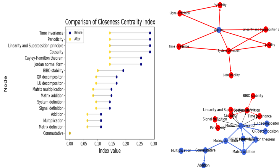
Figure 38: Closeness centrality calculated on the 'Systems Theory' learning graph before and after replacing super nodes, using the method that connect to the nodes with the highest degree.
