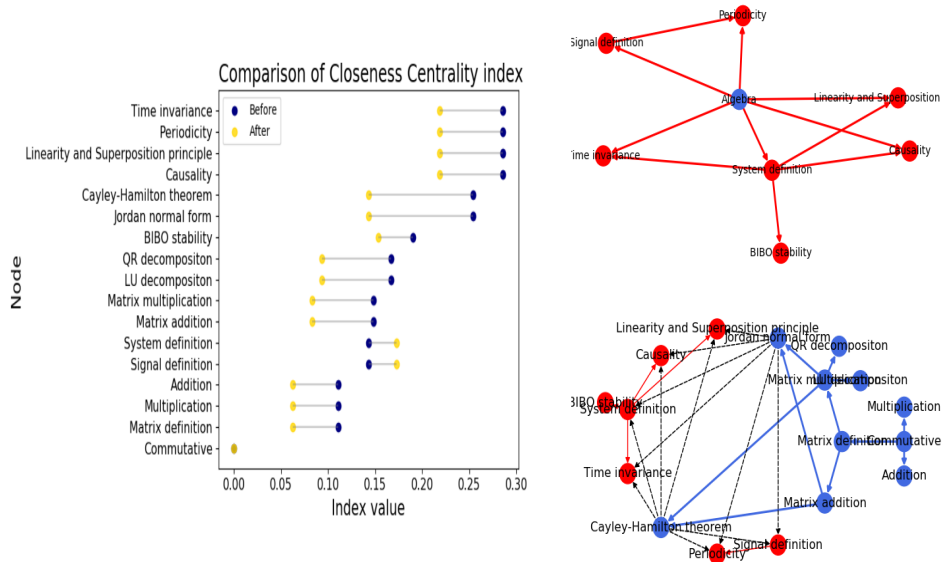
Figure 28: Closeness centrality calculated on the 'Systems Theory' learning graph before and after replacing super nodes, using the method that connect to the nodes with the highest indegree.
