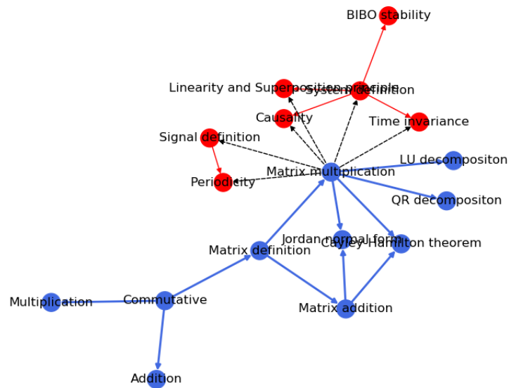
Figure 34: The merged graph for the Systems Theory course using the method that connect to the nodes with the highest degree.
