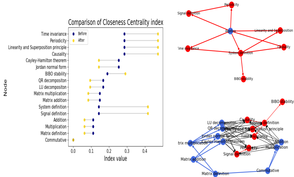
Figure 33: Closeness centrality calculated on the 'Systems Theory' learning graph before and after replacing super nodes, using the method that connect to nodes with no outgoing edges.
