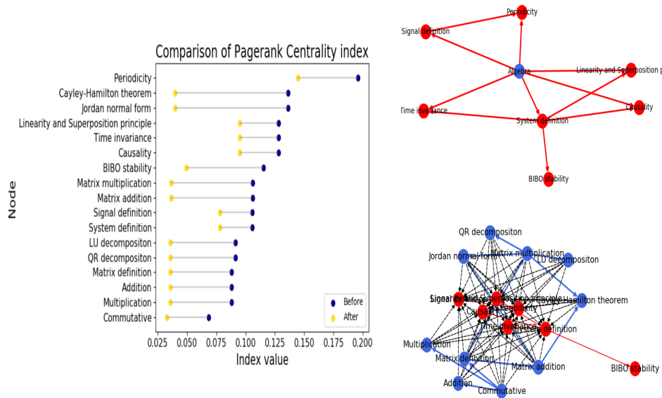
Figure 21: PageRank centrality calculated on the ‘Systems Theory’ learning graph before and after replacing super nodes, using the naive method. The values are calculated using a damping factor of \alpha = 0.85 .
