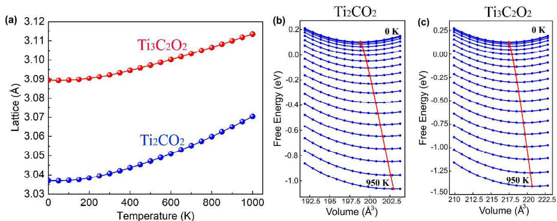
Figure 2. (a) Temperature-dependent a lattice parameters of \text{Ti}_2\text{CO}_2 and \text{Ti}_3\text{C}_2\text{O}_2 MXenes. Helmholtz energy of (b) \text{Ti}_2\text{CO}_2 and (c) \text{Ti}_3\text{C}_2\text{O}_2 MXenes as a function of volume at a temperature from 0 K to 950 K with 50 K steps are illustrated by filled blue circles, which are fit by the solid blue curves. The minimum energy of the curves is shown by the red symbols which determine the equilibrium volumes at each temperature. The red solid lines passing through the equilibrium volumes are guides to the eye.
