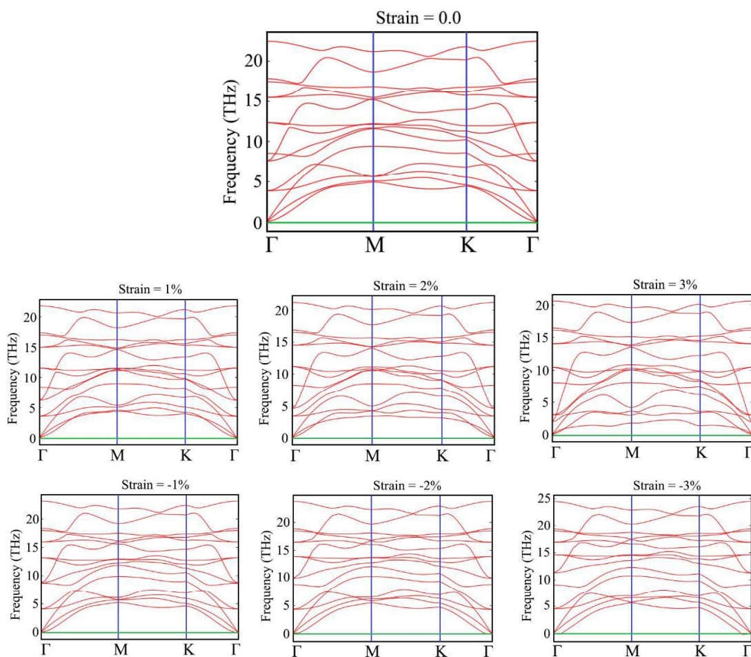
Figure S1. Phonon dispersion curves for \text{Ti}_2\text{CO}_2 at state-free state and biaxial tensile and compressive strain of 1%, 2%, and 3% in the basal plane.
