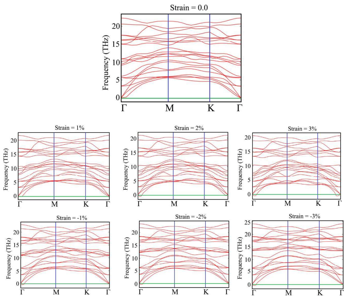
Figure S2. Phonon dispersion curves for \text{Ti}_3\text{C}_2\text{O}_2 at state-free state and biaxial tensile and compressive strain of 1%, 2%, and 3% in the basal plane.
