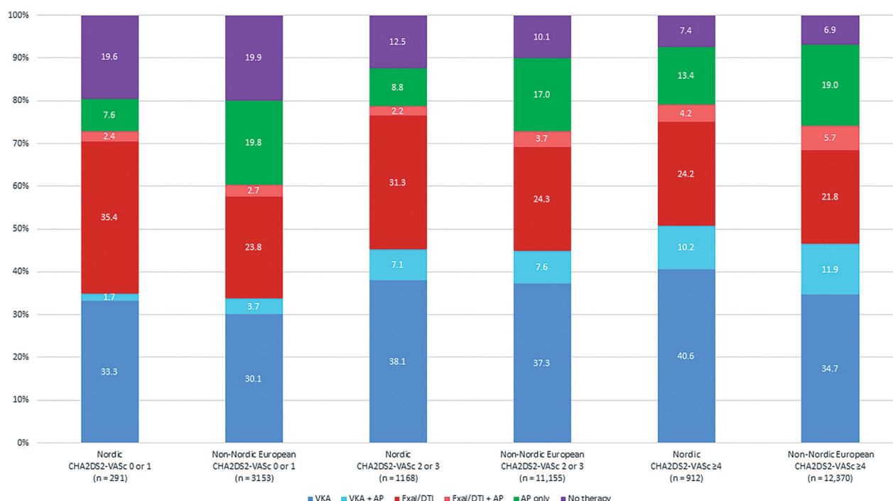
Figure 2. Antithrombotic treatment in CHA 2 DS 2 -VASc categories 0–1, 2–3, \geq 4 in Nordic and Non-Nordic European countries. AP: antiplatelet; DTI: direct thrombin inhibitors; FxaI: factor Xa inhibitors; VKA: vitamin K antagonists.
