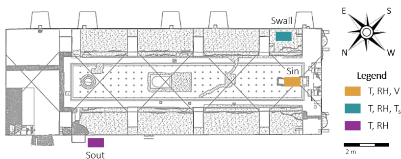
Figure 1. Position of the sensors in the Central Hall of the Mithraeum.
