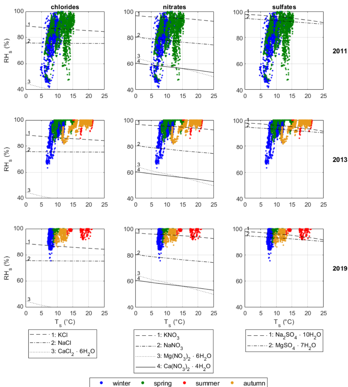
Figure 8. Relative humidity ( \text{RH}_s ) vs temperature ( T_s ) close to wall surfaces plotted on phase diagrams with the critical RH curve for deliquescence of chlorides, nitrates and sulfates. Chlorides: (1) sylvite (potassium chloride—KCl), (2) halite (sodium chloride—NaCl), (3) antarcticite (calcium chloride— \text{CaCl}_2 \cdot 6(\text{H}_2\text{O}) ). Nitrates: (1) nitre or nitrokalite (potassium nitrate— \text{KNO}_3 ), (2) nitratine (sodium nitrate— \text{NaNO}_3 ), (3) nitromagnesite (magnesium nitrate— \text{Mg}(\text{NO}_3)_2 \cdot 6(\text{H}_2\text{O}) ), (4) nitrocalcite (calcium nitrate— \text{Ca}(\text{NO}_3)_2 \cdot 4(\text{H}_2\text{O}) ). Sulfates: (1) mirabilite (sodium sulfate— \text{Na}_2\text{SO}_4 \cdot 10(\text{H}_2\text{O}) ), (2) epsomite (magnesium sulfate— \text{MgSO}_4 \cdot 7(\text{H}_2\text{O}) ).
