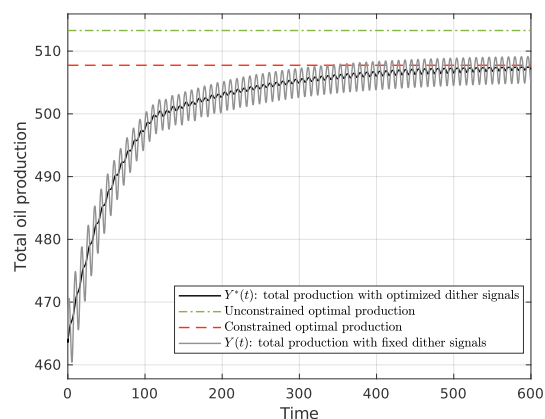
Fig. 7. Objective function.
