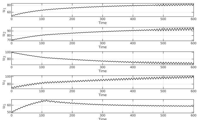
Fig. 4. Input signals.
