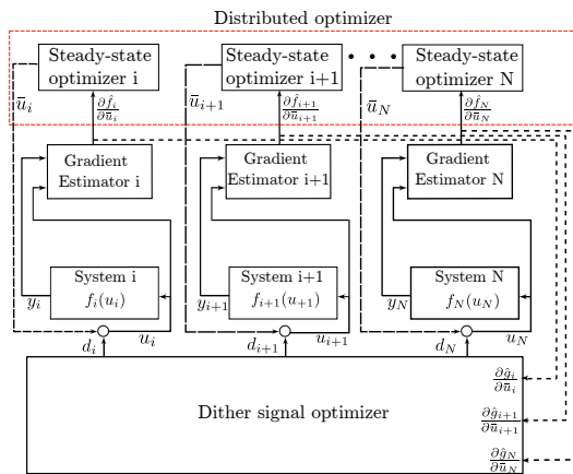
Fig. 1. Extremum-Seeking Scheme.
