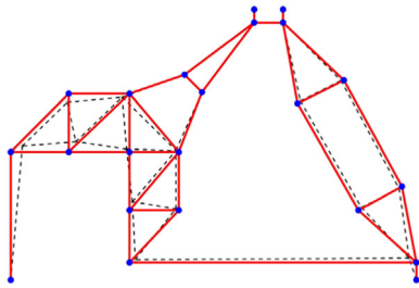
FIGURE 23 Truss-like structure of Result I-2. Dashed lines indicate the generated truss-like structures and solid lines show the adjusted structure
