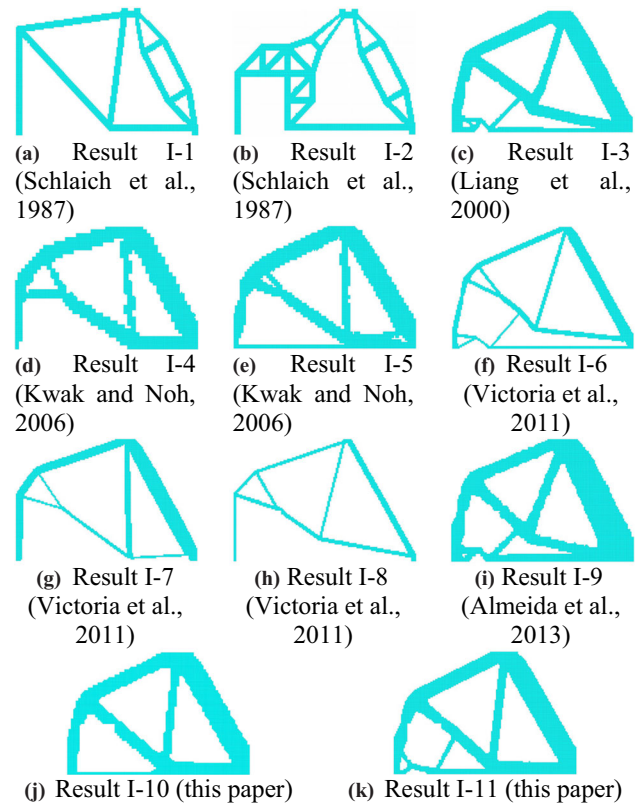
FIGURE 17 Case I: Topology optimized results of the deep beam with an opening
