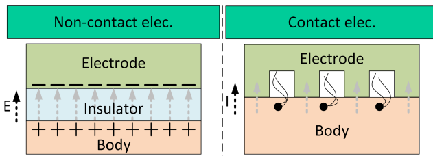
Fig. 2. Concept of contact and non-contact dry electrodes.
