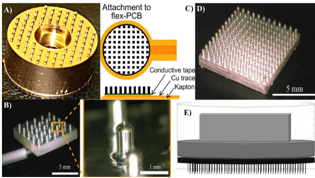
Fig. 8. Examples of invasive dry electrodes: A) micro-spike EEG electrode [79], B) candle-like dry micro-needle electrode [67], C) patterned vertical carbon nanotube electrode [73], D) newer version of candle-like dry micro-needle [67], and E) ENOBIO EEG electrode [49].
