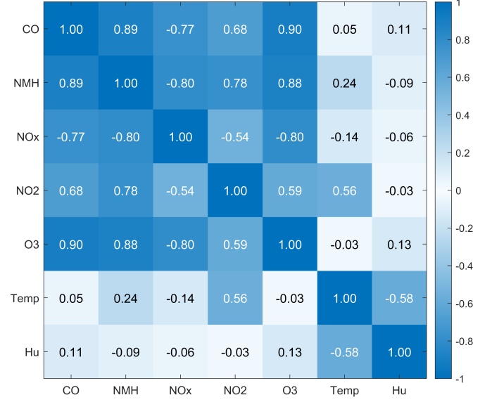
Fig. 2: correlation matrix of sensor pairs for AQ data-set.
