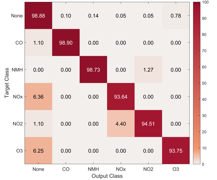
Fig. 4: Normalized confusion matrix for all classes during the test period. Numbers are in percent.
