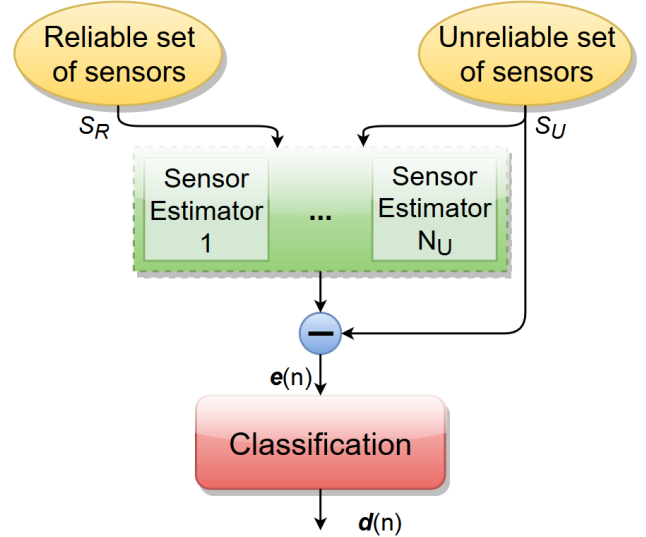
Fig. 1: The proposed system architecture for SFDIA.
