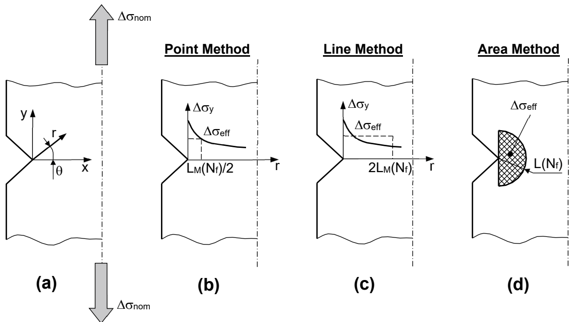
Fig. 1. Notched component subjected to fatigue loading (a); the TCD applied in the form of the Point (b), Line (c) and Area Method (d).
