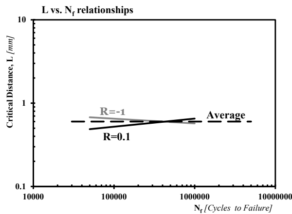
Fig. 3. Calibration of the L_M vs. N_f relationships for the AM titanium alloy under investigation.
