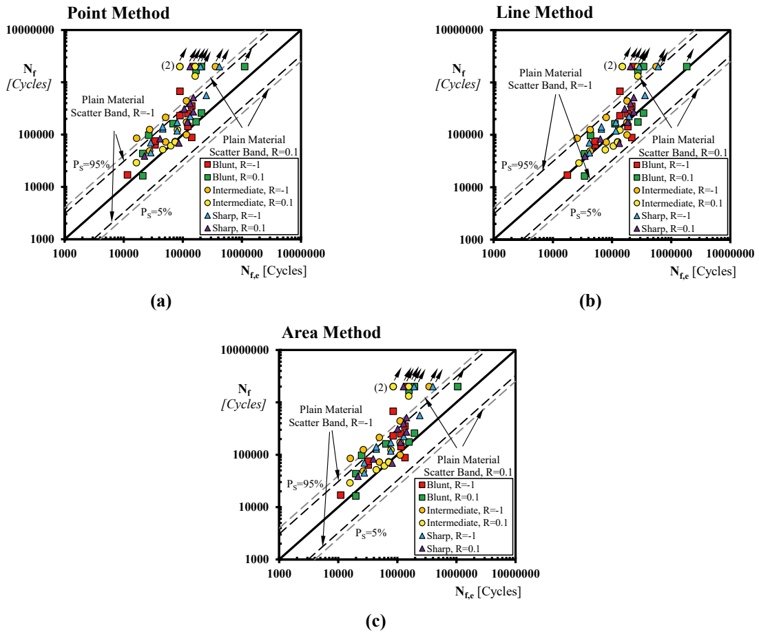
Fig. 4. Accuracy of the TCD in estimating the fatigue lifetime of the tested specimens of AM Ti6Al4V.
