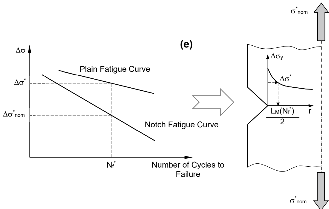
Fig. 2. Calibration of the L_M vs. N_f relationship by using two different fatigue curves.
