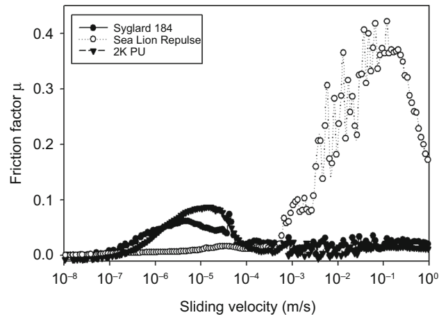
Fig. 7: Stribeck curves with sliding velocities from 10^{-8} m/s to 1 m/s as a comparison between Sylgard 184 (DFT = 122 \mu\text{m} ), Sea Lion Repulse (DFT = 81 \mu\text{m} ) and 2K PU (DFT = 50 \mu\text{m} ). T = -10^\circ\text{C} , F (normal) = 1 N
