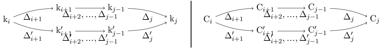
Figure 19: Keys and updated ciphertexts in Definition 11
