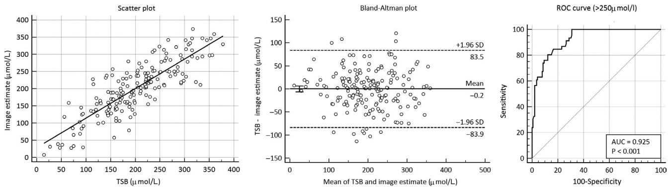
FIGURE 3 Scatter plot, Bland-Altman plot and ROC curve
