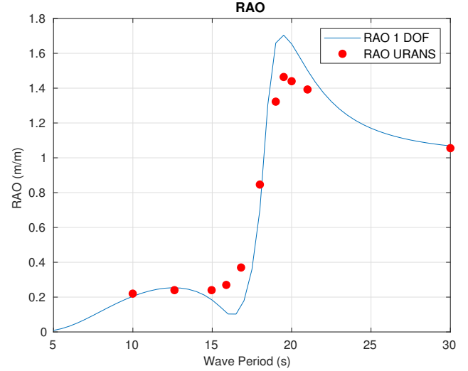
FIGURE 13: Comparison between RAO predictions performed with the decoupled heave differential equation (Eq. 12) and the URANS solver. Significant differences can be seen by comparison with URANS. Probably due to non-linear phenomena such as vortex-shedding and perturbation to the velocity and pressure fields due to platform motions
