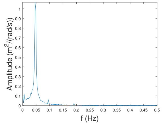
(b) Spectrum of surface elevation \xi(t) in amplitudes.
