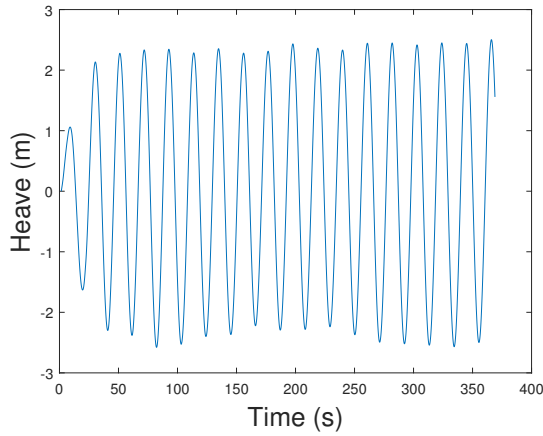
(c) Heave time history.
