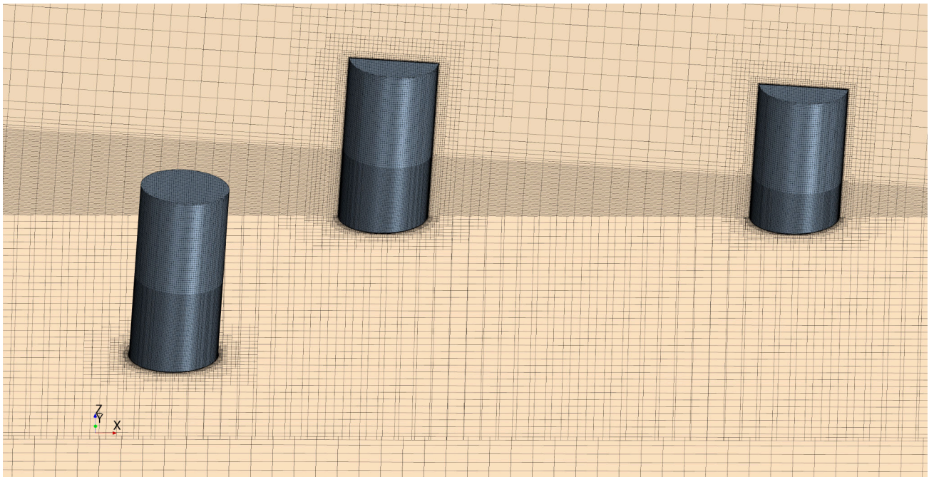
FIGURE 8: Example of a mesh near the platform at a time instant during the simulation. The overset domain is 1.5 \cdot L_p long, 1.5 \cdot B_p wide and 1.8 \cdot D_p deep. The platform is centered within the overset domain.
