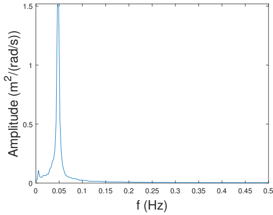
(a) Spectrum of heave motion H(t) in amplitudes.
