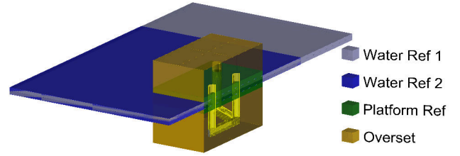
FIGURE 5: Representation of the mesh volume controls using a color code.
