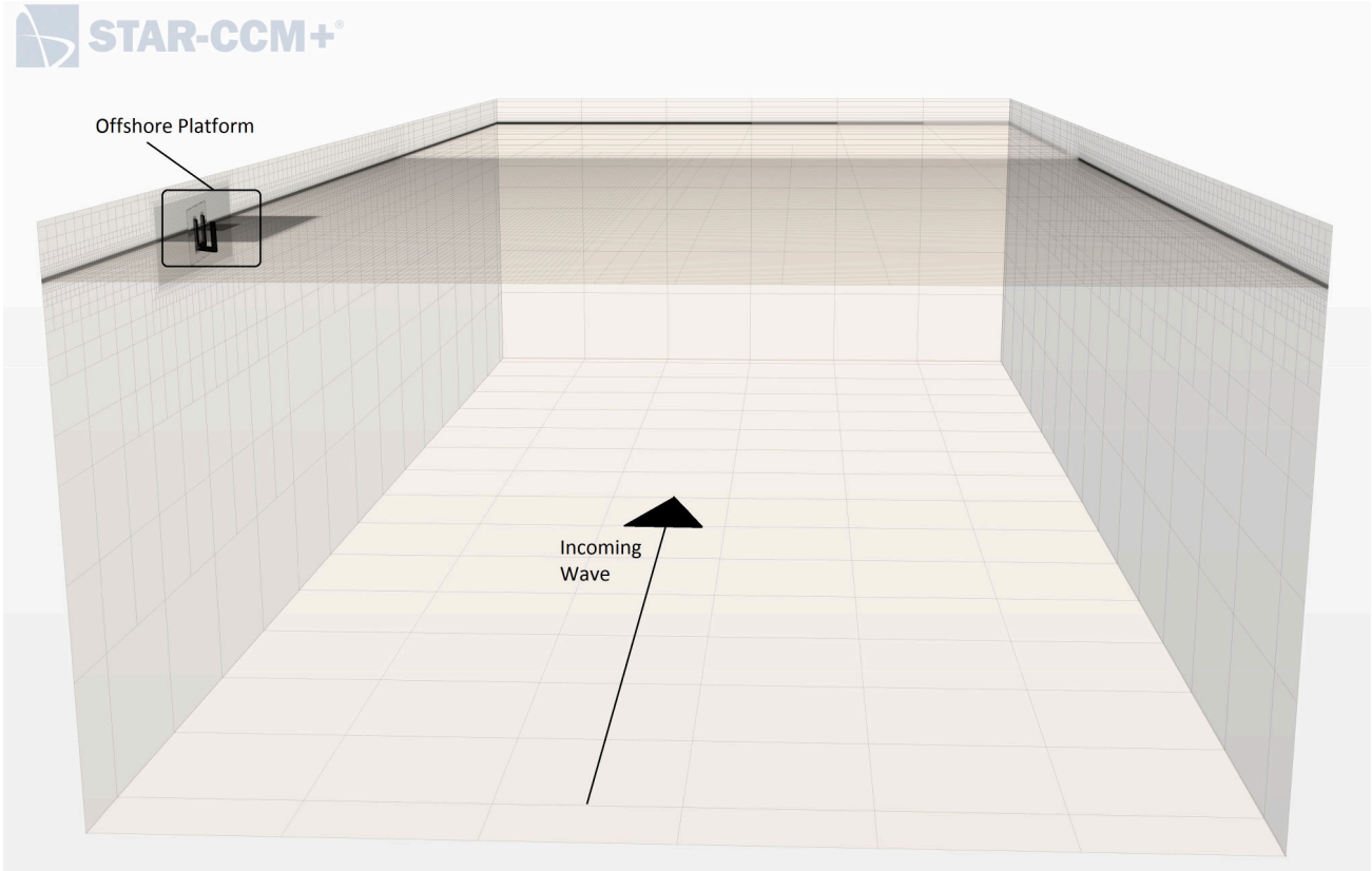
FIGURE 6: Example of the computational domain of the shortest wave ( T_w = 18s , A_w = 1.249m ). The mesh expands transversally, in the y -direction, starting approximately at the lateral mid-length and in the x -direction creating a numerical beach 2 \cdot \lambda_w long. Further mesh refinements are done near the platform, the results of these refinements can be seen in Fig. 7.
