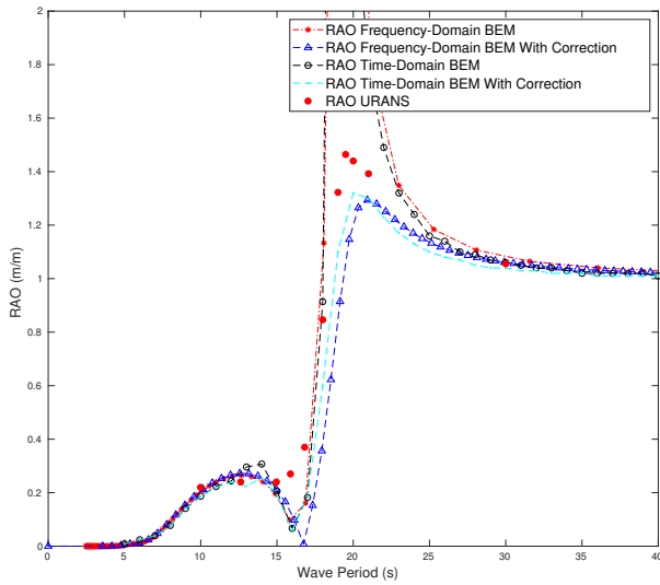
(a) Heave motion RAOs.
