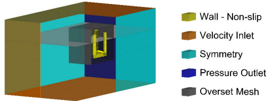
FIGURE 4: Representation of the boundary conditions using a color code. Relative dimensions between the floating body and the computational domain have been modified to allow for better visualization. (here and in Fig. 5).
