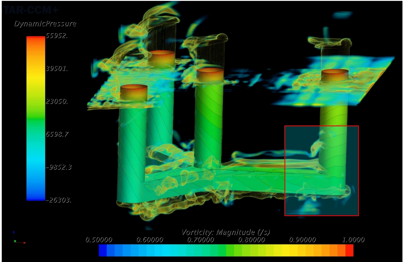
FIGURE 15: Vortex sheets being shedded at the platform edges. Flow confinement between the columns introduces perturbation to the vortex sheet development.
