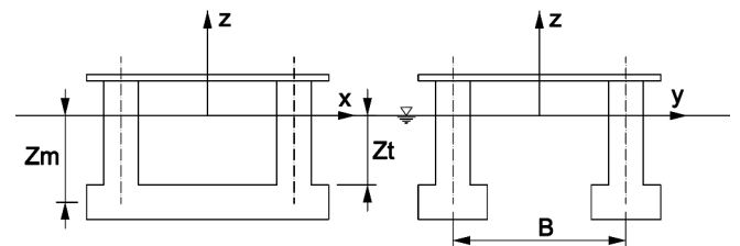
FIGURE 1: Sketch of a semisubmersible platform used in [2] to show how cancellation effects in heave motions occur.
