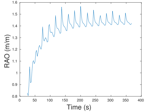
(d) RAO convergence with the increase of time simulated.
