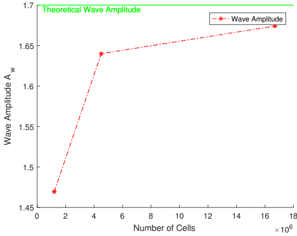
FIGURE 2: For the wave mesh convergence three levels of mesh resolution were used. The wave amplitude obtained through a FTT is plotted in the figure above and compared to the theoretical wave amplitude. The mesh used in the study is the second which has a 3.5% difference with the theoretical wave amplitude.
