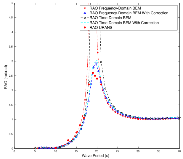
(b) Pitch motion RAOs.
