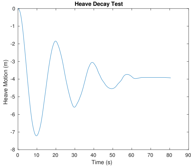
FIGURE 12: Evolution of the heave motions during the heave decay test performed in with the URANS solver. Drag coefficient estimated by comparison with experiments ( C_D = 3 ).
