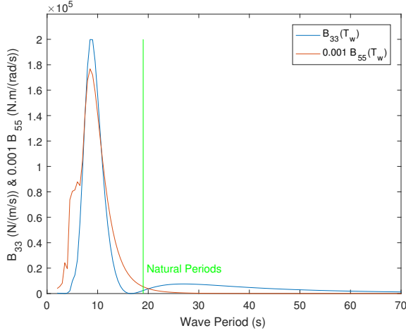
FIGURE 14: B_{33} and B_{55} radiation damping coefficients obtained from the frequency-domain BEM. A minimum near the natural period of oscillation generates unrealistically high motions (Fig. 10).
