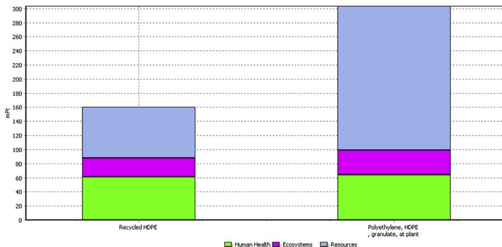
Fig. 11. Damage impacts associated to the use of 1 kg of recycled HDPE and 1 kg of virgin HDPE. Method ReciPe Endpoint.
