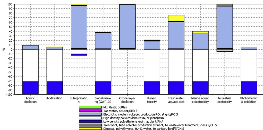
Fig. 10. Impact categories evaluated for the HDPE recycling process.
