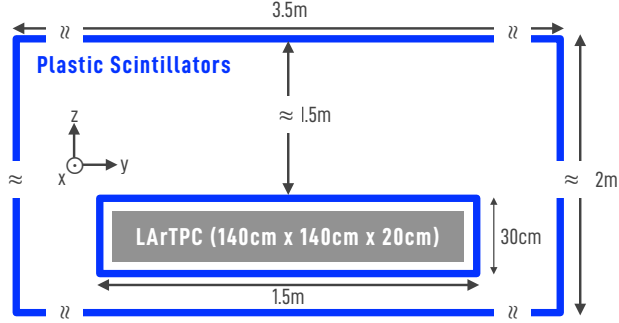
Figure 12: The GRAMS detector consists of a segmented liquid-argon time projection chamber surrounded by plastic scintillators. Reprinted with permission from [192].
