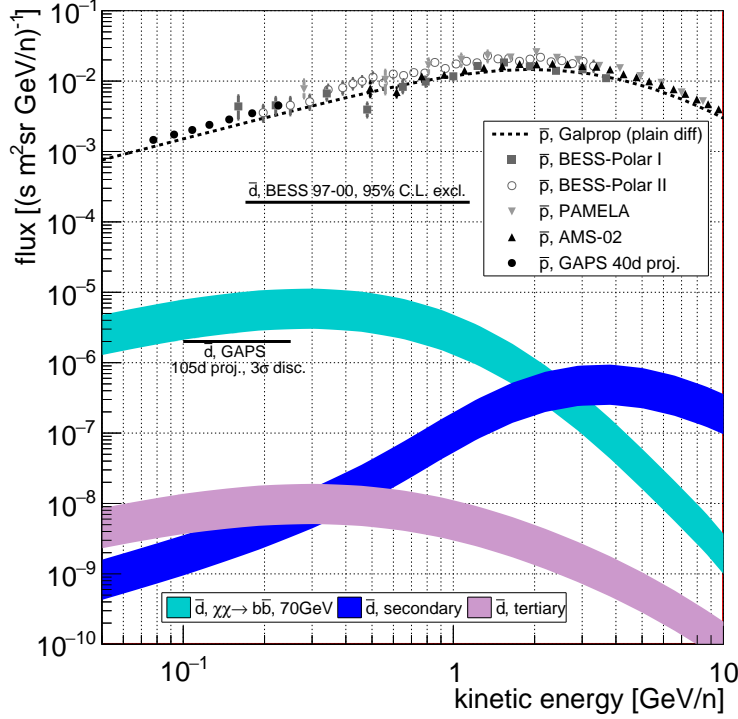
Figure 7: Antiproton flux data from AMS-02 [8], BESS-Polar I/II [4, 107], and PAMELA [6], as well as projections for the GAPS [91] antiproton flux measurements after 40 days, in comparison with the GALPROP plain diffusion prediction [108]. Also shown are the predicted antideuteron flux corresponding to DM parameters indicated by AMS-02 antiproton signal, interpreted as annihilation into purely b\bar{b} [38, 100]), as well as the predicted secondary and tertiary astrophysical antideuteron flux. The anticipated sensitivity of GAPS [57] for a 3\sigma discovery and the BESS 97–00 95% C.L. exclusion limits are indicated [54]. Solar modulation is treated in the force-field approximation with a potential of 500 MV. All antideuteron fluxes are derived in the analytic coalescence model with a coalescence momentum of 160 GeV [101] for the lower edge of the band and with a higher coalescence momentum of 248 GeV [102] for the upper edge of the band.
