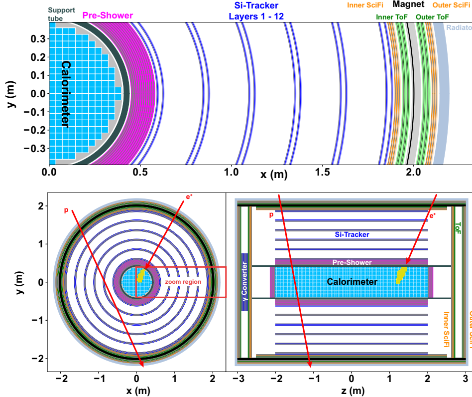
Figure 14: The AMS-100 instrument consists of a central calorimeter surrounded by a silicon-strip and scintillating-fiber tracker, all within a high-temperature superconducting solenoid magnet. Reprinted with permission from [204].
