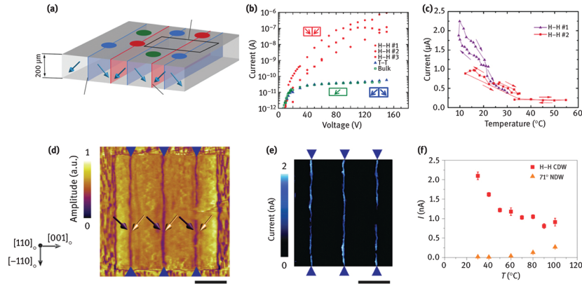
Figure 7: Conduction at created charged domain walls in ferroelectrics and multiferroics. (a) Sketch of the (110) \text{BaTiO}_3 crystal where the surface is covered with 200\ \mu\text{m} diameter electrodes. The domain walls are irregularly distributed with periods from 100 to 300\ \mu\text{m} . (b) Current-voltage characteristics of the tail-to-tail and head-to-head walls, as well as the domains. (c) Temperature dependence of the current through the head-to-head domain walls indicating a metallic behavior. ((a)–(c) are reprinted with permission from Springer Nature, taken from [104]. Copyright 2013 by Springer Nature.) (d) PFM amplitude of the domain pattern with alternating head-to-head and tail-to-tail domain walls defined by the trailing field of the SPM tip in La-doped \text{BiFeO}_3 thin films. (e) CAFM maps of the same domain pattern show an enhanced conduction at the head-to-head domain walls. The scale bars in (d) and (e) are 1\ \mu\text{m} . (f) Temperature dependence of the current through the head-to-head walls compared to that of native 71^\circ domain walls. ((d)–(f) are reprinted with permission from Springer Nature, taken from [114]. Copyright 2015 by Springer Nature.)
