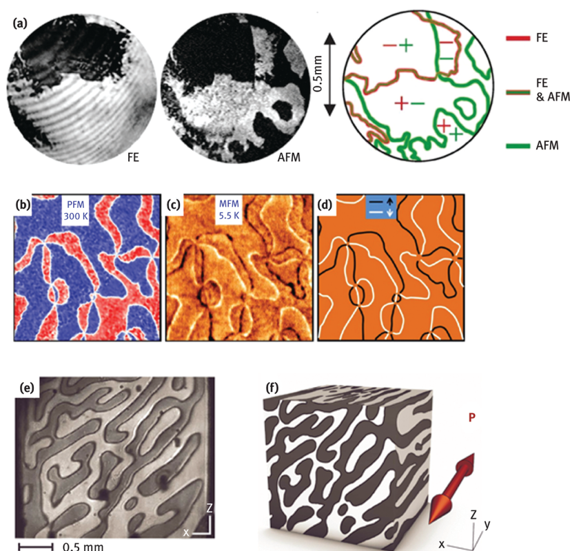
Figure 8: Electric and magnetic domains in multiferroics. (a) Coexistence of ferroelectric and antiferromagnetic domains in hexagonal \text{YMnO}_3 visualized by SHG. Bright and dark areas correspond to regions with different orientations of the order parameter ( P on the left image – ferroelectric (FE), L on the right image – antiferromagnetic (AFM)). The sketch on the right shows that some of the domain walls are both antiferromagnetic and ferroelectric. ((a) is reprinted with permission from Springer Nature, taken from [41]. Copyright 2002 by Springer Nature.) (b) PFM image of hexagonal \text{ErMnO}_3 showing up- and down-polarized ferroelectric domains. (c) MFM image at low temperature at the same location as in (b) showing an induced magnetic moment at ferroelectric domain walls. (d) Sketch from image in (c), emphasizing the magnetic moments at domain walls of the 16 \times 16 \mu\text{m}^2 image. ((b)–(d) reprinted (adapted) with permission from [140]. Copyright 2012 American Chemical Society.) (e) Multiferroic domain walls in the spin-spiral system \text{MnWO}_4 visualized by SHG. (f) Illustration showing the 3D distribution of the multiferroic domains in (e). ((e)–(f) reprinted with permission from [37]. Copyright 2009 by the American Physical Society.)
