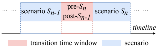
Fig. 6. Transition time windows on the timeline.
