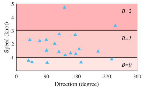
Fig. 3. Wind speed and direction in statistics.
