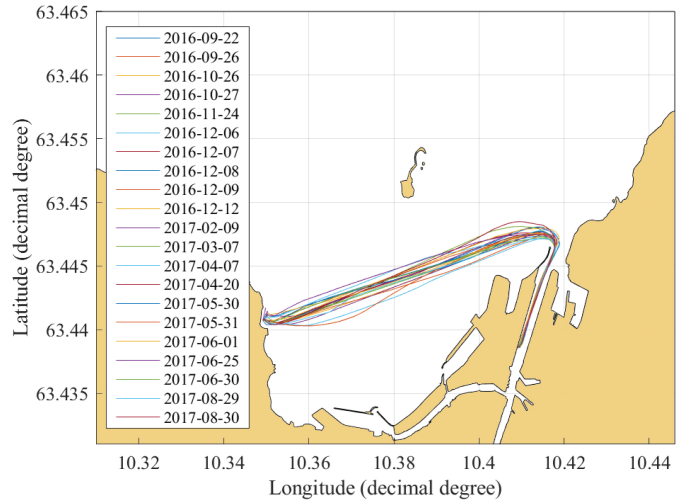
Fig. 2. Collection of 21 commuter sailings.
