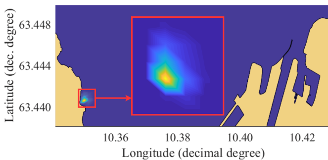
Fig. 9. Heat map presenting the likelihood site of the departing scenario.
