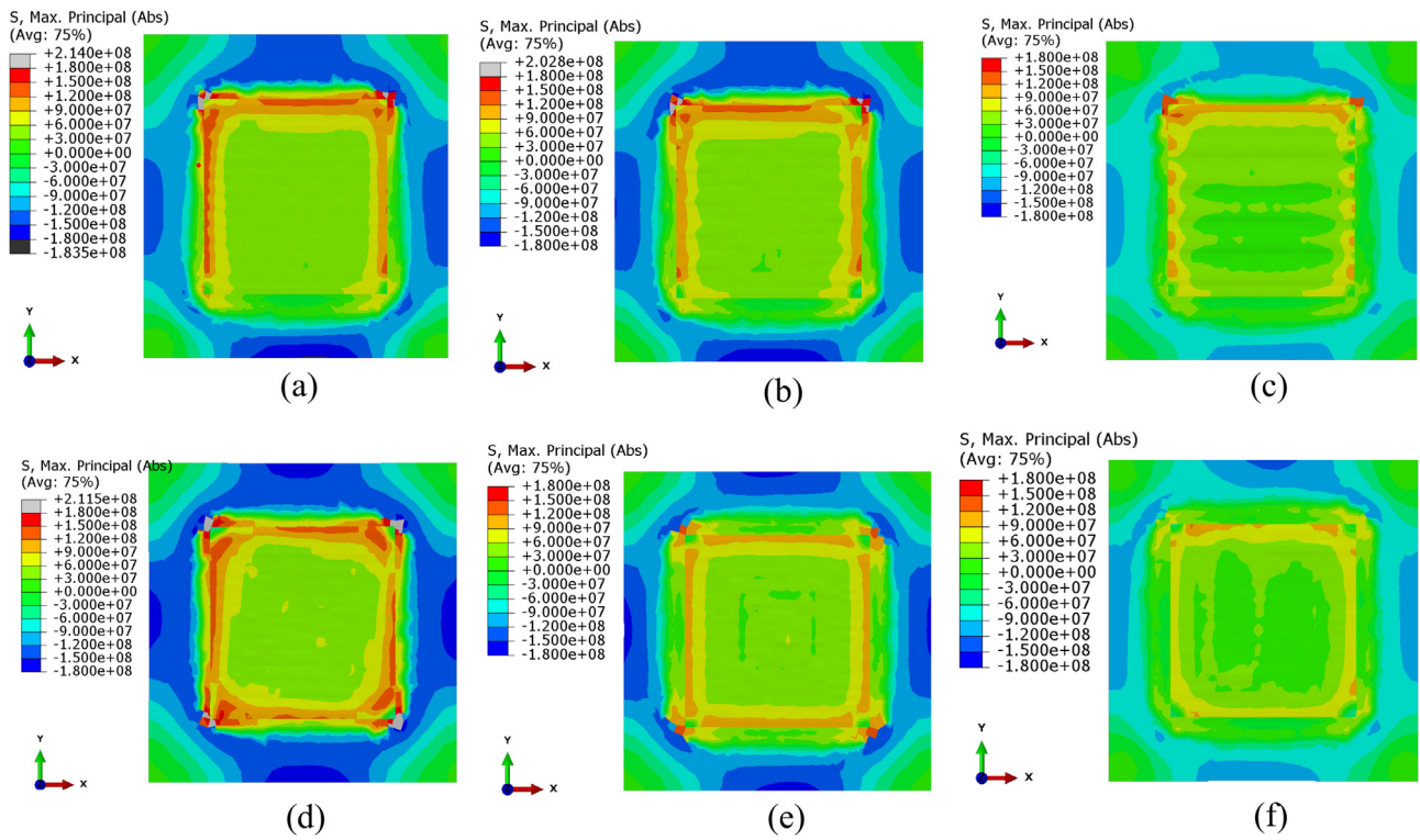
Fig. 8. Maximum principal residual stress distribution of different deposition patterns, (top view, unit: Pa), (a) Zig-zag; (b) Raster; (c) Alternate-line; (d) Out-in spiral; (e) In-out spiral; (f) S.
