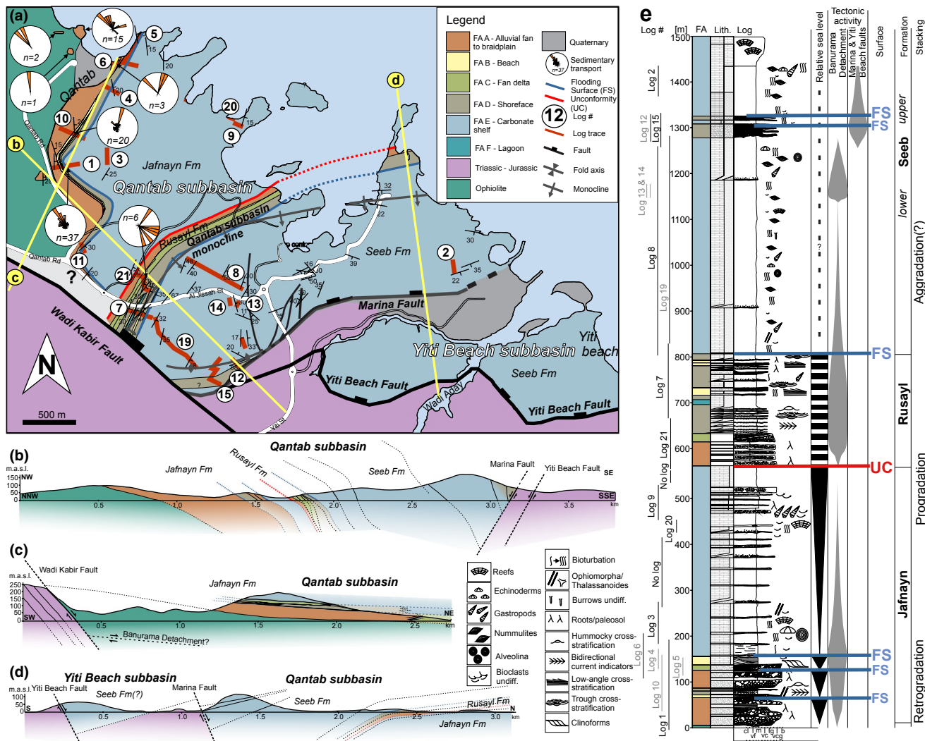
FIGURE 3 (a) Mapped facies associations in the Bandar Jissah Basin with structural measurements, log traces reported in Figure 5 and paleocurrent measurements. Main structural elements annotated. Location shown in Figure 2b. Modified after Le Métour et al. (1992). (b, c and d) show cross-sections with key structural and stratigraphic features. Profile locations in (a). (e) Displays a composite log through the Bandar Jissah Basin succession
