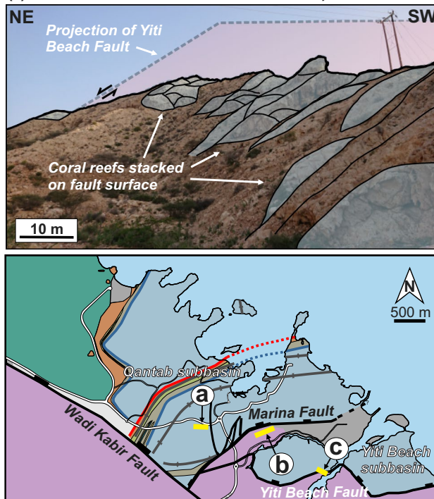
FIGURE 9 Seeb Formation carbonate growth sections in the Qantab subbasin. (a) Lower Seeb Formation growth package in Qantab subbasin monocline with supporting logs and proposed model. (b) Upper Seeb Formation growth packages as seen along strike in the immediate hanging wall of the Marina fault. Strata expand towards inferred local displacement maximum. (c) Coral reefs stacking on Yiti Beach Fault
