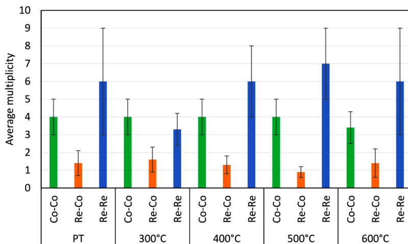
Fig. 8. Average coordination numbers ( N ) from EXAFS analysis for \text{CoRe}_{1.6} after 60 min pre-treatment at 600 °C in \text{H}_2/\text{Ar} (left), and during heating in 5% \text{NH}_3 for Co \text{K} -edge and \text{Re L}_{\text{III}} -edge at selected temperatures.
