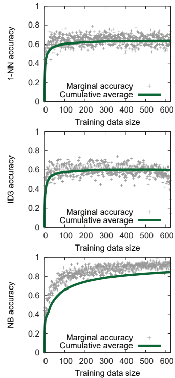
Fig. 6 Average marginal and cumulative accuracy for the Balance Scale data set. The data points show the average marginal accuracy for each incremental problem solving attempt, while the solid curves shows the cumulative average accuracy over the entire data set up to that point
