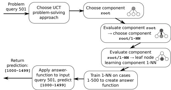
Fig. 5 Example system flow. This shows the process the system goes through to solve a single problem query. The nodes in the tree correspond to components that are recursively evaluated, until a leaf node is reached which in turn produces a prediction for the given problem query
