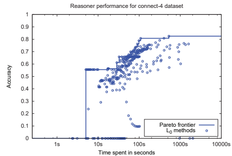
Fig. 3 Example reasoner performance differences (using the methods from 4.4). The points in the centers of the circles represent different L_0 reasoning methods and show their accuracy vs. time performance records. The Pareto frontier of possible optimal choices representing different accuracy/time trade-offs is shown as a solid line.
