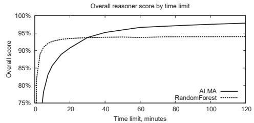
Fig. 9 Overall reasoning performance across all data sets, comparing ALMA and the best individual reasoning method RandomForest. Given sufficient time, ALMA considerably outperforms RandomForest and the other individual reasoning methods
