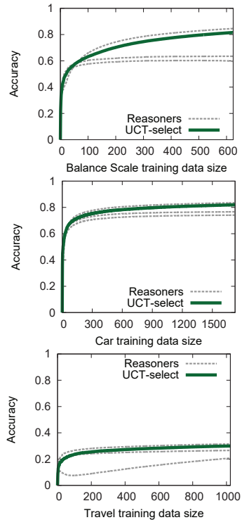
Fig. 8 Aggregate system behavior for 3 different data sets. The thin dashed lines in the graphs represent the performance of individual reasoning methods (1-NN, ID3, Naive Bayes) while the thick line is UCT-select’s performance using those three methods
