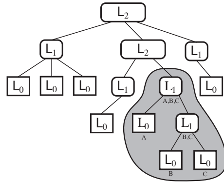
Fig. 1 Snapshot of a (tiny) ALMA component hierarchy. The L_0 boxes represent non-learning instances of fully trained classifier functions, e.g. decision trees and neural networks. A single ALMA system typically contains a heterogeneous variety of such classifier instances. L_1 boxes represent methods that learn from training data, and L_2 boxes represent the metareasoning components that ALMA is focused on. The shaded subtree illustrates score aggregation, where the L_1 component marked "A,B,C" is scored based on the combined scores of the L_0 components marked "A", "B", and "C"
