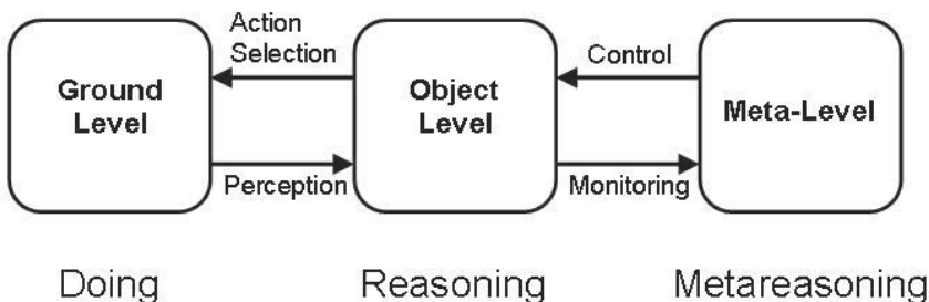
Figure 2.2: Duality in reasoning and acting [15], a high-level framework for describing metareasoning processes.
