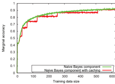
Fig. 4 The performance of an underlying learning component and the effect of adding caching. The graph shows marginal accuracy, which clearly displays the step-wise behavior of the caching component.
