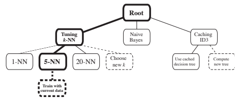
Fig. 2 Example problem-solving flow. For each new query, components are recursively evaluated from the root node until arriving at a leaf node. The leaf node component is used to predict the output solution for the query. In this example the Tuning k -NN sub-tree is first selected, then 5-NN, a new L_0 component is trained using 5-NN, and this new component is used to answer the problem query. (Previously trained L_0 components are not shown in this figure)
