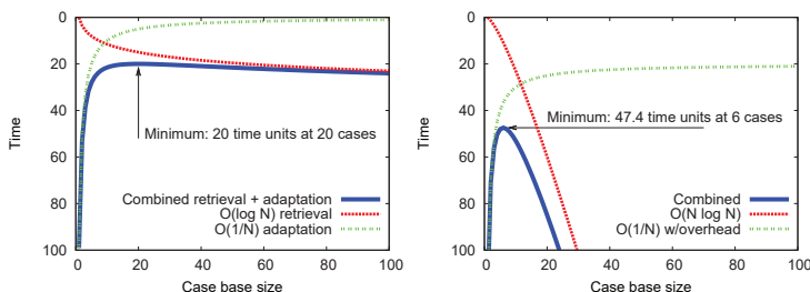
Fig. 2. Retrieval, adaptation and combined solution time compared to case base size for two other speed-up learner scenarios: On the left, using an O(\log N) retrieval algorithm and a O(1/N) adaptation algorithm. On the right, using an O(N \log N) retrieval algorithm and a O(1/N) adaptation algorithm with overhead.
