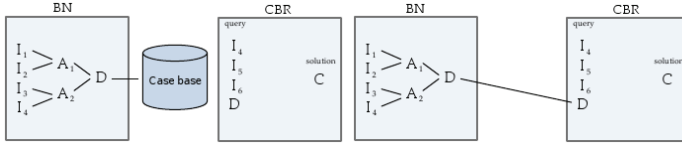
Figure 3. BN-CBR-1 Architecture
