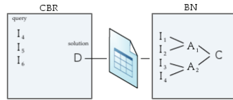
Figure 6. CBR-BN-2 Architecture
