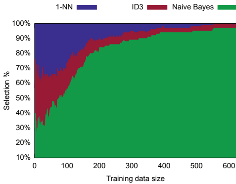
Fig. 7 UCT-select behavior for the Balance Scale data set. The graph shows the average fraction of queries where each of 1-NN, ID3, and Naive Bayes are chosen for the Nth problem query. Naive Bayes performs the best on this data set, and the system correctly learns to prioritize using Naive Bayes higher than the other methods
