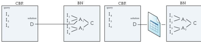
Figure 5. CBR-BN-1 Architecture
