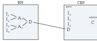
Figure 4. BN-CBR-2 Architecture
